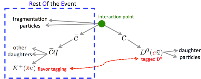
Fig. 2. The sketches of the ROE method. The events with only one K^\pm in the ROE are selected; the flavour of the neutral D meson is determined by the charge of the kaon.
