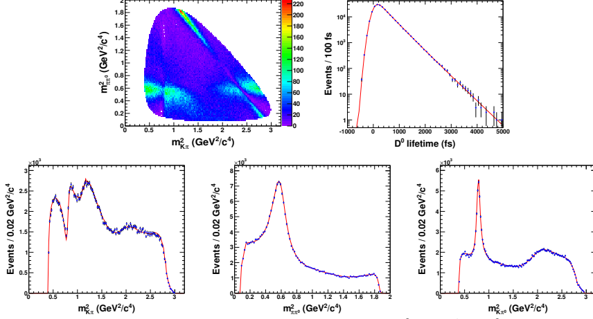
Fig. 1. Time-dependent fit to the Dalitz plot of wrong-sign D^0 \rightarrow K^+ \pi^- \pi^0 decays. The decay times are smeared by the expected Belle II decay-time resolution of 140 fs. The second row shows projections of the fitted Dalitz variables m_{K^+ \pi^-}^2 (left), m_{\pi^- \pi^0}^2 (middle), and m_{K^+ \pi^0}^2 (right).
