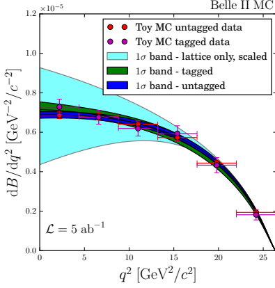
Figure 6: An example of a Belle II simultaneous fit to MC data and LQCD input at 5 \text{ ab}^{-1} including LQCD forecasts in 5 years for the tagged and untagged analysis.
