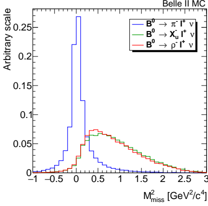
Figure 2: The M_{miss}^2 = p_{miss}^2 distribution of tagged B^0 \rightarrow \pi^- \ell^+ \nu_\ell candidates. The signal is expected to be located in a narrow peak near zero, while background from other b \rightarrow u transitions populates a wider region towards higher missing mass, due to missing particles.
