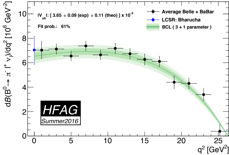
Figure 1: Extraction of |V_{ub}| from the B \rightarrow \pi \ell \nu mode with a simultaneous fit to averaged Belle and BABAR data, LCSR point and LQCD form-factor parameters, using a model independent parametrization of the form-factors.
