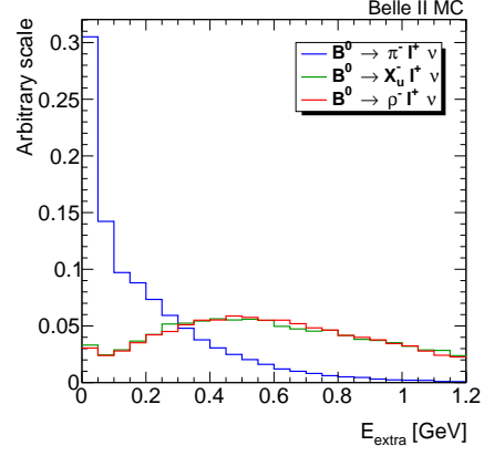
Figure 3: The E_{extra} distribution of tagged B^0 \rightarrow \pi^- \ell^+ \nu_\ell candidates. In correctly reconstructed signal events there is little energy deposited in the calorimeter that can not be associated neither to the decay products of the signal nor to the companion B meson.
