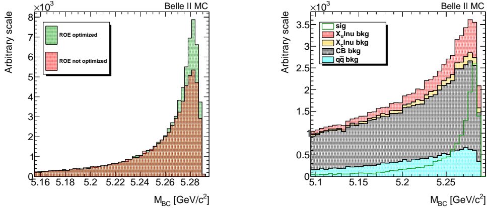
Figure 5: The M_{BC} distribution of signal B \rightarrow \pi \ell \nu candidates before and after rest of event (ROE) clean-up (left). M_{BC} is a variable which constrains the B meson to the CMS energy of the initial beam, while obtaining the reconstructed momentum of the particle. Signal candidates peak at nominal B meson mass with a narrow width, while the peak-like distribution of background candidates is not as prominent (right).
