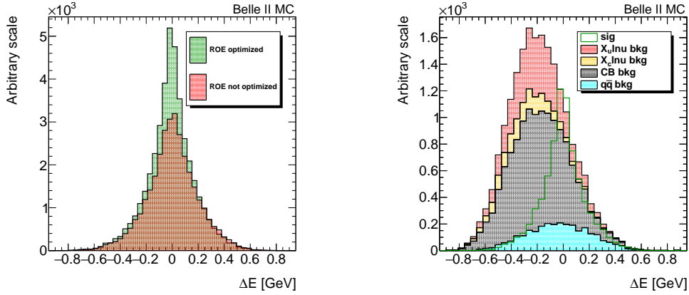
Figure 4: The \Delta E distribution of signal B \rightarrow \pi \ell \nu candidates before and after rest of event (ROE) clean-up (left). \Delta E is a variable which compares the B meson energy to the CMS energy of the initial beam. Signal candidates peak at zero, while background (except continuum) candidates are shifted to the negative values due to an incomplete reconstruction (right).
