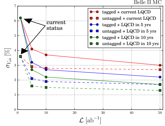
Figure 7: |V_{ub}| precision estimates for the tagged and untagged reconstruction method at 5, 10 and 50 \text{ ab}^{-1} of integrated luminosity for current LQCD and LQCD forecasts in 5 and 10 years.
