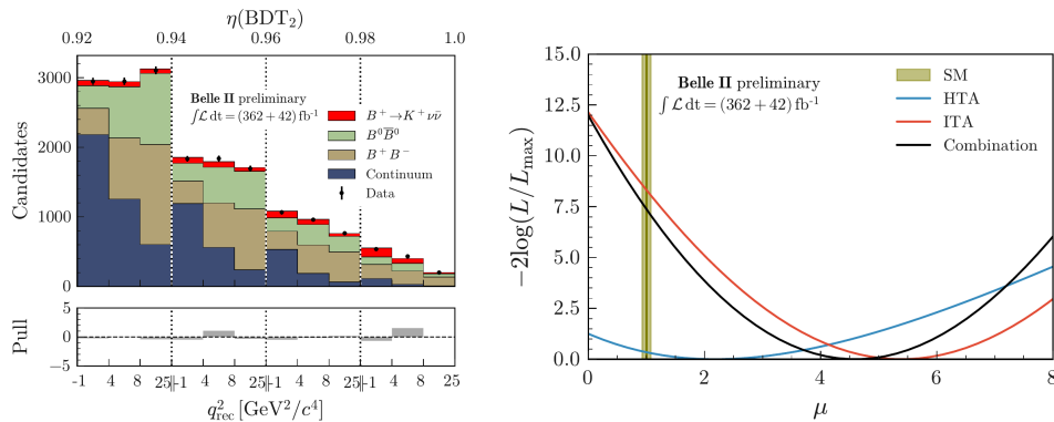
Fig. 3. Left figure: distribution of the output of the multivariate classifier utilized for signal discrimination in the ITA analysis (the signal component is in red). Right: profile log-likelihoods of the signal strength \mu for the HTA analysis (blue curve), ITA (red) and their combination (black).
