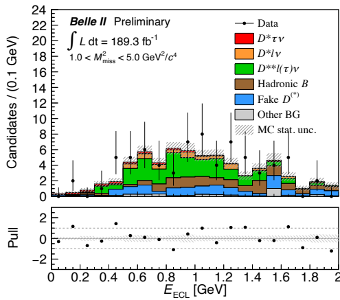
Figure 1. Comparison of the E_{\text{ECL}} distribution between data and simulation in the \bar{B} \rightarrow D^0 \ell^- \bar{\nu}_\ell sideband region, where 1.0 < M_{\text{miss}}^2 < 5.0 \text{ GeV}^2/c^4 is applied. The bottom panel shows the difference between data and simulation divided by the uncertainty in the data (pull).
