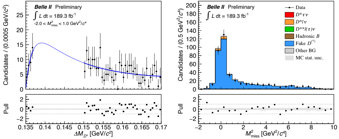
Figure 2. Left: the distribution of M_D (black points) in the sideband for D^0 \rightarrow D^0 \pi^0 at M_{\text{miss}}^2 \in [2.0; 1.0] \text{ GeV}^2/c^4 with \tau results overlaid (blue line). Right: the distribution of M_{\text{miss}}^2 in the M_D region for data (black points) and simulation (histogram) after the calibration of the fake D yields. The bottom panels show pull values from \tau results or simulation.
