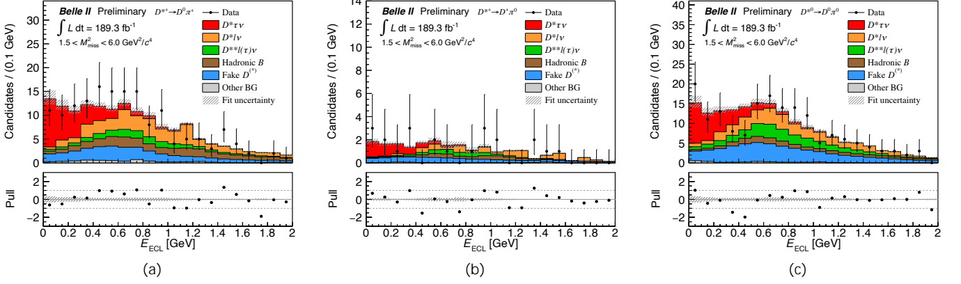
Figure 6. Distributions of E_{\text{ECL}} in the signal-enhanced region 1.5 < M_{\text{miss}}^2 < 6.0 \text{ GeV}^2=c^4 for the D^+ ! D^0 + (left), D^+ ! D^+ 0 (middle), and D^0 ! D^0 0 (right) modes, with t projections overlaid. The bottom panel presents pull values from t results. The rectangular-shaded regions on the histograms and in the pull plot correspond to statistical uncertainties in the t .
