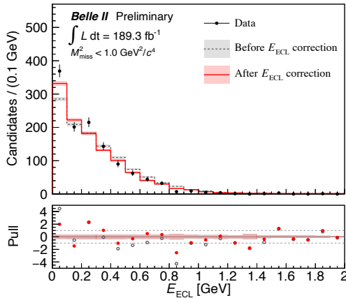
Figure 3. Comparison between data and simulation of the E_{\text{ECL}} distributions for D^+ \rightarrow D^0 \pi^+ at M_{\text{miss}}^2 < 1.0 \text{ GeV}^2/c^4 . The black points with error bars are the data. The red solid (gray dashed) histogram is from the simulation after (before) the E_{\text{ECL}} correction where the nominal energy shift at 15 MeV is applied. The bottom panel presents pull values before (gray open circles) and after the correction (red closed circles). The rectangular-shaded regions on the histograms and in the pull plot correspond to statistical uncertainties of the simulation.
