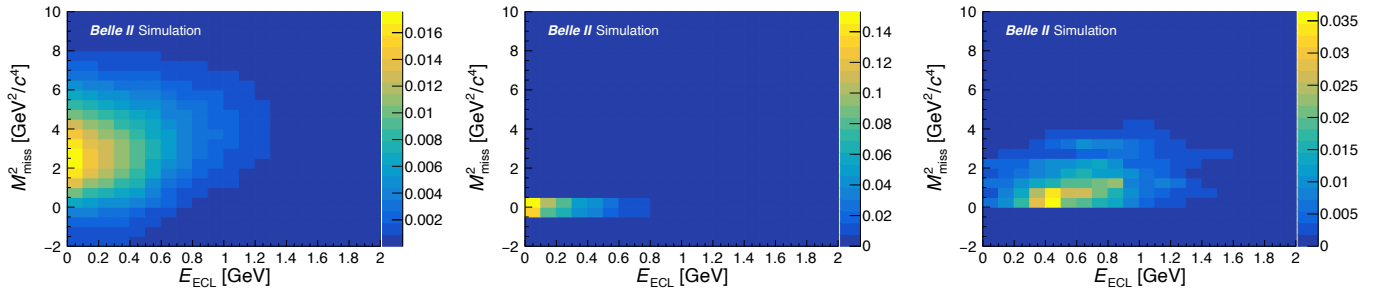
Figure 4. Two-dimensional PDFs of E_{\text{ECL}} and M_{\text{miss}}^2 from \bar{B} \rightarrow D^+ \tau^- \nu (left), \bar{B} \rightarrow D^0 \ell^- \bar{\nu}_\ell (middle), and \bar{B} \rightarrow D^+ \ell^- \bar{\nu}_\ell (right) in the D^+ \pi^0 mode. The normalization of the intensity scale is arbitrary.
