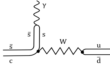
Figure 1: Feynman diagram
