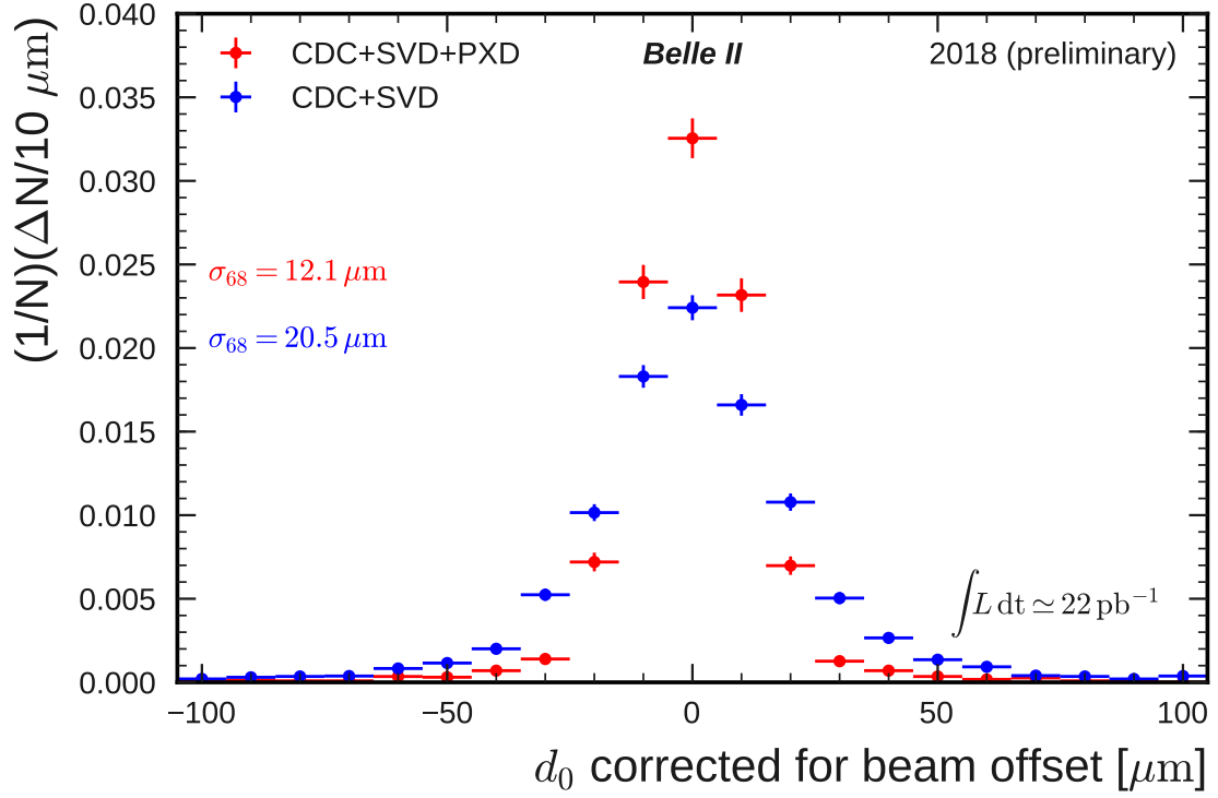
FIG. 1: d_0 distributions of selected tracks reconstructed with the default reconstruction chain (CDC+SVD+PXD) and the chain excluding the PXD detector (CDC+SVD). The resolution is estimated using half of the symmetric range around the median containing 68% of the d_0 distribution. The distributions are normalised to unit area.
