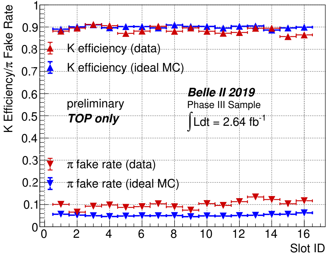
FIG. 6: Kaon efficiency and pion fake rate for the TOP only PID criterion \mathcal{R}_{K/\pi} > 0.5 using the decay D^{*+} \rightarrow D^0[K^-\pi^+]\pi^+ in the 16 TOP slots.
