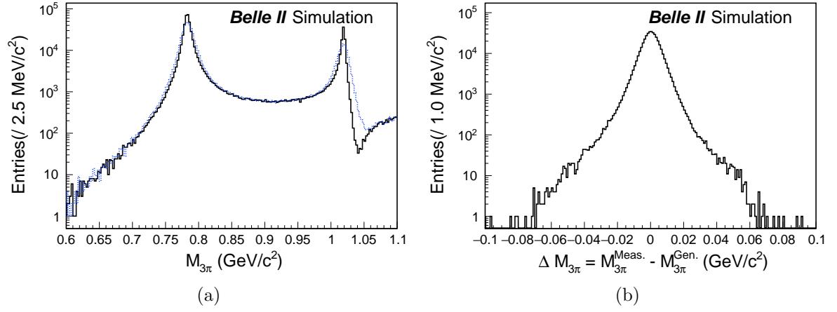
FIG. 11: (a) M(\pi^+\pi^-\pi^0) spectrum of generated (solid) and measured values (dashed) of e^+e^- \rightarrow \pi^+\pi^-\pi^0\gamma MC. (b) Difference of measured and generated values of M(3\pi) .
