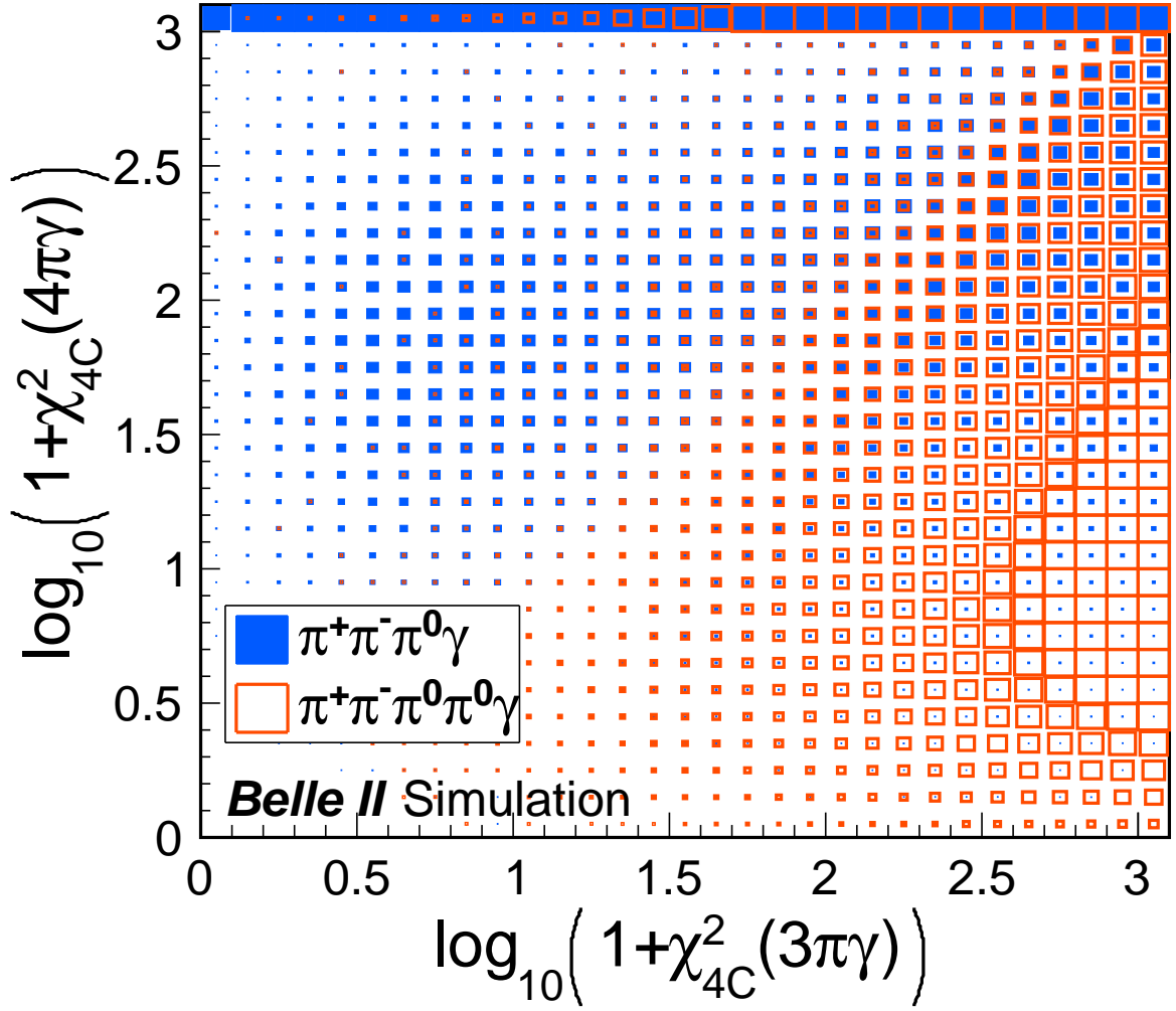
FIG. 3: The \chi^2 distribution of four-momentum conservation kinematic fit under e^+e^- \rightarrow \pi^+\pi^-\pi^0\gamma hypothesis (horizontal axis) and e^+e^- \rightarrow \pi^+\pi^-\pi^0\pi^0\gamma hypothesis (vertical axis). The blue area shows e^+e^- \rightarrow \pi^+\pi^-\pi^0\gamma MC, and red square shows e^+e^- \rightarrow \pi^+\pi^-\pi^0\pi^0\gamma MC. The area indicates the number of events of MC samples. The top row shows the events where an additional \pi^0 is not found and \pi^+\pi^-\pi^0\pi^0\gamma candidates cannot be reconstructed.
