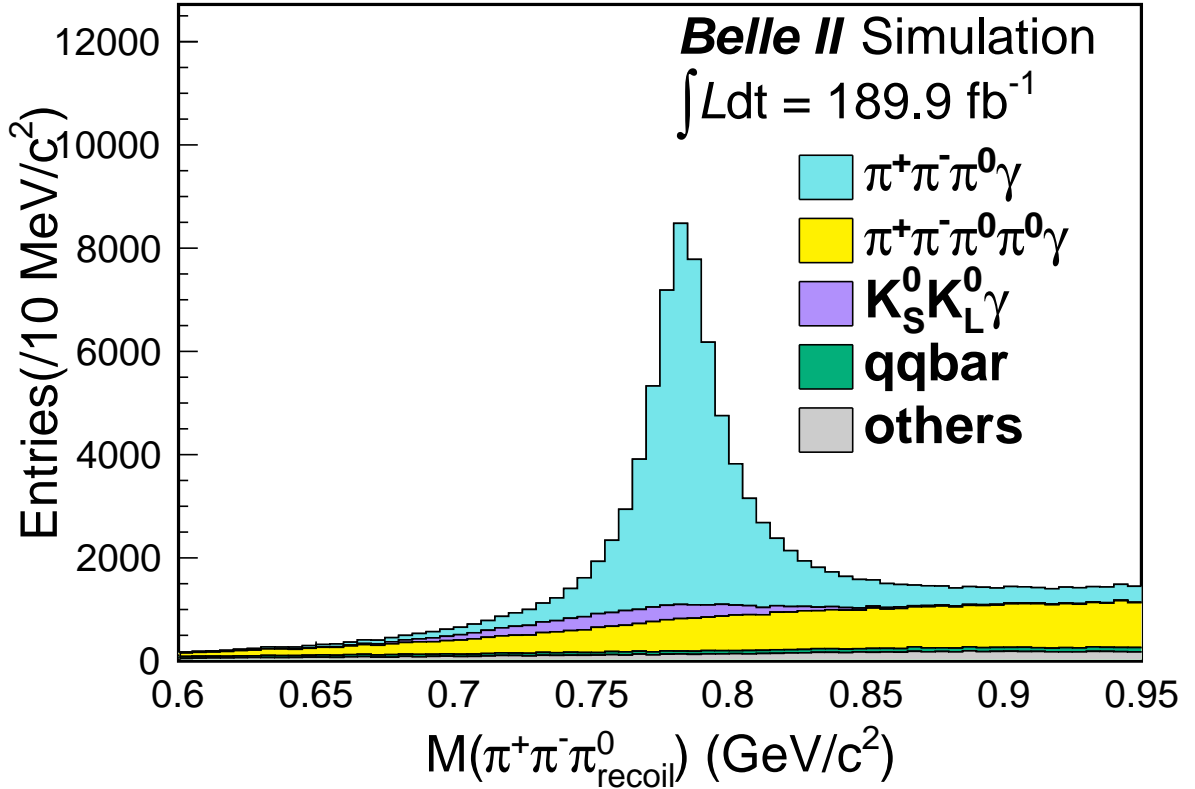
FIG. 9: The M(\pi^+\pi^-\pi_{\text{recoil}}^0) distribution of the partial-reconstructed sample for the \pi^0 efficiency study. The M(\pi^+\pi^-\pi_{\text{recoil}}^0) is calculated from the four vector of charged pions and the recoil momentum after a kinematic fit to \pi^+\pi^-\gamma with a constrain of the recoil mass to be the \pi^0 mass. The stacked histograms are MC samples scaled by the integrated luminosity.
