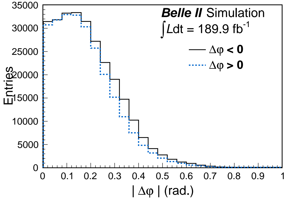
FIG. 8: The |\delta\varphi| distribution of \pi^+\pi^-\pi^0\gamma signal at the \omega resonance. The lines indicate \Delta\varphi < 0 events (solid) and \Delta\varphi > 0 (dashed) of e^+e^- \rightarrow \pi^+\pi^-\pi^0\gamma MC.
