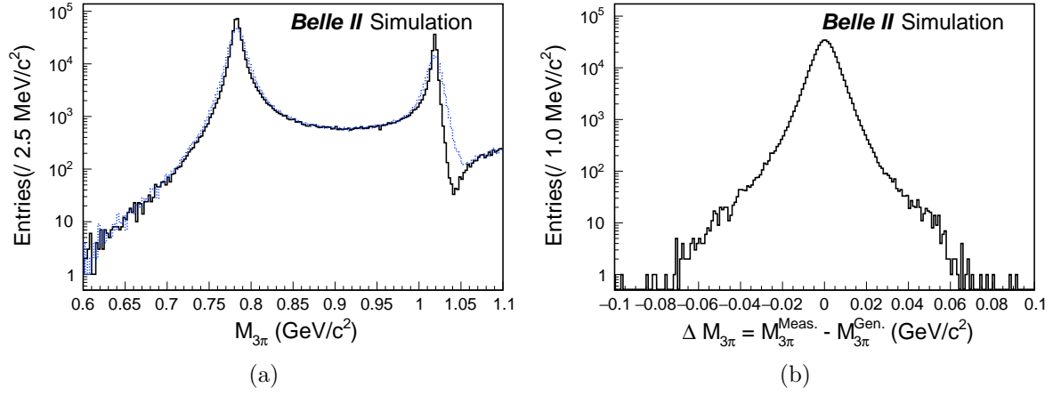
FIG. 11: (a) M(\pi^+\pi^-\pi^0) spectrum of measured value (solid) and generator value (dashed) of e^+e^- \rightarrow \pi^+\pi^-\pi^0\gamma MC. (b) M(\pi^+\pi^-\pi^0) difference of measured value (solid) and generator value (dashed) of e^+e^- \rightarrow \pi^+\pi^-\pi^0\gamma MC.
