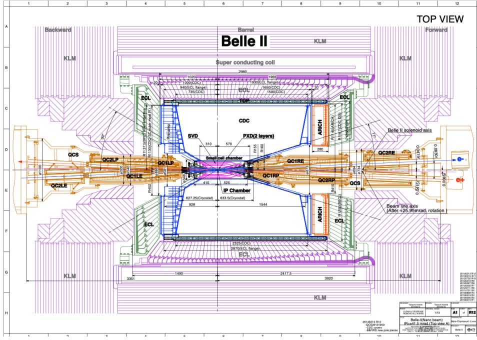
Figure 7.2: Top view of the Belle II detector [79].
