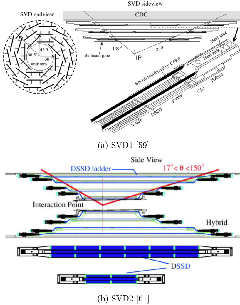
Figure 3.3: Detector configuration of SVD .
