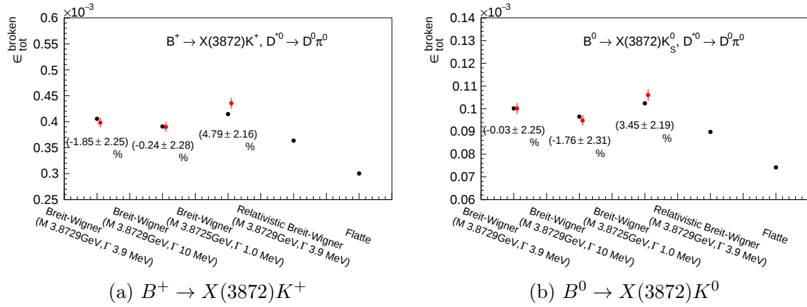
Figure 5.16: Total broken-signal efficiency for five lineshapes when the M(D^0 \bar{D}^{*0}) range is to 4.0 \text{ GeV}/c^2 : from left, the signal MC samples with a mass of 3.8729 \text{ GeV}/c^2 and a width of 3.9 \text{ MeV} , the signal MC samples with a mass of 3.8729 \text{ GeV}/c^2 and a width of 10 \text{ MeV} , the signal MC samples with a mass of 3.8725 \text{ GeV}/c^2 and a width of 1.0 \text{ MeV} , the relativistic Breit-Wigner with a mass of 3.8729 \text{ GeV}/c^2 and a width of 3.9 \text{ MeV} and the Flatté lineshape with the parameters of Eq. (2.20). In each panel, black points represent the calculation method results, and red points represent the results obtained by counting the number of events. The values under the points show the relative difference between the methods.
