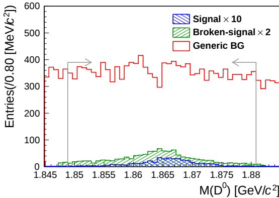
(a) D^0 candidate reconstructed with \pi^0
