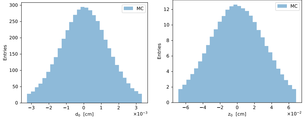
Figure 4.2: Histograms of the parameters d_0 (left) and z_0 (right) for the MC.
