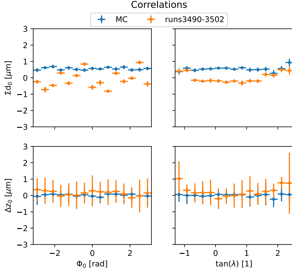
Figure A.4: Detail on correlations of the helix parameters for muons from collisions.
