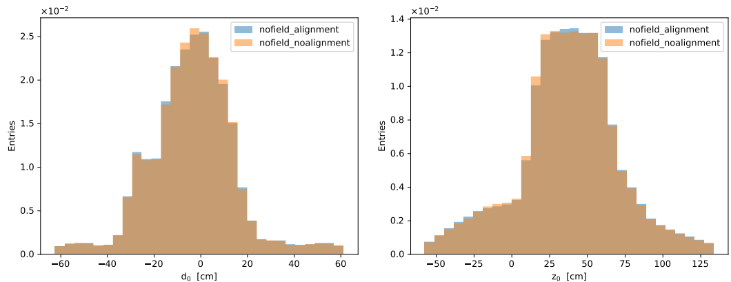
Figure 3.1: Histograms of the parameters d_0 (left) and z_0 (right) for all cosmics without any cuts.
