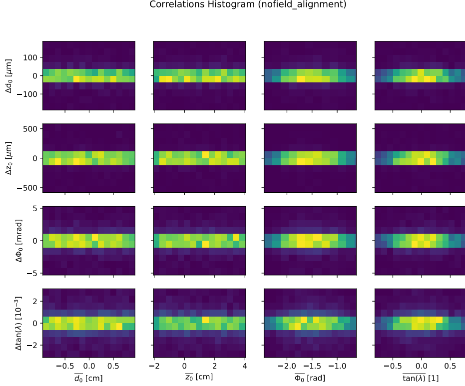
Figure 3.6: Histogram of correlations of the helix parameters for cosmic muons with alignment with the beampipe cut 3.1. Lighter colors signify larger number of events.
