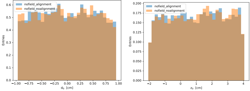
Figure 3.2: Histograms of the parameters d_0 (left) and z_0 (right) for cosmuics with a beampipe cut (shown in equation 3.1).
