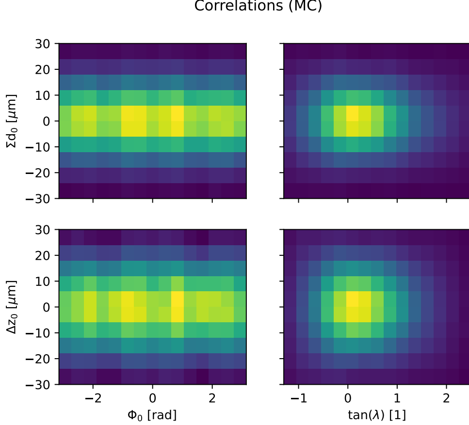
Figure 4.6: Histogram of correlations of the helix parameters for the MC.
