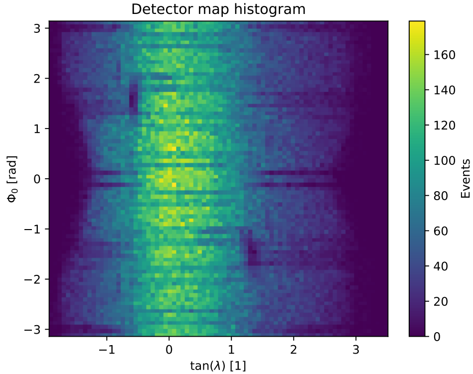
Figure A.2: Distribution of tracks for muons from colisions (runs3490-3502).
