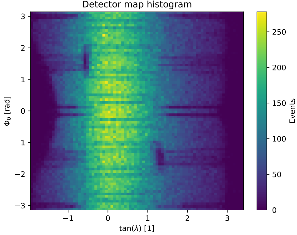
Figure 4.1: A 2D histogram of all muons from collisions (MC).
