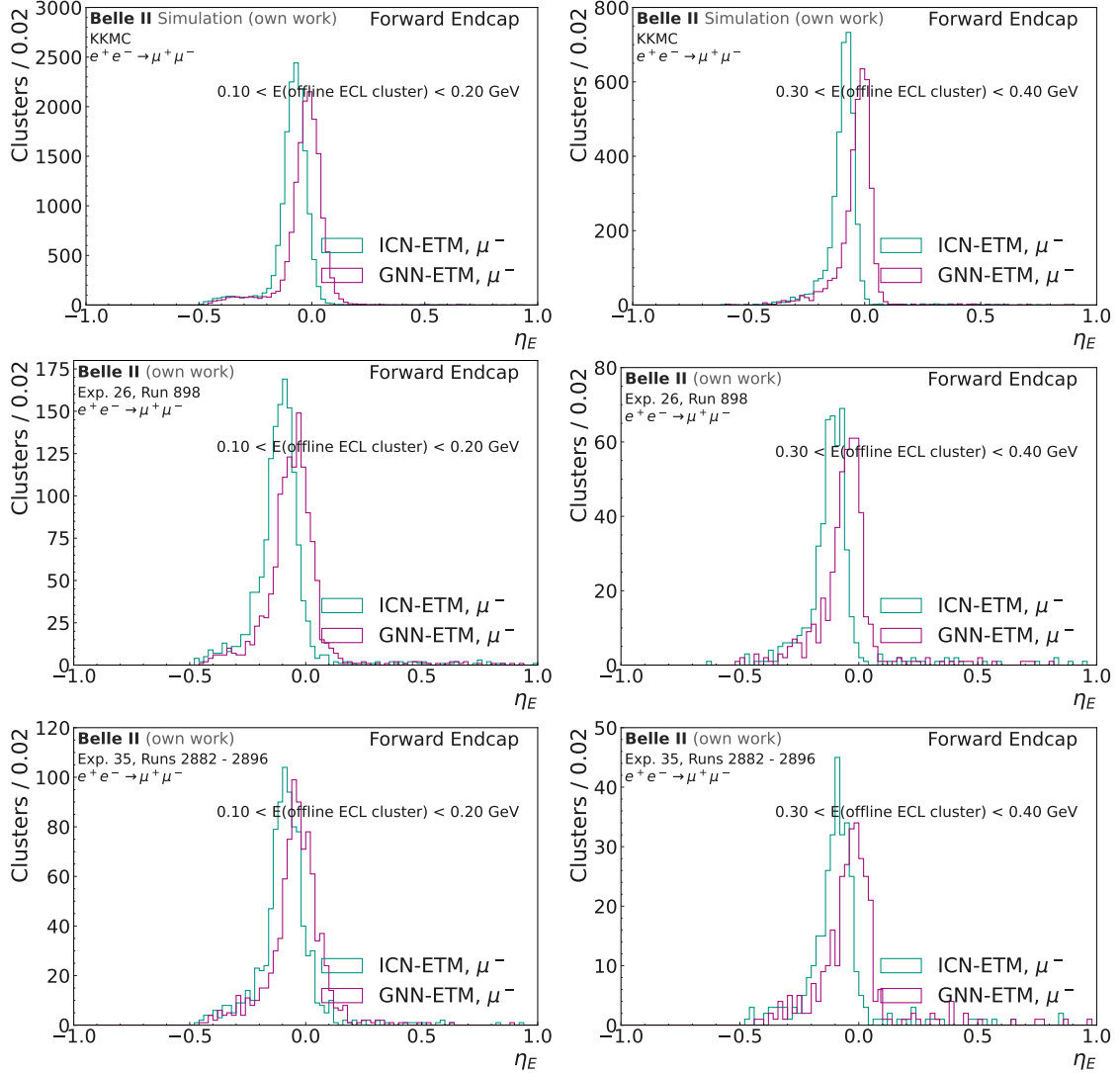
Figure D.18: \eta_E for GNN-ETM and ICN-ETM clusters matched to the \mu^- offline ECL cluster for 0.1 < E(\text{offline ECL cluster}) < 0.2 \text{ GeV} (left) and 0.3 < E(\text{offline ECL cluster}) < 0.4 \text{ GeV} (right). The top row shows the position resolution on the MC dataset, the center row on the Exp. 26 dataset and the bottom row on the Exp. 35 dataset. The resolution is shown for offline ECL clusters in the forward endcap.
