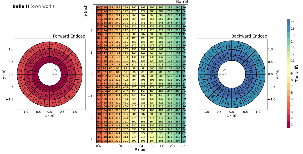
Figure 3.5: TC placement in the ECL. The current TC setup consists of 576 TC, shown here with their corresponding TC ID. The color of the TC denotes the \theta ID, going from 1 in the innermost forward endcap to 17 in the innermost backward endcap. Each TC also has a \phi ID, which ranges from 1 to 36 with 1 starting at \phi = 0^\circ (not depicted in this figure).
