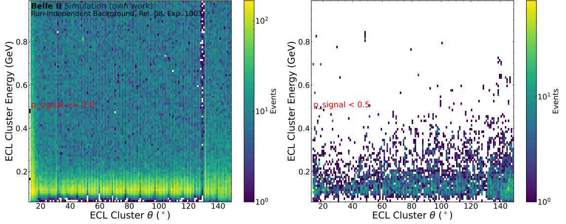
Figure 7.10: The energy of the matched offline ECL cluster versus its reconstructed \theta position. The left plot shows clusters with a signal classifier value \geq 0.5 , so more likely being signal, while the right plot shows clusters with a signal classifier value below 0.5. While structures such as the gap in the ECL at 130^\circ are visible, no evident structure of the classifier output can be seen.
