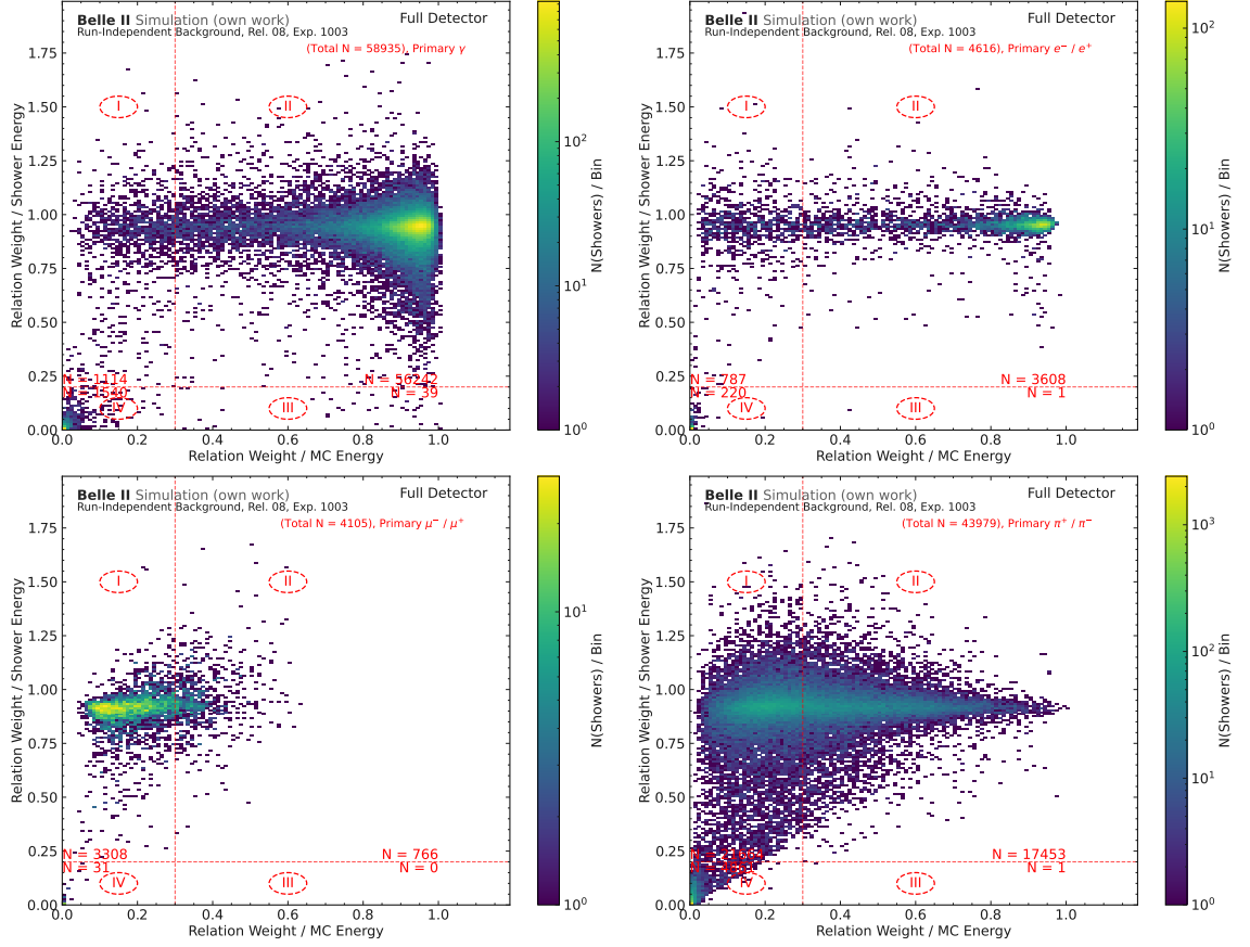
Figure 4.12: Cluster Ratio (y-Axis) over MC Ratio (x-Axis) for offline ECL clusters with energy depositions from primary particles originating from 10000 e^+e^- \rightarrow B^0\bar{B}^0 decays. One offline ECL cluster only appears in a single plot, as it is assigned to the particle with the highest MC Ratio. The top left plot shows the distribution for primary photons, top right for primary electrons, lower left for primary muons and lower right for primary pions. The red lines indicate the basf2 standard cuts of 0.2 and 0.3 to label a offline ECL cluster as MC matched.
