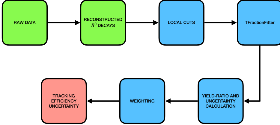
Figure 5.1: Overview of the analysis procedure.
