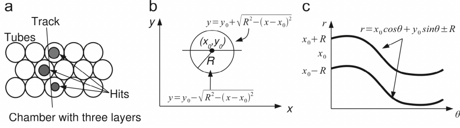
Figure 4.2: (a) A charged track passing by CDC wires and their drift circles. (b) Piecewise definition of a circle. (c) r - \theta representation of the Legendre transformed circle [5].
