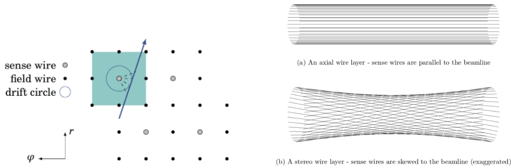
Figure 3.19: A wire cell inside the CDC [39].
