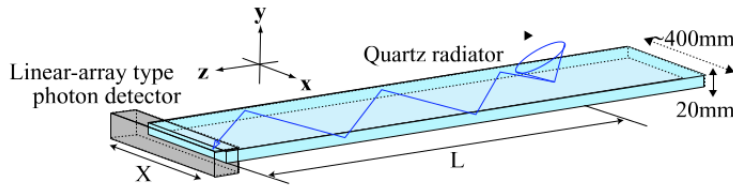
Figure 3.25: Schematic 3-D render of a TOP counter [2].
