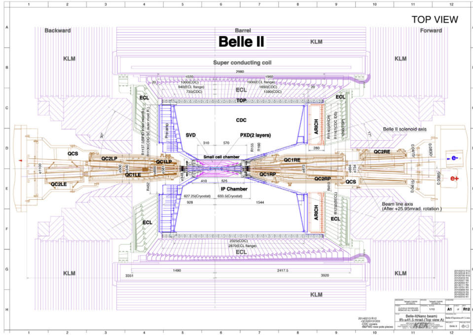
Figure 3.14: Top view of the Belle II layout [3]
