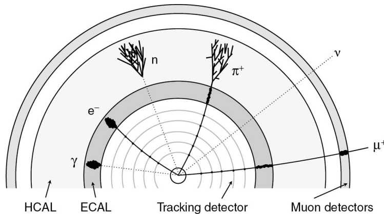
Figure 3.2: Schematic detector layout surrounding the interaction point [40].
