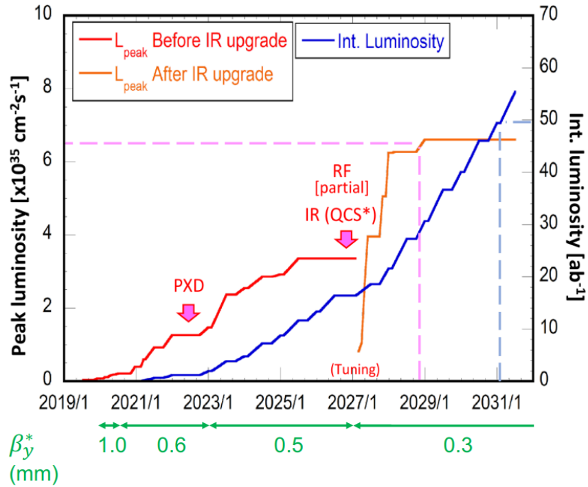
Figure 3.12: Roadmap for the luminosity of SuperKEKB [41].
