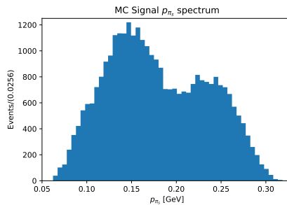
Figure 2.8: p_{\pi_s} spectrum from D^{*-} \rightarrow \bar{D}^0 \pi_s^- decays.
