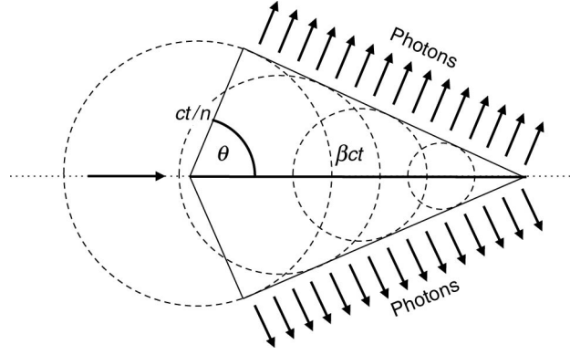
Figure 3.9: Geometric construction for Cherenkov radiation [40].
