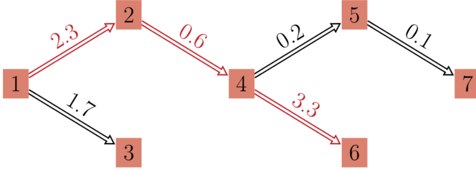
Figure 4.6: Example of path finding by maximizing the sum of weights using a cellular automaton. Here, the red path yields the largest sum [14].
