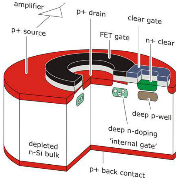
Figure 3.17: Schematic of a DEPFET [34].
