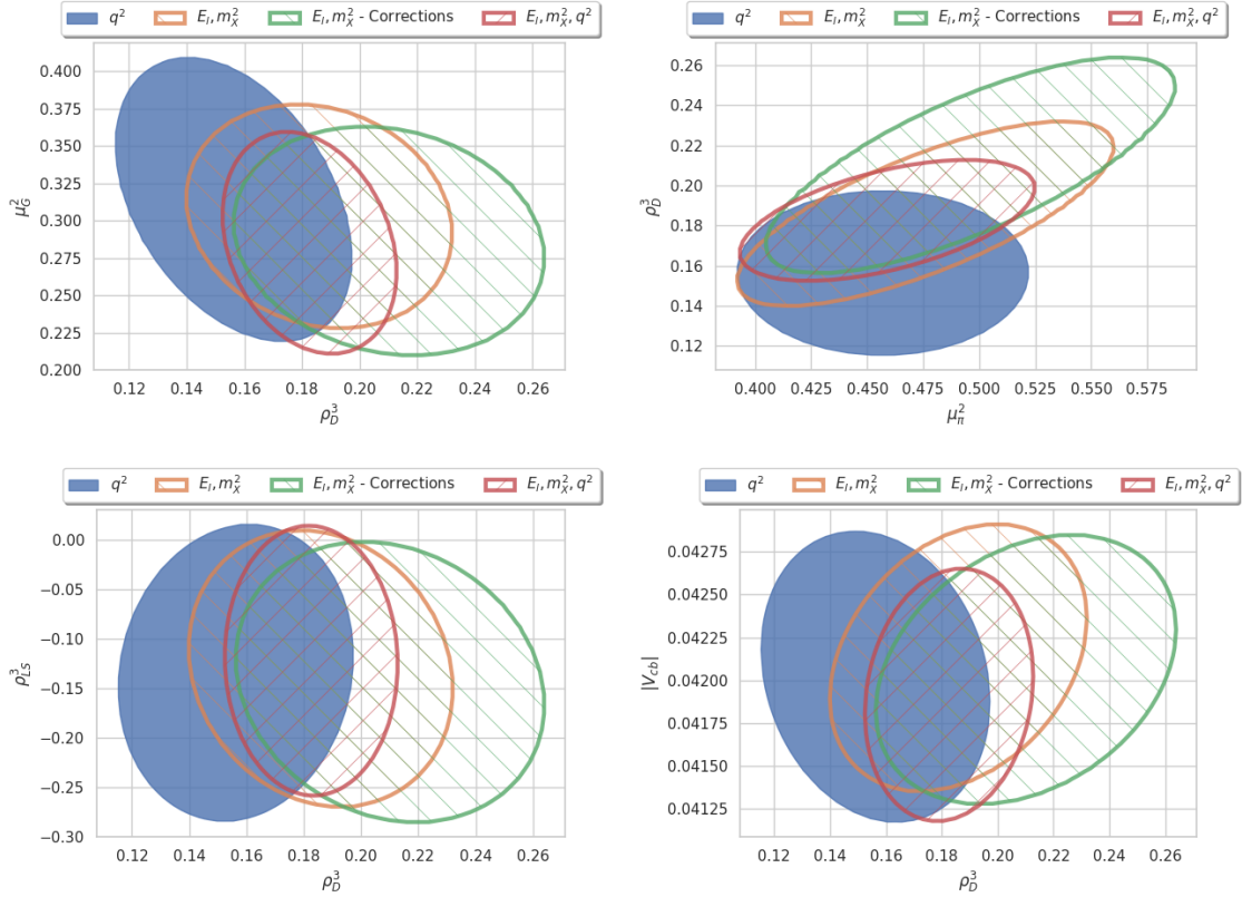
Figure 7.2: Regions of \Delta\chi^2 < 1 in the 2D planes (\rho_D^3, \mu_G^2) (upper left), (\mu_\pi^2, \rho_D^3) (upper right), (\rho_D^3, \rho_{LS}^3) (lower left) and (\rho_D^3, |V_{cb}|) (lower right). The blue region corresponds to the fit on only q^2 with additional constraints on BR_{cl\nu} and \mu_\pi^2 . E_l & m_X fits are shown in orange (without correction) and green (with the corrections). The red outline corresponds to the fit on E_l , m_X & q^2 moments.
