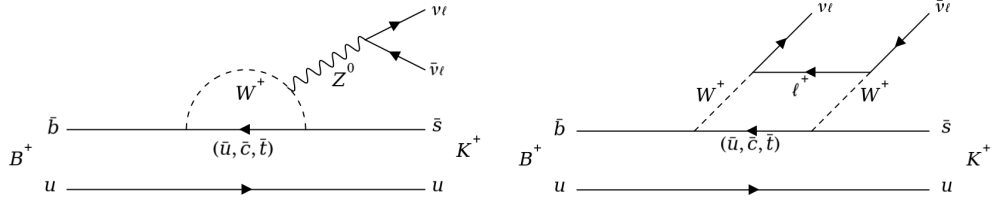
Figure 3.7: Leading order Feynman diagrams, an electroweak penguin (left) and a box diagram (right), for the quark level transition b \rightarrow s \nu \bar{\nu} \ell^+ \ell^- , responsible for the decay B^+ \rightarrow K^+ \nu \bar{\nu} .
