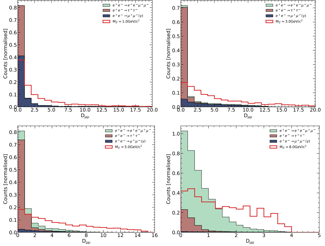
Figure 2.10: Distribution of D_{\mu\mu} for signal and background events that fall within 0.5\sigma of the signal peak of the given mass hypothesis.
