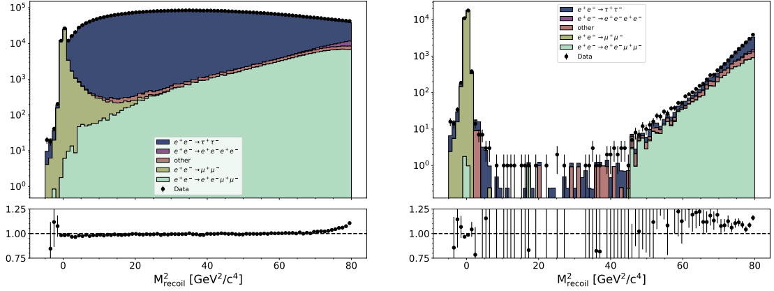
Figure 3.4: M_{\text{recoil}}^2 distribution of data and MC events in the e^+e^- \rightarrow e^\pm\mu^\mp control sample before (left) and after (right) the application of the Punzi-Net.
