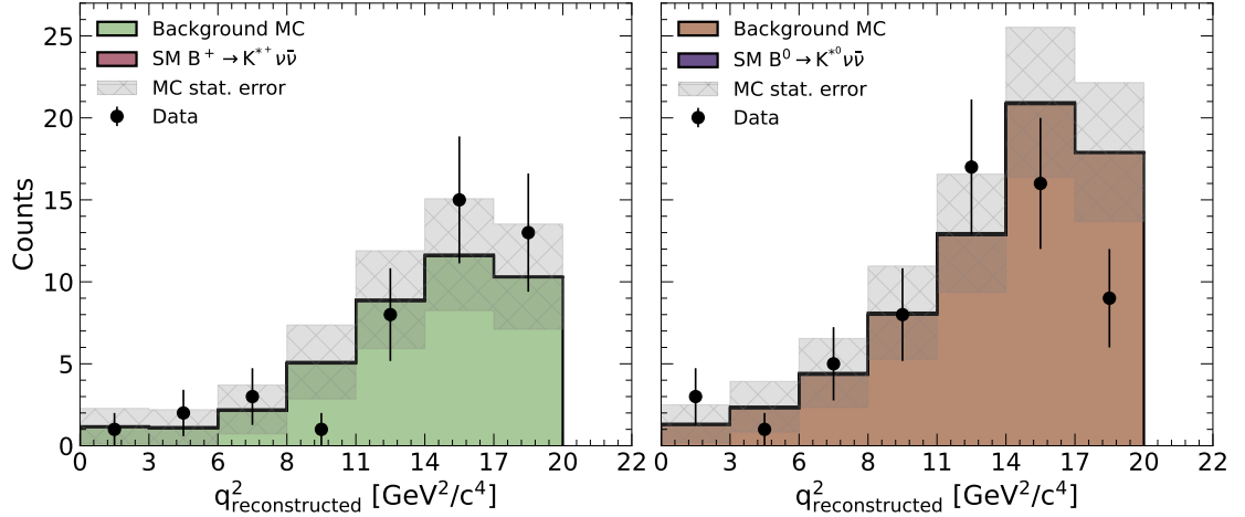
Figure 3.4: Reconstructed q^2 distributions of the studied B^+ \rightarrow K^{*+} \nu \bar{\nu} (left) and B^0 \rightarrow K^{*0} \nu \bar{\nu} (right) decays, provided by the BaBar collaboration. The expected standard model MC signal and backgrounds are shown, along with the observed data counts.
