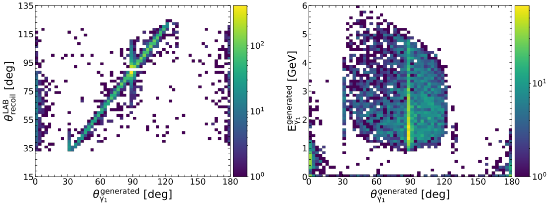
Figure 2.16: Left: distribution of the recoil polar angle and MC generated polar angle (LAB frame) of the photon in \mu^+\mu^-(\gamma) events that survive all selections due to the photon going undetected. This figure contains only events with M_{\text{recoil}}^2 \leq 4 \text{ GeV}^2/c^4 . Right: distribution of the MC generated energy and polar angle (LAB frame) of the photon in \mu^+\mu^-(\gamma) events that survive all selections due to the photon going undetected. This figure contains only events with M_{\text{recoil}}^2 \leq 4 \text{ GeV}^2/c^4 .
