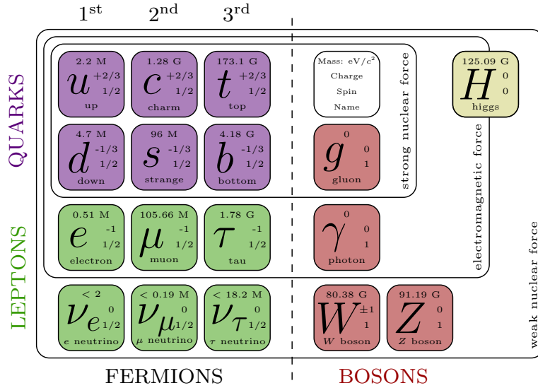
Figure 1.1: The particles of the Standard model shown divided into fermions and bosons, with the former also divided into the leptons and quarks. Each is shown with its mass, charge and spin.
