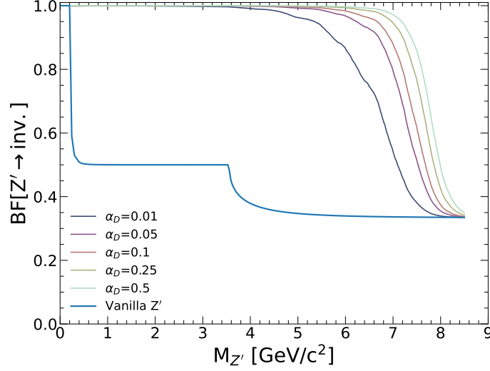
Figure 1.9: The branching fraction of the invisible decay mode for the Z' as a function of M_{Z'} . The L_\mu - L_\tau model is shown, along with the dark Z' model for which the distribution under multiple values of \alpha_D are shown.
