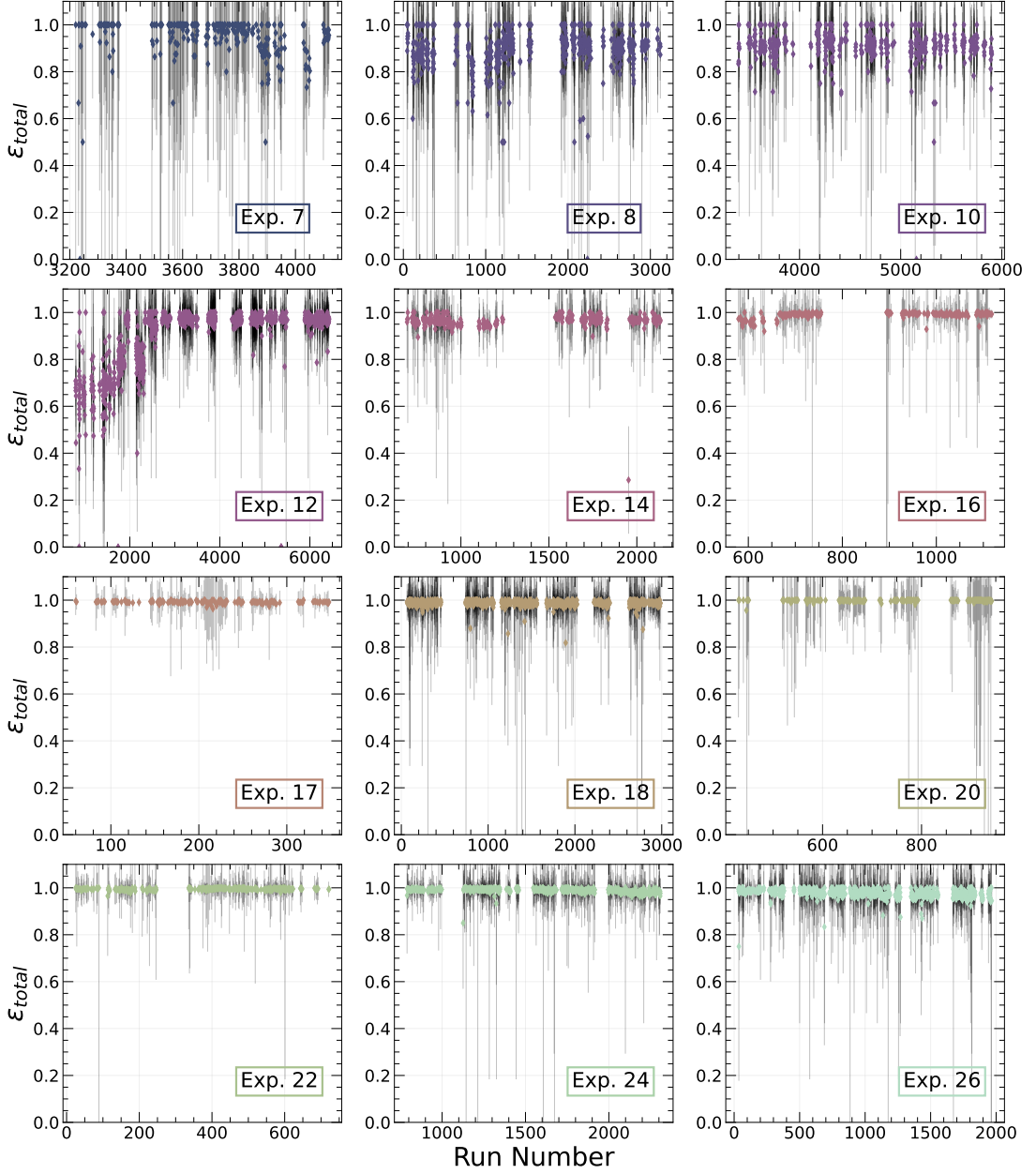
Figure 2.3: Trigger efficiency calculated for each run during each of the twelve experiments spanning the full data-taking period.
