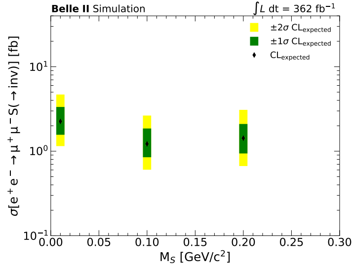
Figure 4.9: The 90% CL upper limits on the cross section for the mass hypotheses 10, 100 and 200 \text{MeV}/c^2 , along with the \pm 1, 2\sigma uncertainty bands shown in green and yellow.
