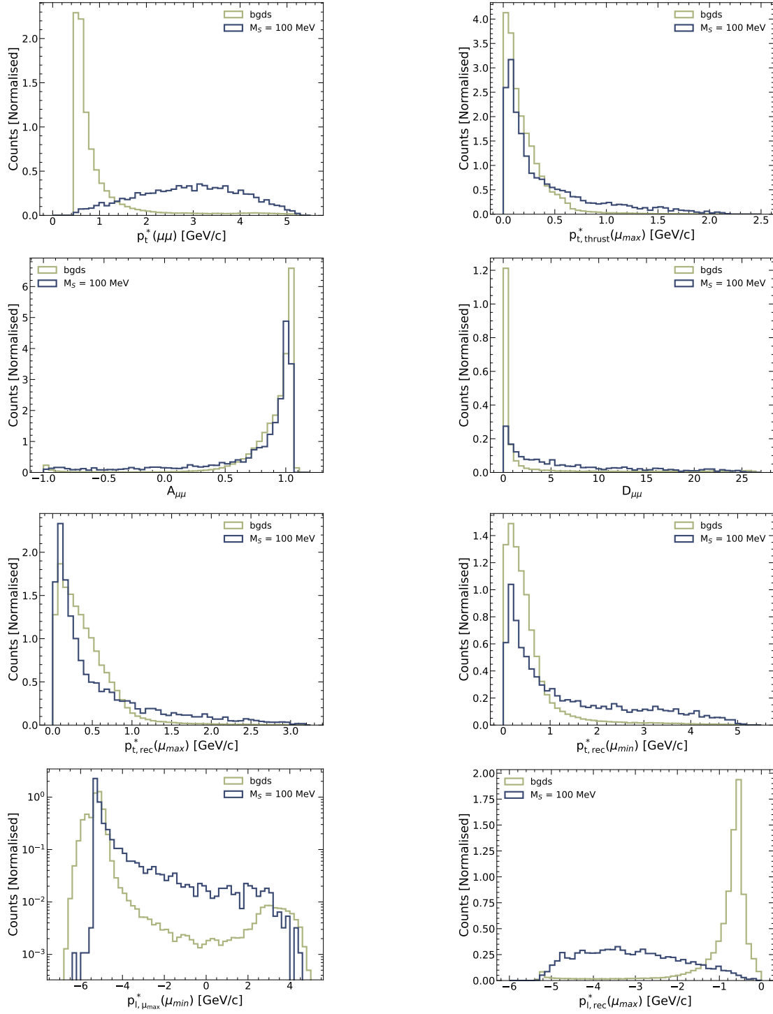
Figure 2.13: Signal and background distributions for the 8 input variables of the BDT used for selection in the muonphilic scalar search.
