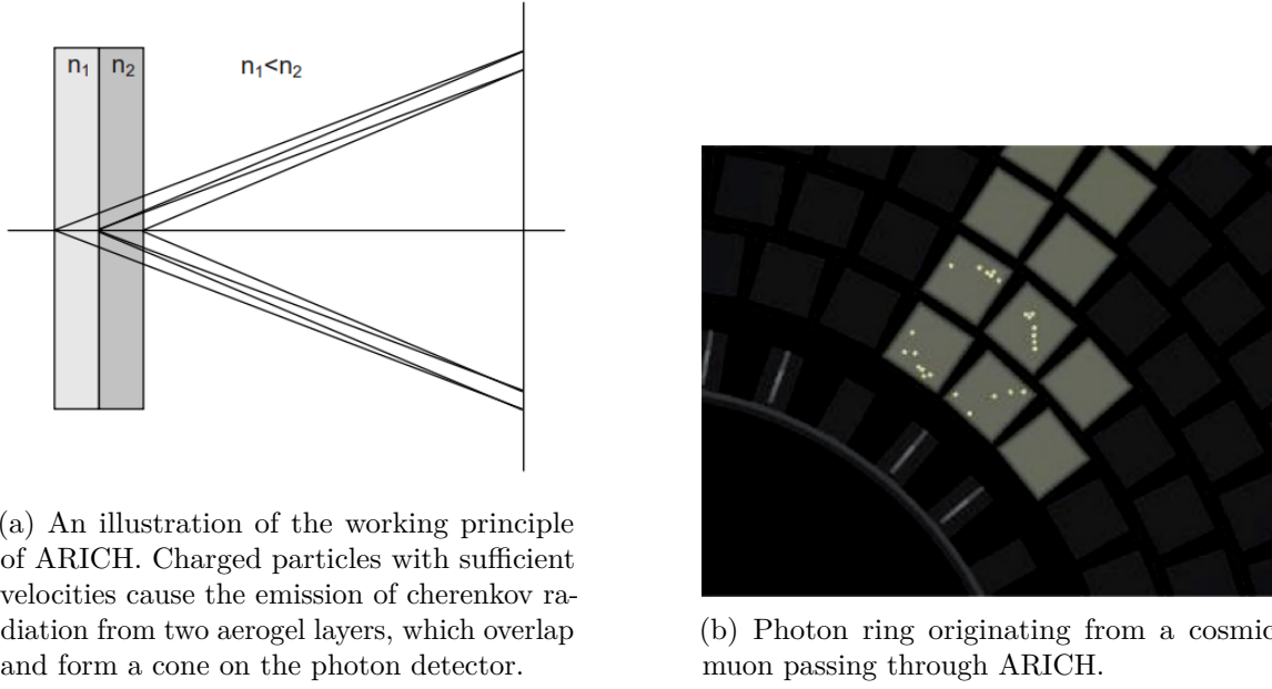
Figure 3.12: The layout of ARICH is depicted in Fig.a, while Fig.b shows the detected cone from a cosmic muon.[16]
