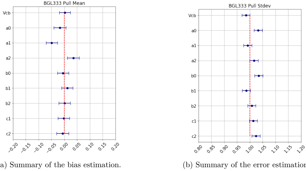
Figure 6.16: Results obtained from the pull test of the |V_{cb}| and form factor fit using the BGL 333 parameterization.
