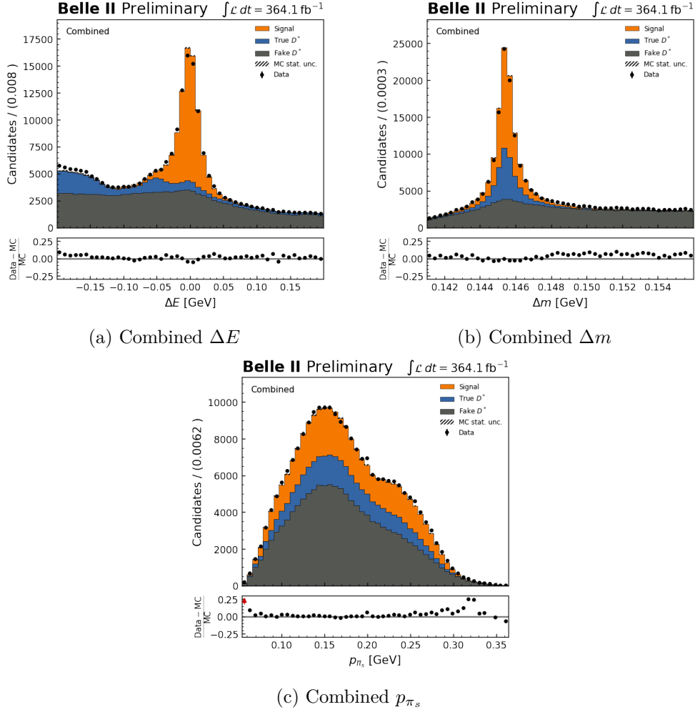
Figure 5.8: Shape comparison of pre-fit distribution of all variables relevant to the signal extraction for the combination of all decay channel. The signal, true D^{*-} and fake D^{*-} components of the MC are depicted by the orange, blue and gray components, respectively. Additionally the dots indicate the data. These figures only include statistical uncertainties.
