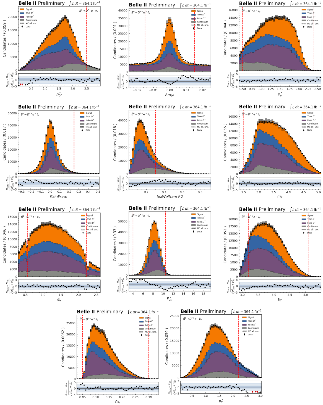
Figure A.6: On-resonance data and MC pre-fit agreement for the n-1 cutflow of B \rightarrow D^* e \nu .
