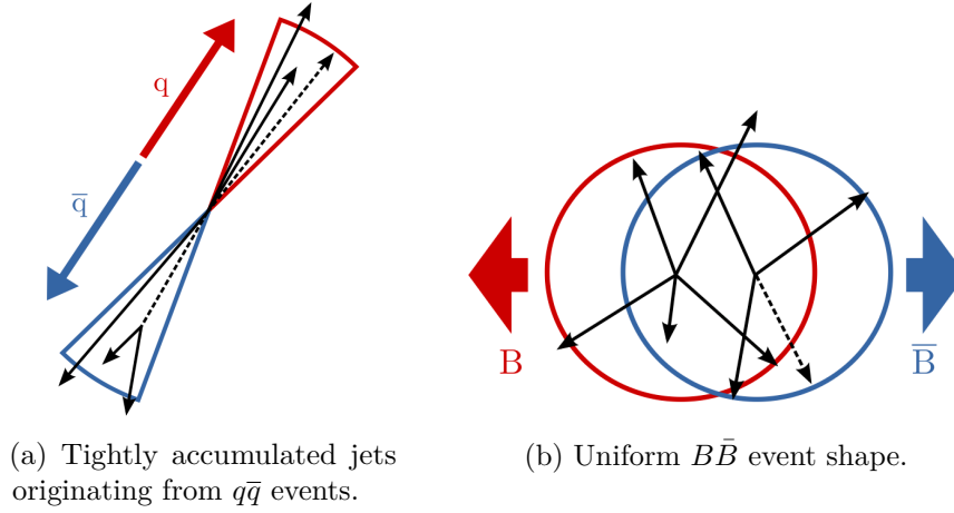
Figure 4.5: Comparison between the continuum and B\bar{B} event shapes. [49]
