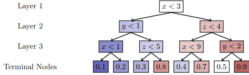
Figure 4.7: Schematic of a three layer decision tree. Each candidate has to traverse the tree until a terminal node is reached. A cut based decision is made at each node of the path for every candidate, here represented by the thresholds for three arbitrary variables x, y, z . This process ends, when a candidate finally reaches a terminal node that represents the probability of it being a signal candidate. The probability is based on the percentage of signal labeled candidates from the training-data that ended up on the node. [51]
