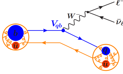
Figure 2.7: Feynman diagram of semileptonic B meson decays. [19]
