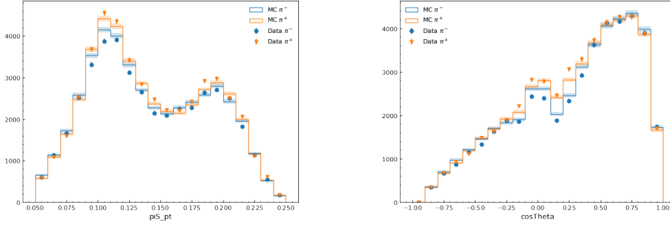
Figure 5.19: One dimensional comparison of the data and MC charge dependent efficiencies in bins of the transverse momentum of \pi_s p_T (left) and the cosine of the polar angle \cos\theta (right).
