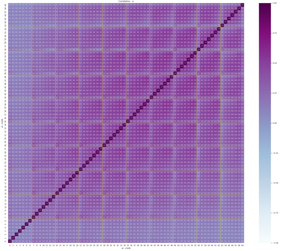
Figure 6.14: Statistical and systematic correlation matrix of B \rightarrow D^* e \nu_e .
