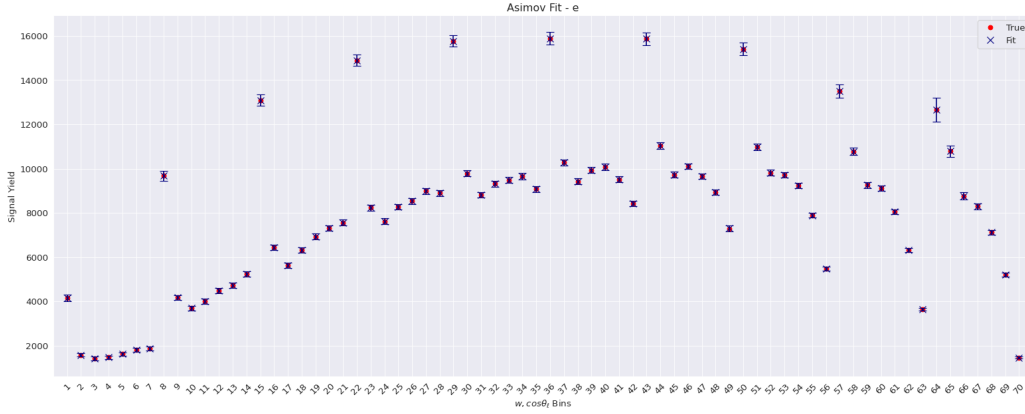
Figure 6.12: Asimov result of the B \rightarrow D^* e \nu_e channel, showing perfect agreement between the known signal yield and the yield estimated by the fit. The red dots indicate the true amount of signal events and the blue crosses with their respective uncertainties show the estimation.
