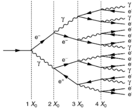
Figure 3.13: Development of electromagnetic showers in the ECL.[3]
