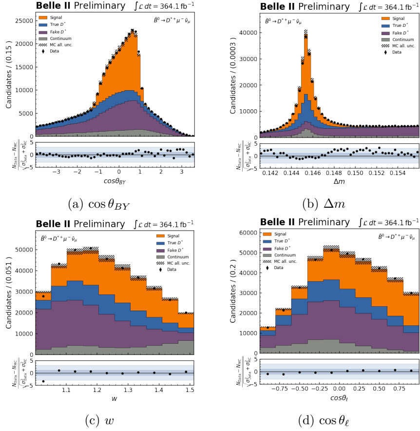
Figure A.8: Agreement between data and MC of the distributions of the parameters used during the signal extraction for B \rightarrow D^* \mu \nu_\mu .
