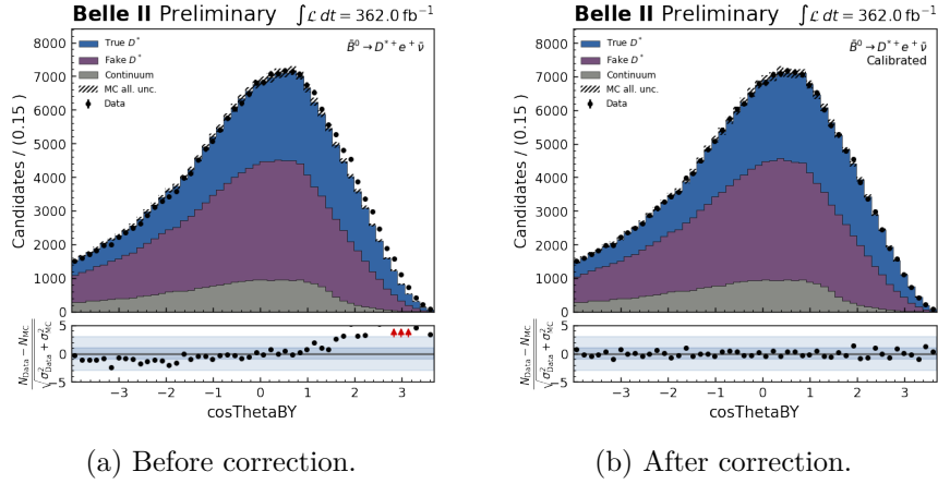
Figure 6.8: The comparison between the \cos \theta_{BY} distribution before and after the calibration is shown. It can be observed, that after the application of the newly calculated correction factors to the fake and true D^* component only very minor discrepancies from the continuum component are left over. This observation further solidifies the assumption, that the original disagreement is not caused by continuum events.
