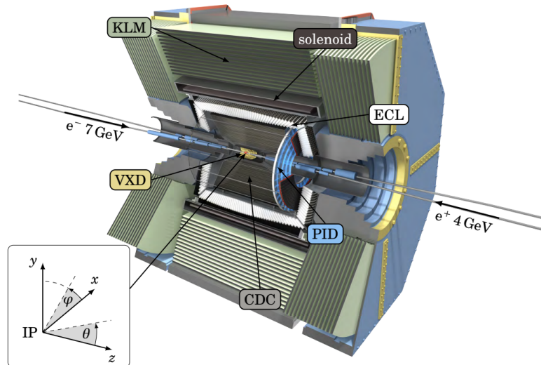
Figure 3.3: Schematic view of the Belle II detector, with its subdetectors indicated with arrows [51, 52]. The coordinate frame is superimposed in the bottom left corner.
