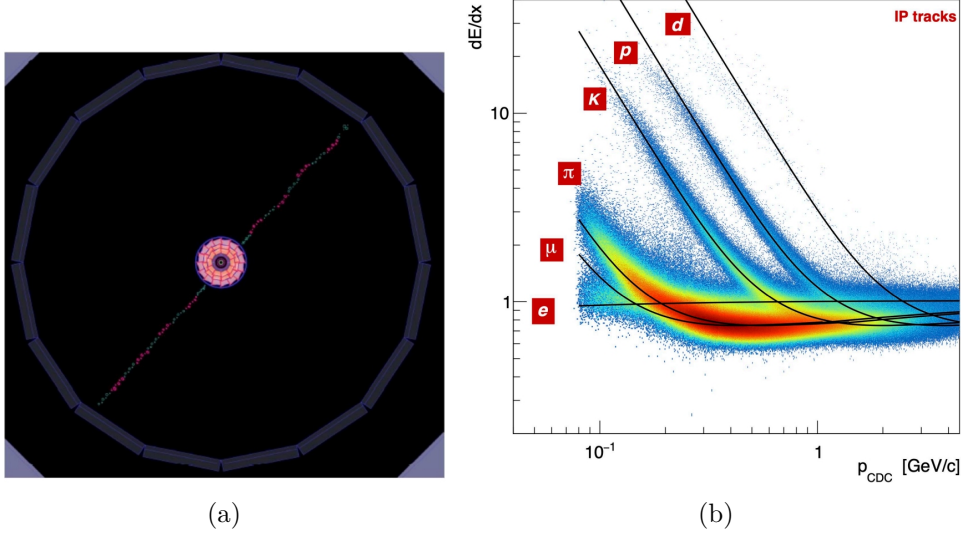
Figure 3.6: (a) A cosmic muon being tracked in the CDC [52]. (b) Characteristic dE/dx energy loss curves in the CDC [57].
