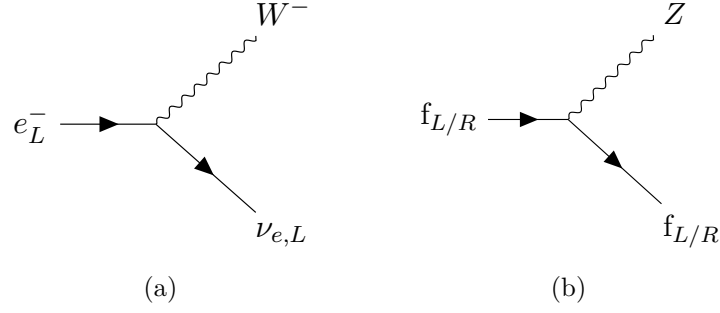
Figure 2.3: Feynman diagram of (a) charged-current and (b) neutral-current weak interactions. The letters L and R denote left- and right-handed chiral states.
