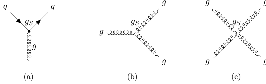
Figure 2.6: Feynman diagrams of (a) quark-gluon interactions, (b) three-point gluon self-interactions, and (c) four-point gluon self-interactions.
