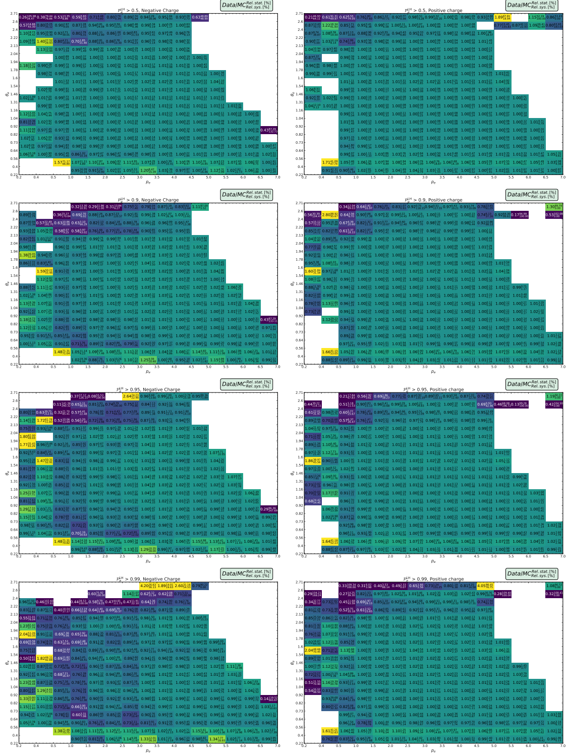
Figure A.3: Correction factors and uncertainties for likelihood-based global electronID with different thresholds and charges.
