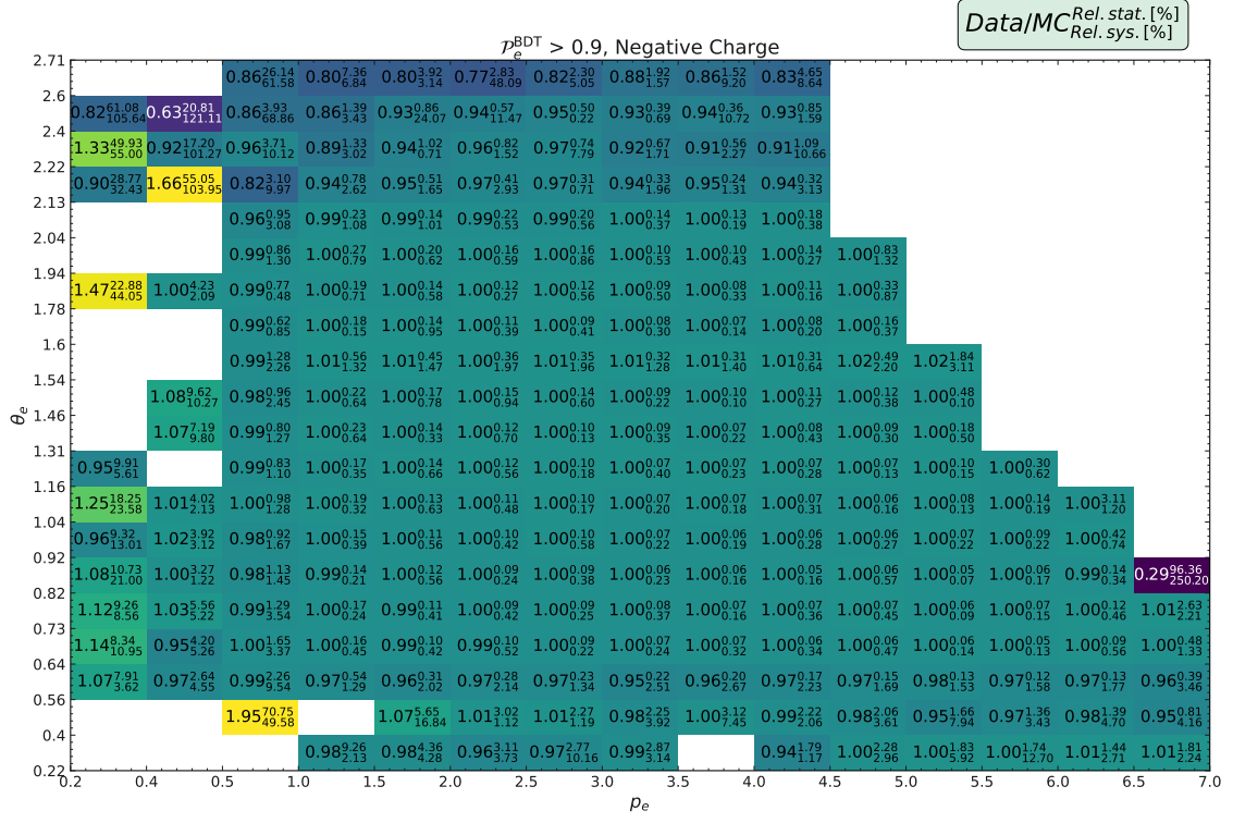
Figure 5.4: Results of correction factors with statistical and systematic uncertainty, for p_e^{\text{BDT}} > 0.9 and electrons.
