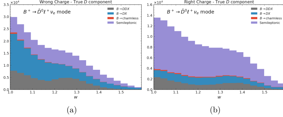
Figure 6.14: The compositions of the true D component when reconstructing while requiring the (a) wrong charge and (b) right charge combinations. A bigger share of semileptonic decays is observed in the right charge reconstruction. Among hadronic decays, there are proportionally more B \rightarrow DX decays in the wrong charge sample, particularly towards low w .
