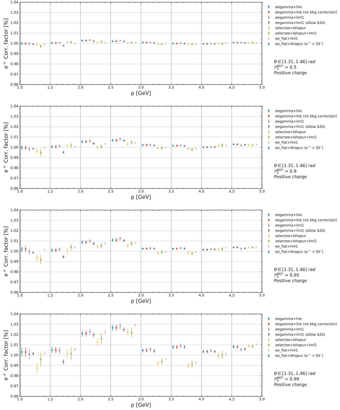
Figure 5.3: Differences in correction factors between control samples for multiple increasing thresholds from top to bottom. The correction factors shown are for positron momenta between 1 and 5 GeV in the barrel bin \theta \in [1.31, 1.46] rad and different \mathcal{P}_e^{\text{BDT}} selections.
