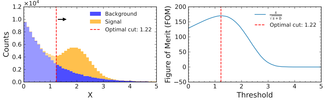
Figure 4.1: Stacked example histograms of an exponentially decaying background component and a Gaussian distributed signal component over a feature X . For each potential rectangular cut threshold X > \lambda , the right-hand side plot shows the FOM of the resulting sample. The optimal cut is shown as a red dashed line.
