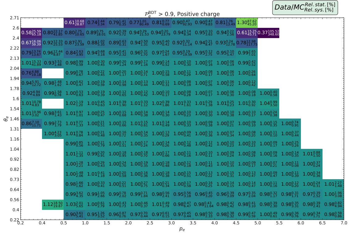
Figure 5.5: Results of correction factors with statistical and systematic uncertainty, for p_e^{\text{BDT}} > 0.9 and positrons.
