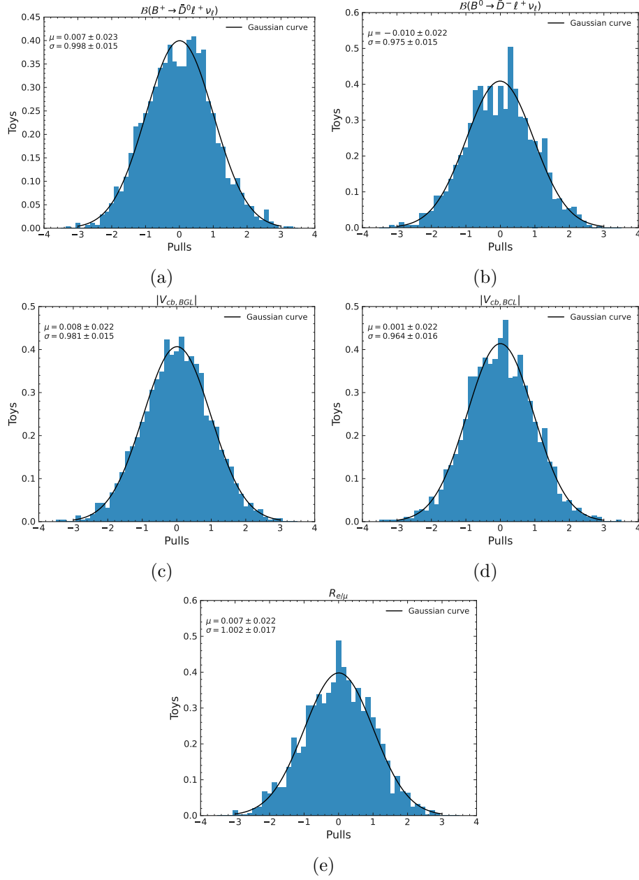
Figure 6.30: Pull distributions for the toy fit results for the average B^+ \rightarrow \bar{D}^0 \ell^+ \nu_\ell and B^0 \rightarrow D^- \ell^+ \nu_\ell branching ratios, |V_{cb}| with both BGL and BCL fits, and R_{e/\mu} .
