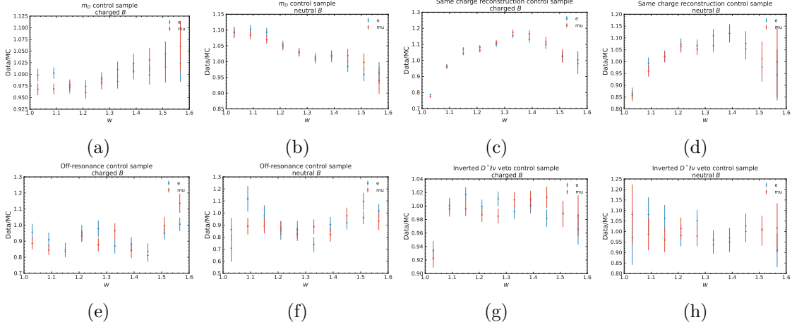
Figure 6.23: Data-MC ratios in bins of w in the background control samples.
