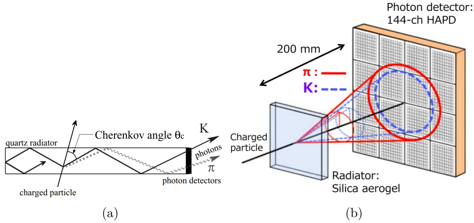
Figure 3.7: (a) Functioning principle of the TOP detector, with photons radiated at the Cherenkov angle \theta_c and subsequent propagation through the Quartz bar [54]. (b) Principle of the ARICH detector. The radius of the observed Cherenkov ring depends on the charged particles' mass [59].
