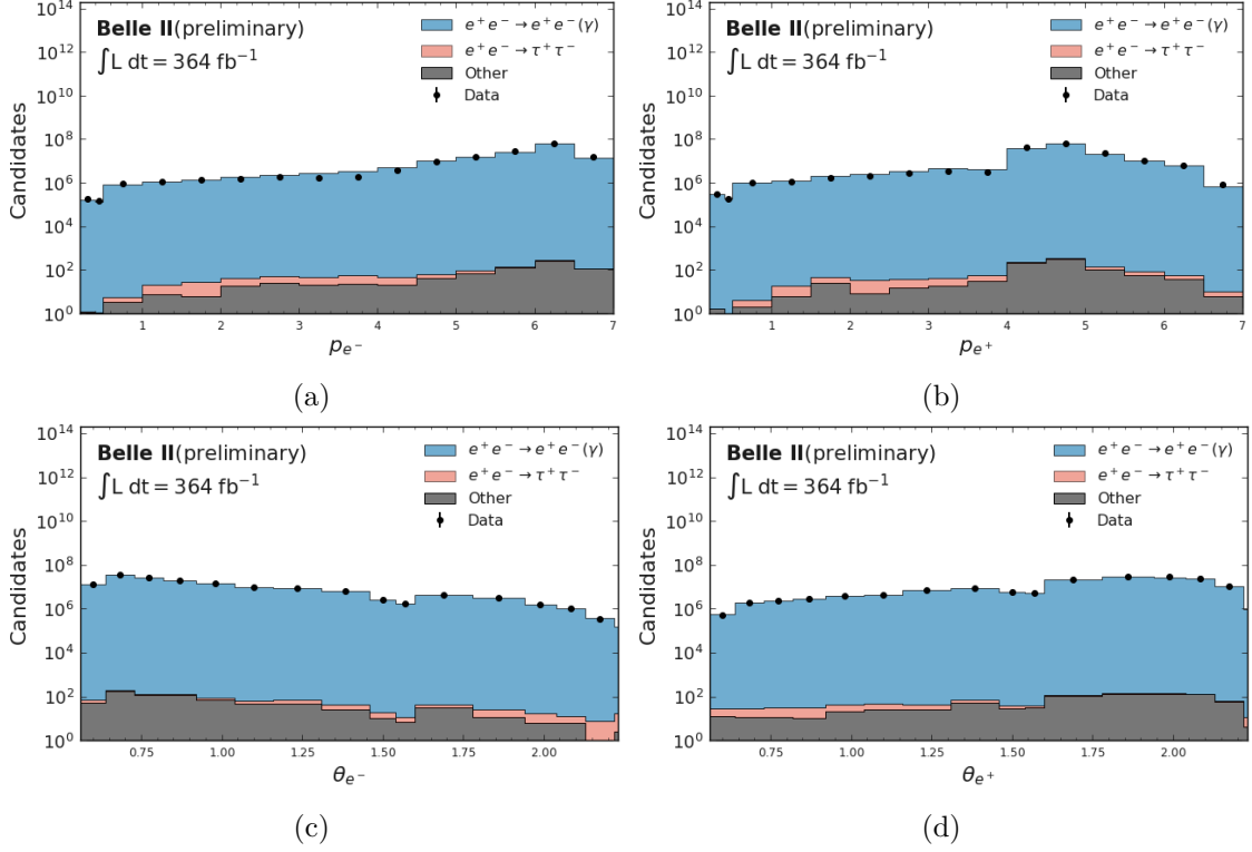
Figure 5.2: Laboratory frame momentum and polar angle distributions for the probe in reconstructed Bhabha events, with a loose electronID selection on the tag. The y axis is scaled logarithmically. The left plots shows electrons, and the right plots positrons.
