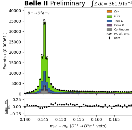
Figure 6.13: The plot shows the stacked \Delta m distributions for candidates where a slow \pi^+ fulfilling the requirements stated in Section 6.4.3 is found. A B \rightarrow D^*\ell\nu_\ell control sample can be defined by selecting candidates close to the peak.
