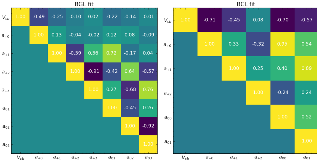
Figure 6.28: Correlation between BGL/BCL form factor parameters in the fit to MC.
