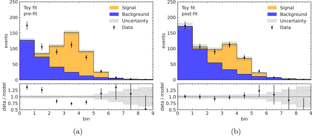
Figure 4.4: A fit to a toy data sample with a signal and background template. The histograms are shown before the fit on the left and after the fit on the right. Data is shown as black dots with error bars, and the expected templates from simulation as colored, stacked histograms. The overall normalization of the templates is left unconstrained, while shape variations are allowed in the templates according to their Poisson statistics. In this example, the signal yield in the toy data is significantly overestimated in simulation with respect to observed data.
