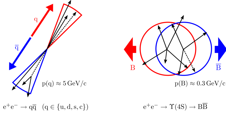
Figure 6.2: A schematic illustration of the geometrical event shape difference between continuum and B\bar{B} events [88].
