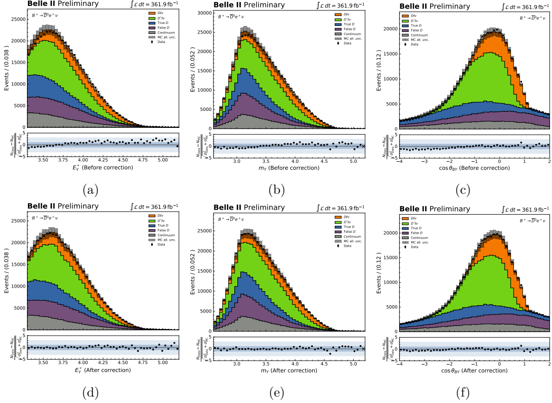
Figure 6.18: Data-MC agreements for the variables E_Y^* , m_Y and \cos\theta_{BY} in the nominal B^+ \rightarrow \bar{D}^0 e^+ \nu_e sample before (top) and after (bottom) applying the reweight correction.
