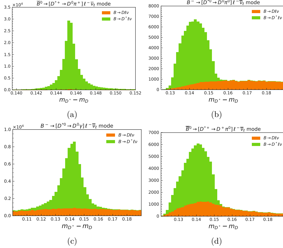
Figure 6.6: Distributions for the mass difference in each explicitly reconstructed B \rightarrow D^*\ell\nu_\ell mode after optimization of selections. The modes in (a) and (b) are used to veto candidates in B^+ \rightarrow \bar{D}^0\ell^+\nu_\ell reconstruction, while a veto of the mode in (d) is used for B^0 \rightarrow D^-\ell^+\nu_\ell .
