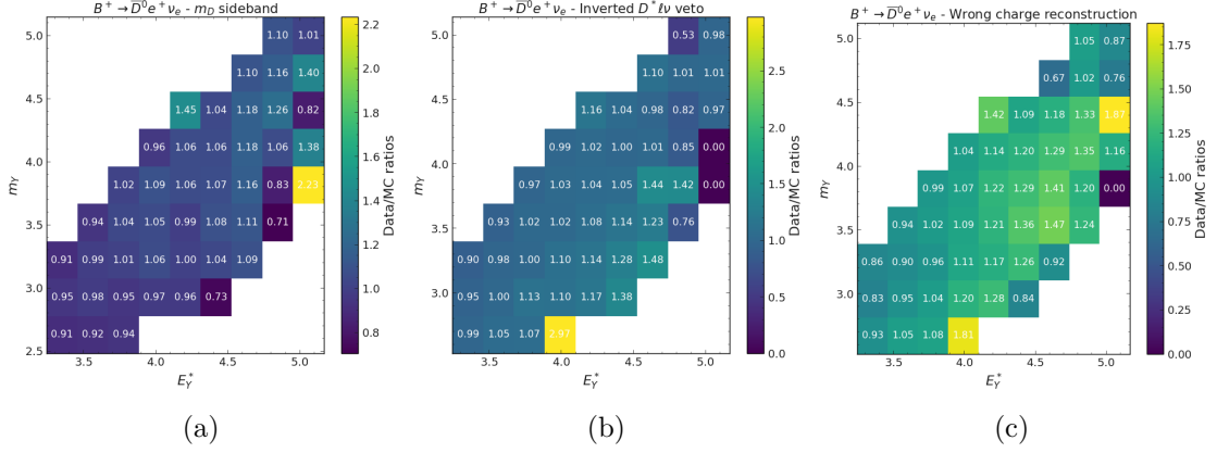
Figure 6.17: Correction factors derived from control samples in the B^+ \rightarrow \bar{D}^0 e^+ \nu_e mode.
