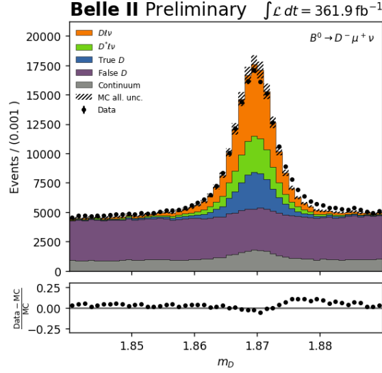
Figure 6.12: The m_D distribution peaks at the nominal D meson mass, with some width due to detector resolution. Combinatorial false D backgrounds dominate the sidebands outside of the signal region and can, therefore, be used as a control sample.
