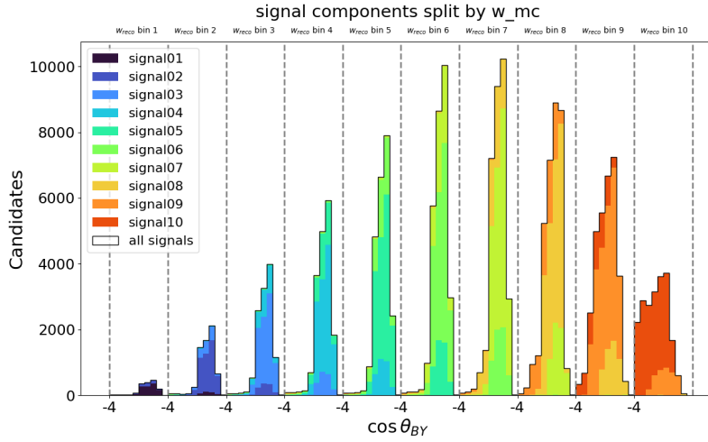
Figure 6.24: The signal templates \cos\theta_{BY} distributions in each bin of w flattened onto one combined axis. By categorizing the signal templates using w_{MC} rather than w_{reco} , migration effects between w bins are directly mapped into the fit.
