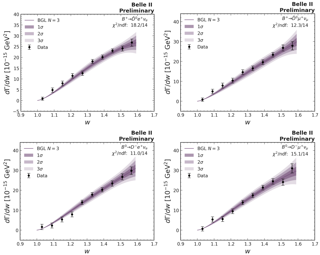
Figure 6.31: B \rightarrow D\ell\nu_\ell differential decay rates and the result of the BGL fit for all four final states.
