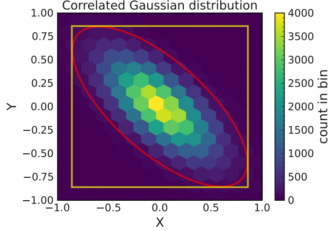
Figure 4.2: The plot shows a heatmap of an example signal distribution in two correlated variables X and Y . If overlaid on a uniform background distribution, the multivariate selection in the red ellipsis leads to a higher FOM than the optimized rectangular cuts in yellow.
