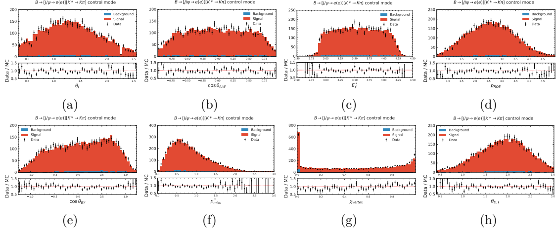
Figure 6.19: Distributions of selection variables in the B \rightarrow J/\psi K^* control sample with electrons in data and MC. Uncertainties are only statistical.
