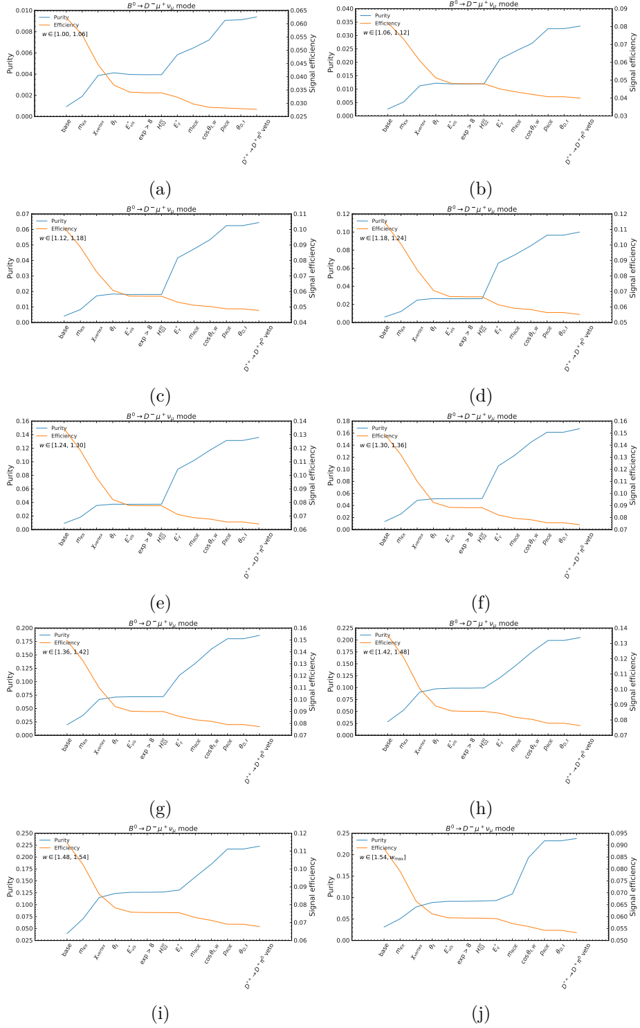
Figure B.4: Purity and signal efficiency in bins of w for the B^0 \rightarrow D^- \mu^+ \nu_\mu mode.
