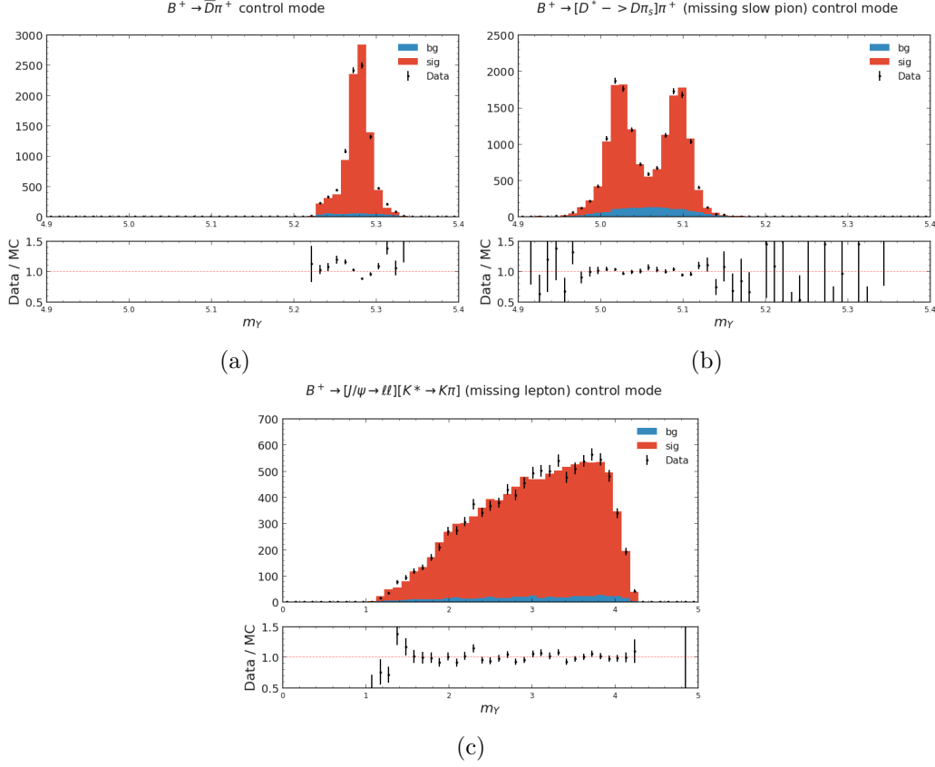
Figure 6.15: Distribution of the hadron-lepton system invariant mass in each control sample. The J/\psi mode has the highest amount of missing momentum and energy due to the missing second lepton in the reconstruction.
