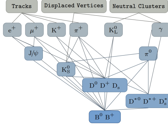
Figure 3.9: Schematic overview of the individual layers that each gather information and feed forward into other layers to reconstruct the tag-side B meson [74].
