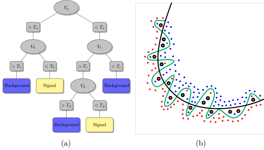
Figure 4.3: (a) Schematic view of a decision tree. Each node represents a test in a feature V_i , with thresholds T_i . After traversing each test, every instance in the training set is classified into signal or background [78]. (b) The green line schematically represents an overfitted model distinguishing blue and red categories. Individual decision trees are prone to overfitting; boosting can mitigate the effect by combining multiple decision trees into a single classifier output [79].
