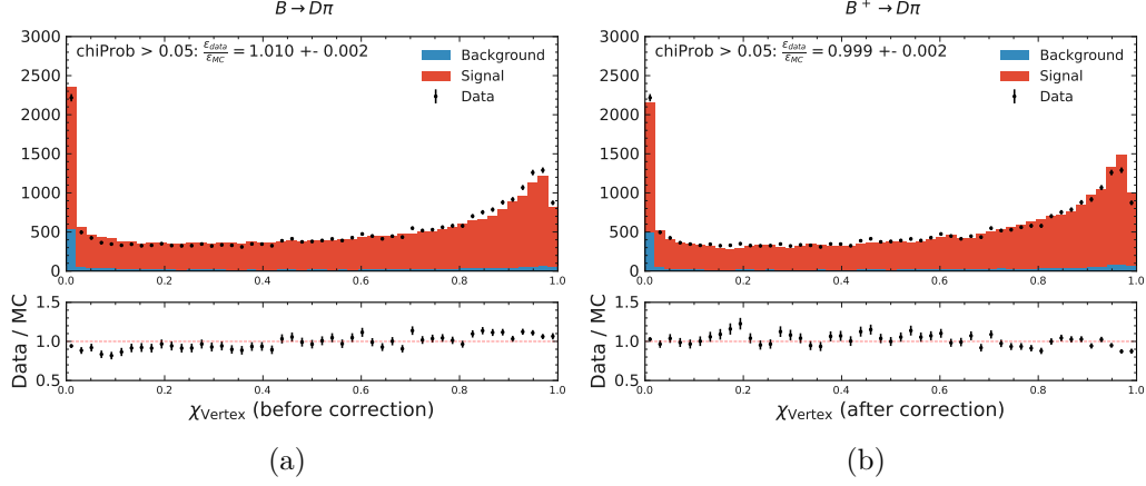
Figure 6.20: Vertex fit probability distribution in the B \rightarrow D\pi control sample before and after applying the correction calibrated on B \rightarrow J/\psi K^* decays. The selection efficiency ratio improves to move within the statistical uncertainty of unity.
