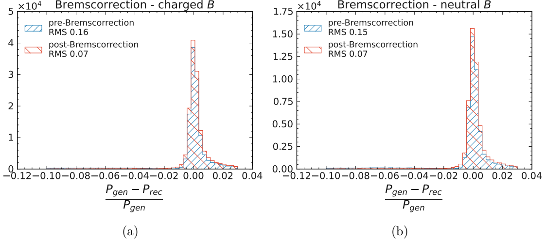
Figure 6.5: The resolution of electron momentum for truth-matched electrons in both the charged and neutral B modes. The blue curve shows the resolution before applying bremscorrection, while the red curve shows the improved resolution when allowing to correct electrons with radiated photons. The legends denote the root mean square deviations of the candidates.
