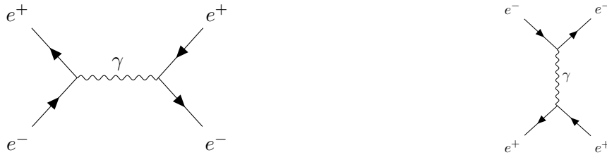
Figure 5.1: Feynman diagrams for e^+e^- \rightarrow e^+e^- in the s (left) and t (right) channels.
