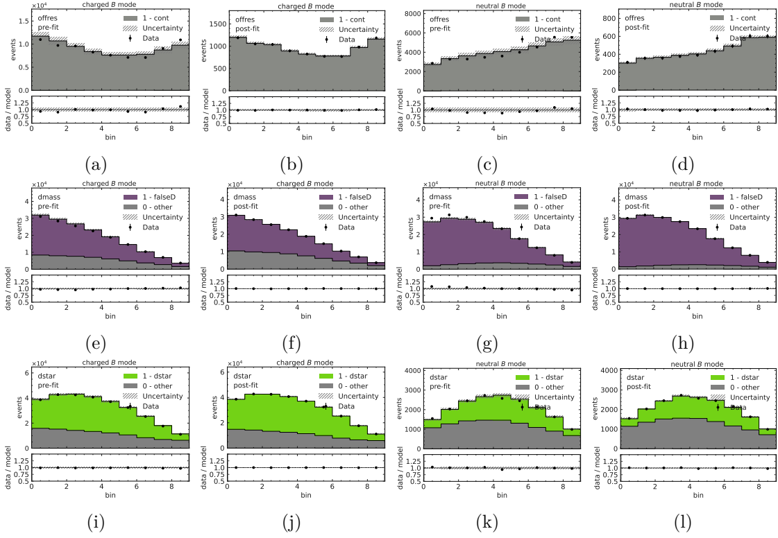
Figure 6.26: Pre- and post-fit plots for the fits to the background components in the control samples. The fit is performed separately for each control sample and for neutral and charged B modes.
