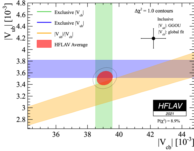
Figure 2.8: Experimental status of the observed discrepancy between exclusive and inclusive measurements of the CKM parameters |V_{cb}| and |V_{ub}| obtained from a global fit by the HFLAV group [3]. The experimental measurements and their global average are shown as colored bands and red ellipses, respectively. The inclusive measurement is shown as a black marker with error bars.
