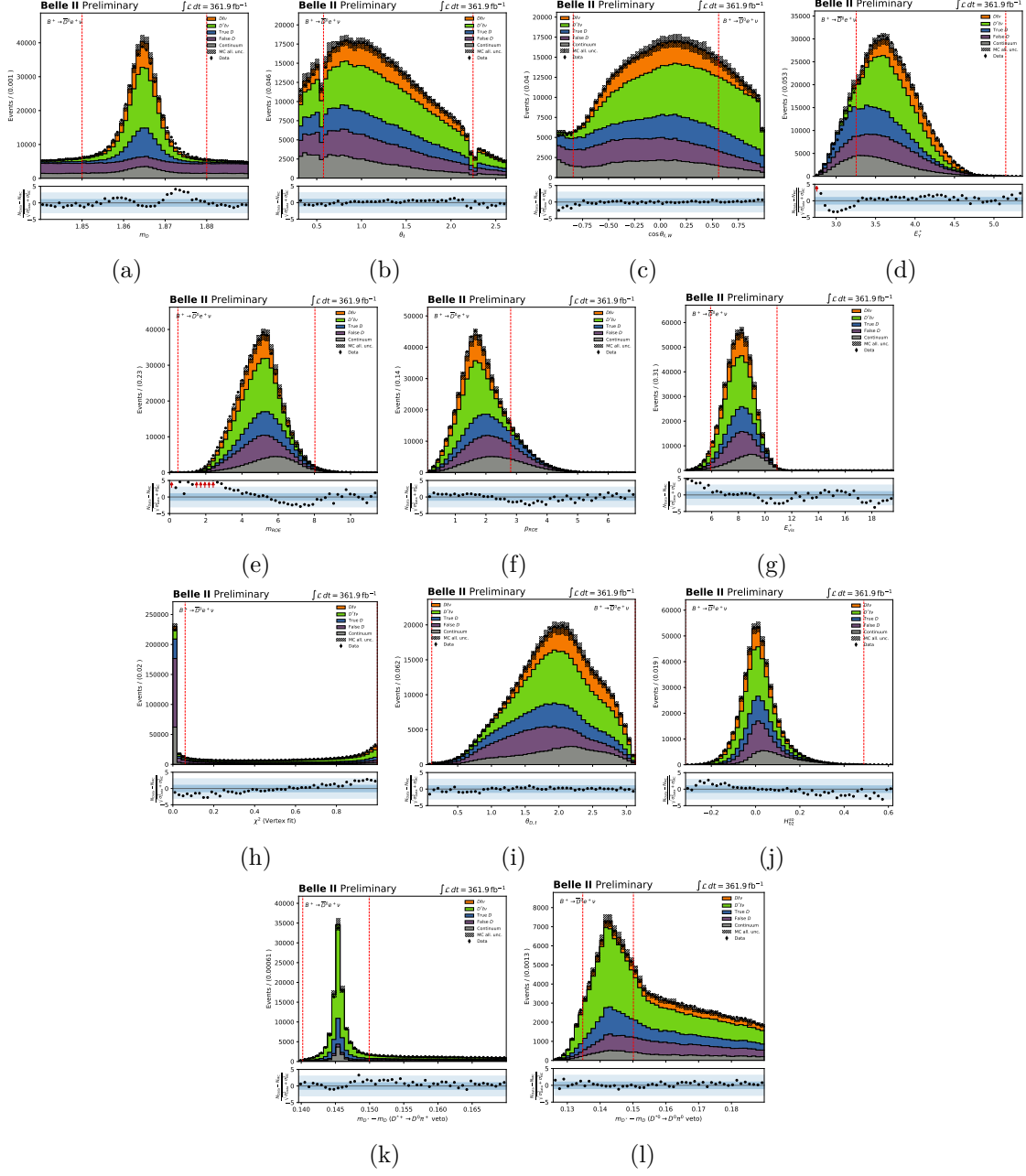
Figure C.1: All selections applied except the one shown in the plot for the B^+ \rightarrow \bar{D}^0 e^+ \nu_e mode.
