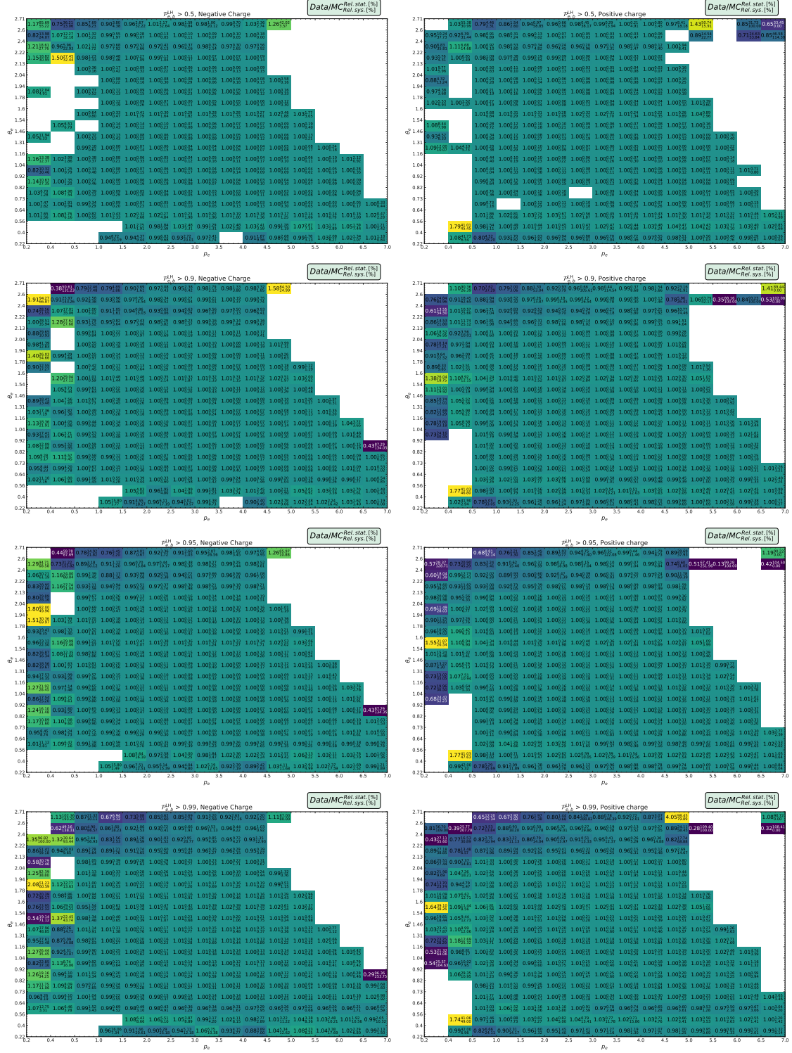
Figure A.4: Correction factors and uncertainties for likelihood-based binary electronID with different thresholds and charges.
