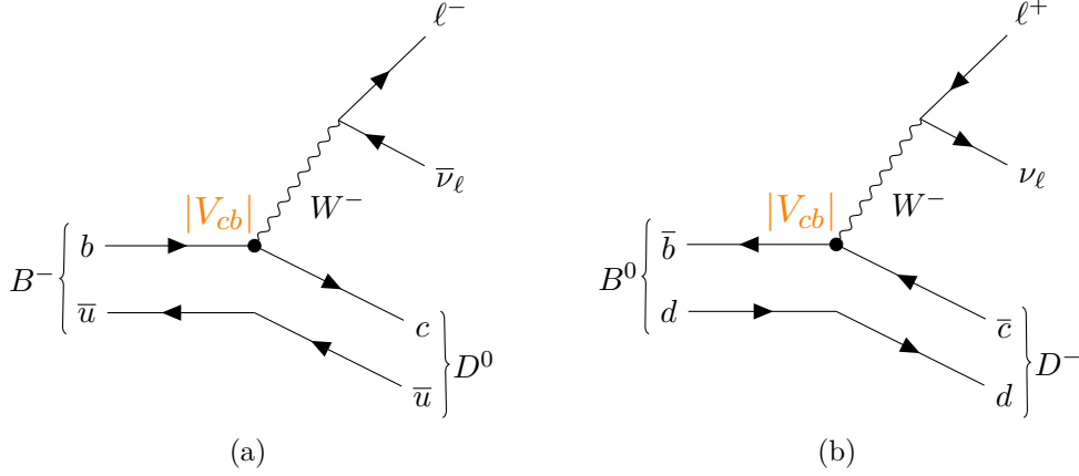
Figure 2.7: Feynman diagrams representing B^- \rightarrow D^0 \ell^- \bar{\nu}_\ell and B^0 \rightarrow D^- \ell^+ \nu_\ell decays.
