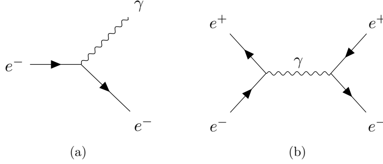
Figure 2.2: Feynman diagrams for electromagnetic interactions. Subfigure (a) depicts an electron that emits a photon in a process known as bremsstrahlung . Subfigure (b) shows e^+e^- \rightarrow e^+e^- scattering, also known as Bhabha scattering .
