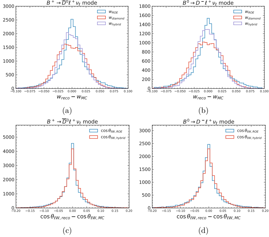
Figure 6.10: Resolutions for the kinematic variables w and \cos \theta_{\ell,W} . We compare approaches of ROE information only, diamond frame, and a combination of both. The combination results in the lowest width of the distributions. e and \mu channels are combined for each B mode.
