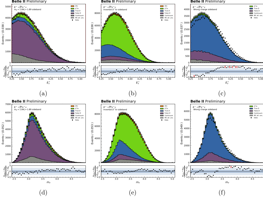
Figure 6.16: Data-MC agreements for the variables E_Y^* and m_Y in the control samples for the B^+ \rightarrow \bar{D}^0 e^+ \nu_e mode.
