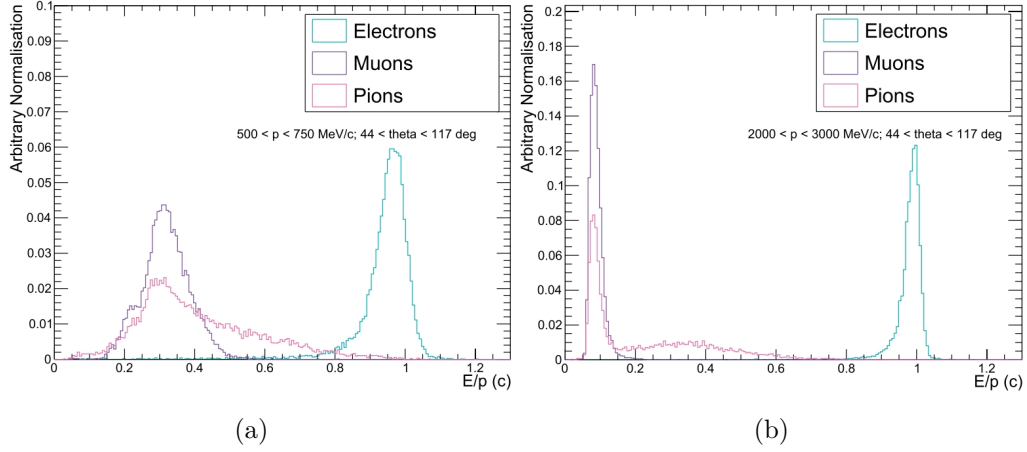
Figure 3.8: The histograms show the E/p distributions in the polar angle range 44^\circ < \theta < 117^\circ in the two momentum ranges (a) 500 < p < 750 MeV and (b) 2000 < p < 3000 MeV. E/p offers good discriminating power between electrons and pions/muons. [52]
