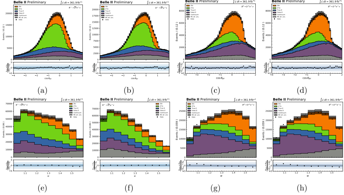
Figure 6.21: \cos \theta_{BY} and w distributions in data and MC for all four modes.
