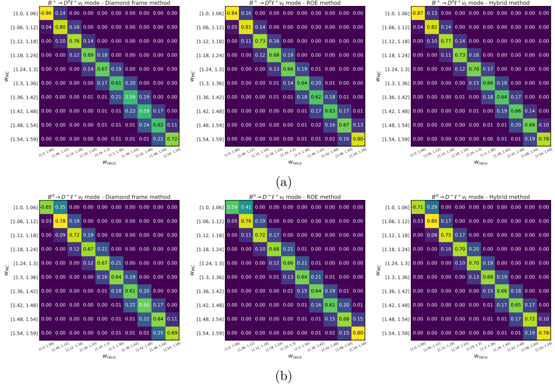
Figure 6.11: Migration matrices with each reconstruction approach for the charged and neutral B modes. The bin entries list the fraction of events reconstructed in each bin relative to their true origin.
