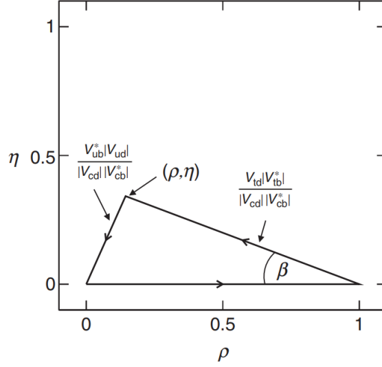
Figure 2.4: The unitarity triangle arising from the equation V_{ud}V_{ub}^* + V_{cd}V_{cb}^* + V_{td}V_{tb}^* = 0 [13].
