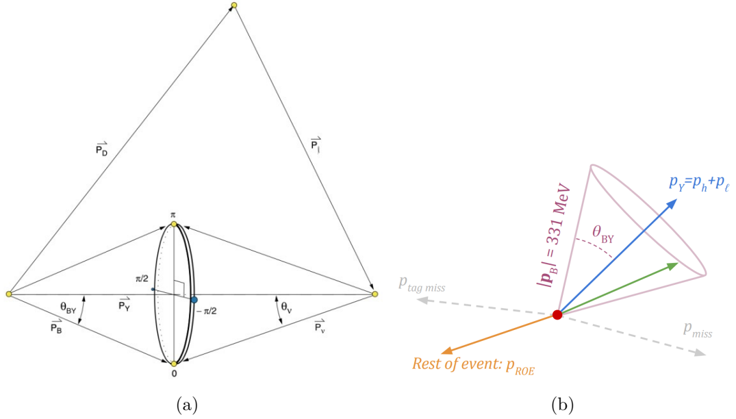
Figure 6.9: (a) Schematic of the diamond frame method, averaging over four directions. (b) Schematic of the ROE method, placing the B meson direction back-to-back with the p_{ROE} .
