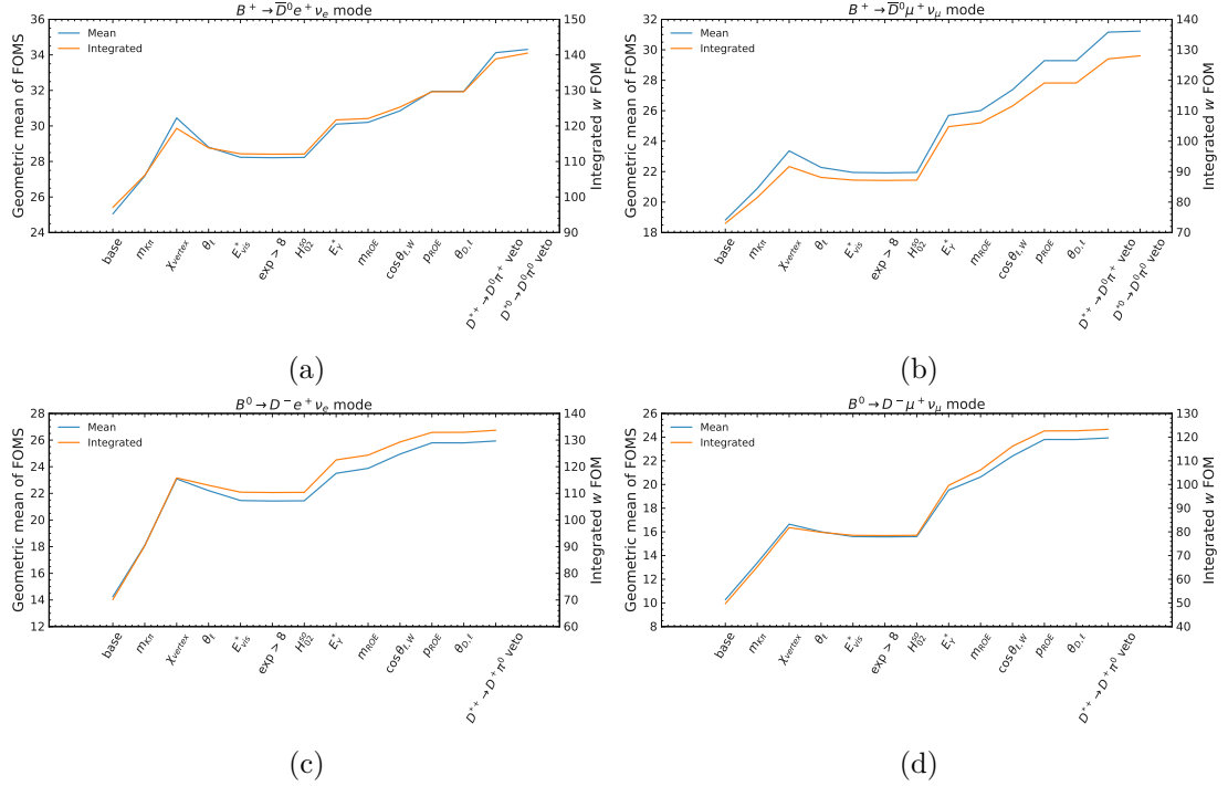
Figure 6.7: The figure of merit after each cut for all four modes, integrated over the full w range, is shown. The overall figure of merit for the entire sample and the geometric mean of the FOMs in each w bin, which serves as the target in the selected annealing, are displayed. Cuts not shown on the x axis but described in the text have already been applied in the steering file.
