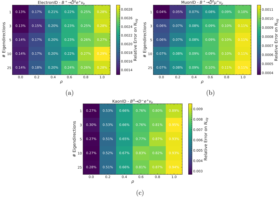
Figure 6.25: The uncertainty from particleID on the total signal yield N_{sig} as a function of assumed correlation coefficient \rho between systematic uncertainties bins in the correction tables, and a truncation order of the eigendecomposition that models the uncertainty. Full correlation \rho = 1 shows the largest uncertainty for all particles.
