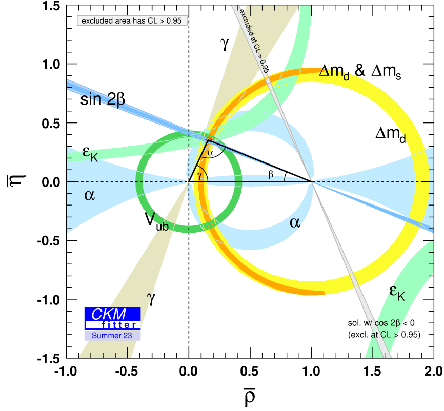
Figure 2.5: Experimental constraints on the unitarity triangle in the \rho - \eta plane [31]. The red hashed region around the top vertex of the triangle indicates the 68% confidence interval of the global combination.
