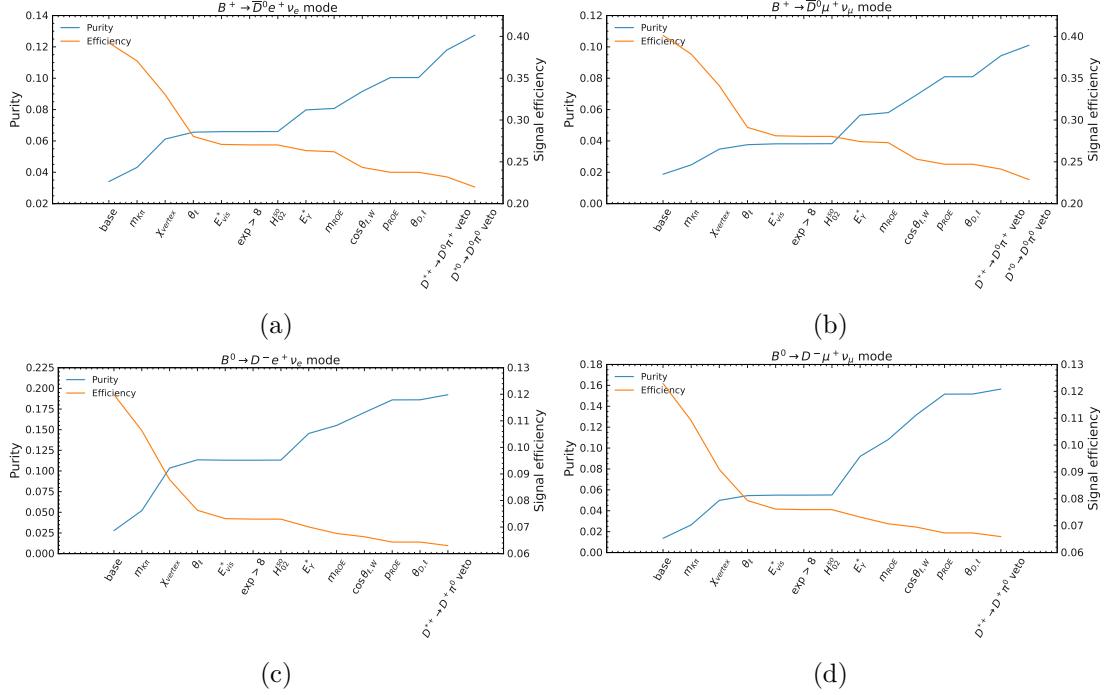
Figure 6.8: Purities and efficiencies after each cut for all four modes, integrated over the full w range.
