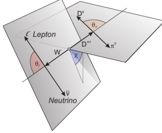
Figure 6.4: The differential decay rate of B \rightarrow D^*\ell\nu_\ell decays depends on the hadronic recoil w and the three angles \theta_\ell , \theta_V , and \chi , defined as shown in the figure.
