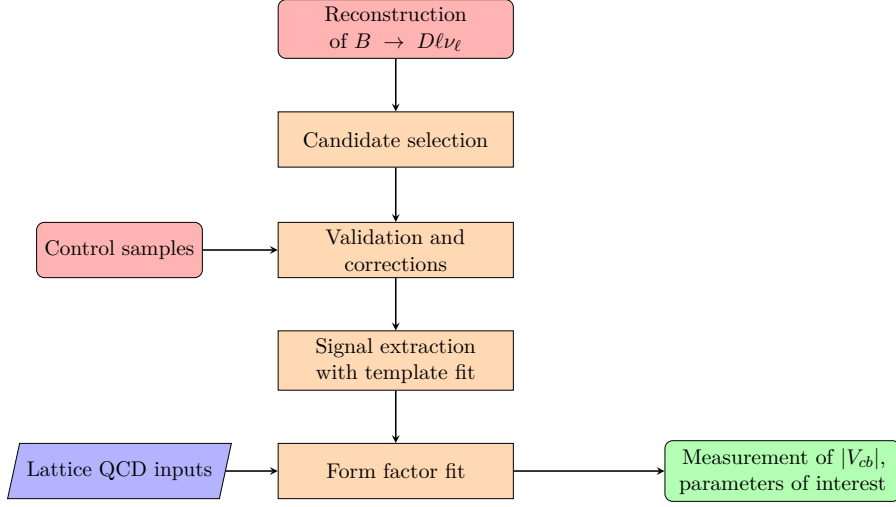
Figure 6.1: A schematic overview of the steps involved in the measurement. After reconstructing B \rightarrow D\ell\nu_\ell events in different final states in collision data, selection criteria are defined for optimal sensitivity. The modelling of signal and backgrounds is validated using control samples. Corrections are derived from control samples or external inputs to account for known and observed effects. Signal yields are extracted using a template fit, and the resulting differential decay rates are fit separately to the form factor. Using inputs from Lattice QCD in the form factor, |V_{cb}| and additional parameters of interest are accessible.
