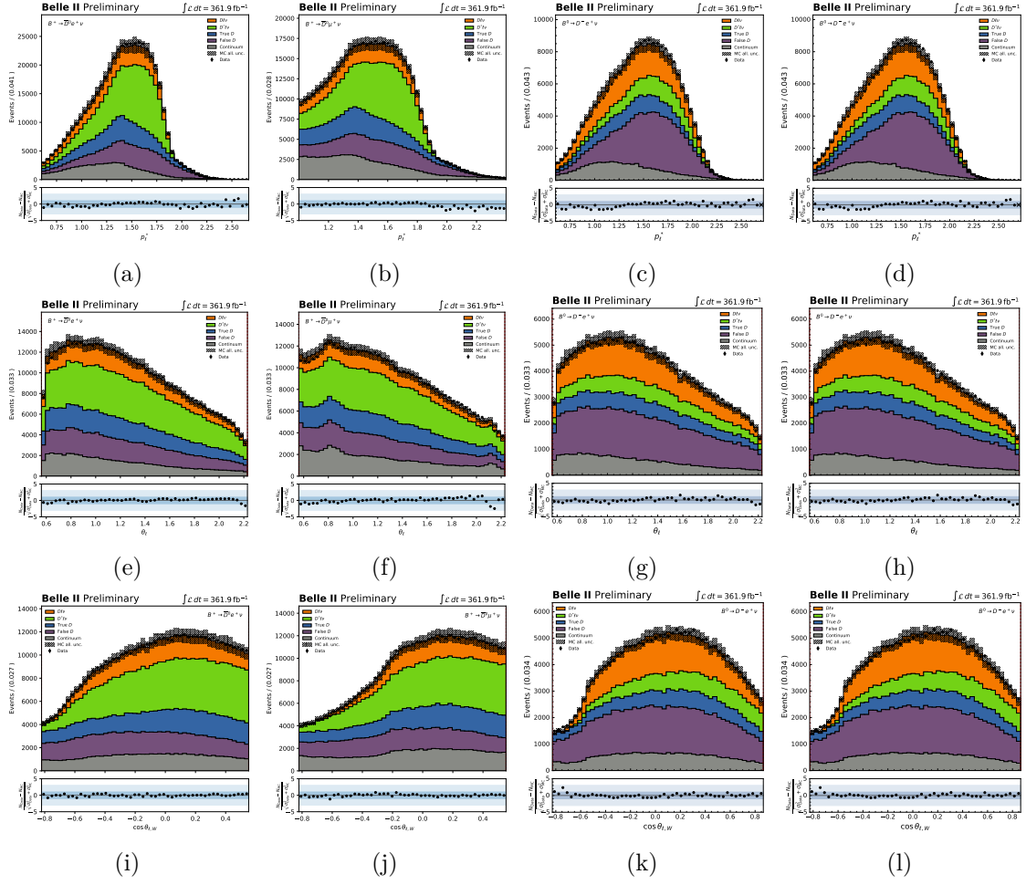
Figure 6.22: p_\ell^* , \theta_\ell and \cos\theta_{\ell,W} distributions in data and MC for all four modes.
