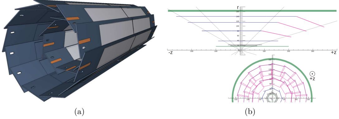
Figure 3.5: (a) Schematic overview of the PXD sensors and their geometric alignment. The DEPFET sensors are shown in light-grey areas [54]. (b) Geometrical alignment of the silicon strips in the SVD. The slanted layout in the forward region reduces the amount of required sensors [54].
