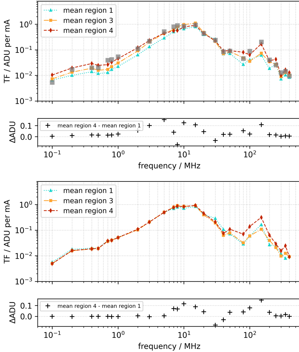
Figure 6.17.: Comparison of transfer functions of the three matrix regions before and after the change in the CDN for otherwise same measurement parameters. The noise was injected into the dgnd, dcd-dvdd, dhp-core, dhp-io and sw-dvdd lines. Before the change (top) there is a spread between the regions below about 10 MHz which is no longer present after the modification (bottom). The gray squares in the plot of the first measurement indicate the mean over all channels from the repeated measurement as references.
