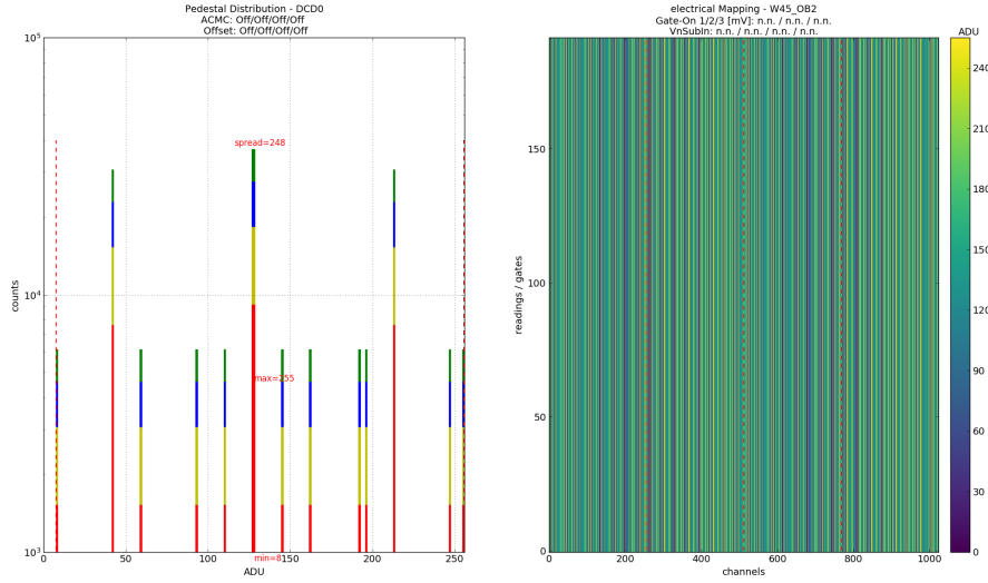
Figure 7.22.: DCD test pattern for data transmission verification. Left: Histogram of pre-defined ADU values. Right: Representation in electrical format. A constant value is assigned to each ADC, hence constant values are displayed along the vertical axis.
