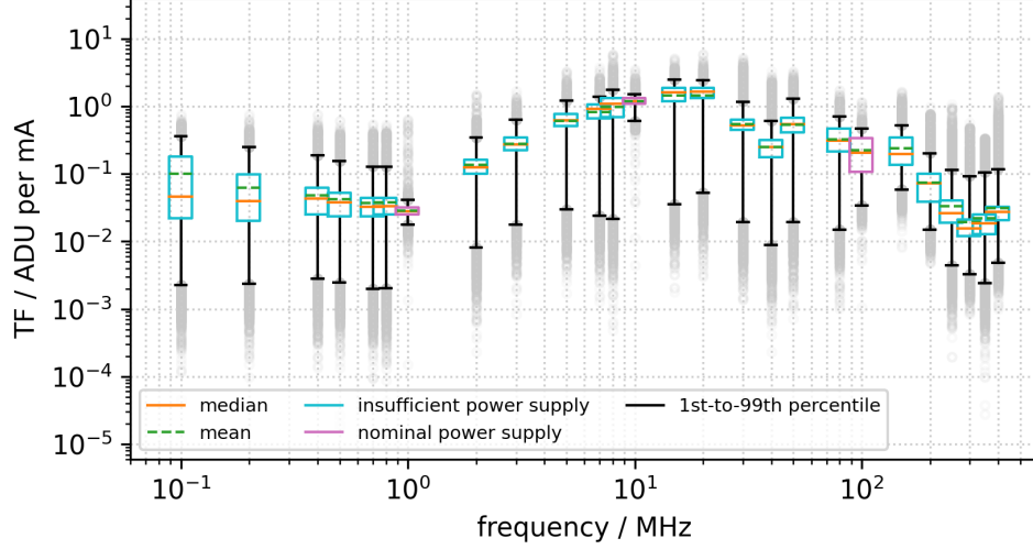
Figure 6.19.: Transfer function for conducted differential-mode noise injected into the gate-on1 line. A total number of 88 060 channels entered in this analysis. While most data points were recorded during insufficient power supply conditions for the DCDs (cyan), three data points were replaced with values from the reference measurement taken with nominal power supply (magenta).
