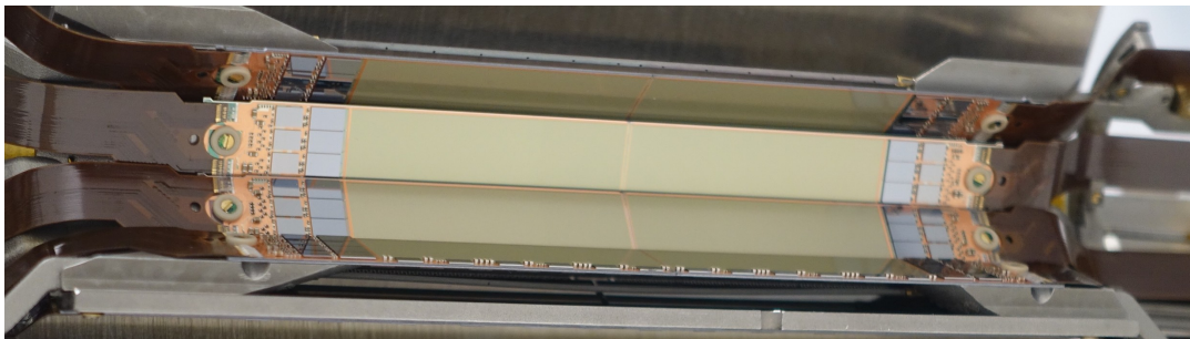
Figure 8.8.: Half-shell HS-1p3 from inside after ladder assembly [105]. The top side of the modules with the ASICs is facing the beam pipe. The windmill structure allows a complete coverage in \phi . The gap between the sensitive areas of glued modules is about 850\mu\text{m} (glue joint and supporting silicon frame). The position of the gap in the outer layer is shifted relative to the one in the inner layer to optimize the coverage.
