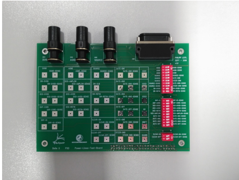
Figure 5.9.: Power Lines Test Board. At the upper right side the Glenair cable has to be connected. The three banana connectors provide the reference voltages for the different domains: dgnd, agnd and source. The test pads feature a large contact area and are clearly labeled simplifying the task of voltage verification. The DIP switches on the right side can be used to close or open the connections between force and sense lines.
