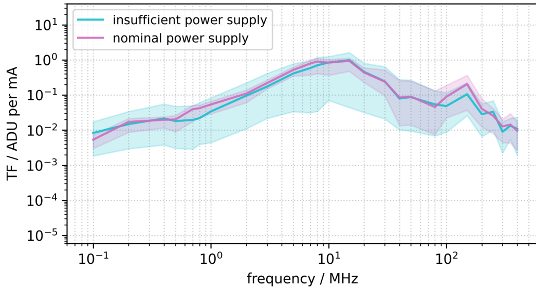
Figure 6.16.: Comparison of calculated transfer functions before and after the change in the CDN for the same measurement settings. The noise was injected into d gnd , dcd-dvdd, dhp-core, dhp-io and sw-dvdd lines. After the change in the CDN this measurement was repeated with otherwise same settings. The 5-to-95-percentile-band around the mean curve reduces largely for frequencies below 40 MHz. The calculated mean curves show good agreement between the two measurements.
