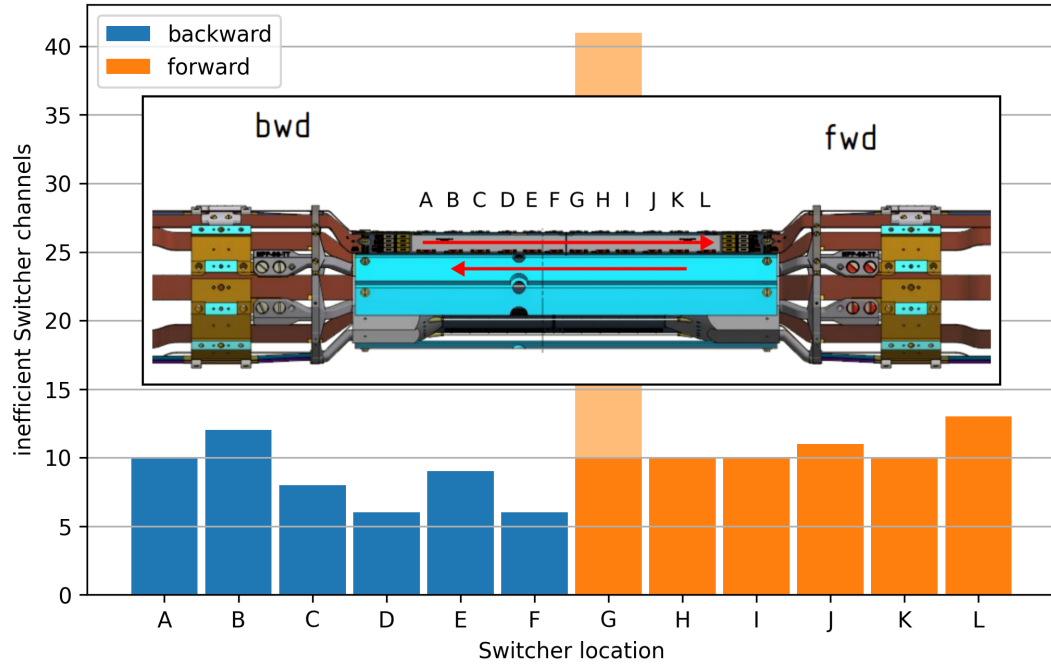
Figure 9.30.: Histogram of inefficient gates per Switcher location. In the forward modules 13 more dead gates are found compared to the backward modules representing a clear effect of 25 %. Whereas a slight preference for the outer locations can only be suspected. The assignment to the Switcher locations has to consider the four different layouts of the PXD modules and the different read-out directions between the two layers (indicated by red arrows). For simplicity it is assumed that the corresponding Switcher locations of inner and outer modules are identical in z. After the incident in experiment 18 the entire last Switcher of module 1.03.1 was affected. Therefore, module 1.03.1 alone contributes with 32 inefficient gates to Switcher location G (indicated by a lighter color).
