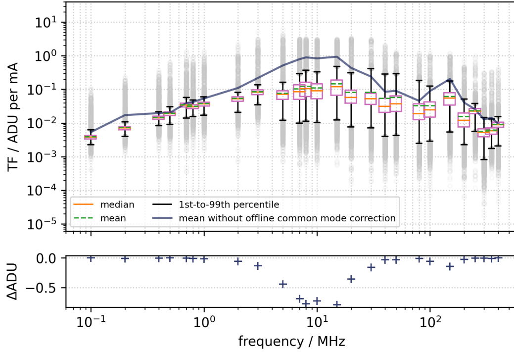
Figure 6.34.: Effect of offline digital common mode correction on susceptibility to external noise injection. The mean values of the actual measurement are plotted as dark line for reference. The response of all pixels was processed by the offline common mode correction and the resulting values entered as box plot. The data from the measurement after the change in the CDN was used. The noise was injected into d gnd , d cd -dv dd , d hp -core, d hp -io and sw-dv dd lines.
