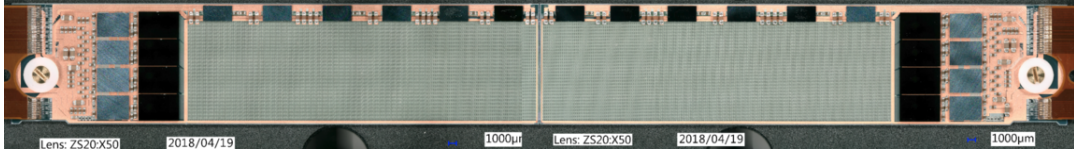
Figure 8.2.: Ladder L1_028 after gluing of backward module W03_IB and forward module W02_IF [184]. The ladder is fixed with a PEEK washer and a screw with specified torque on both sides.
