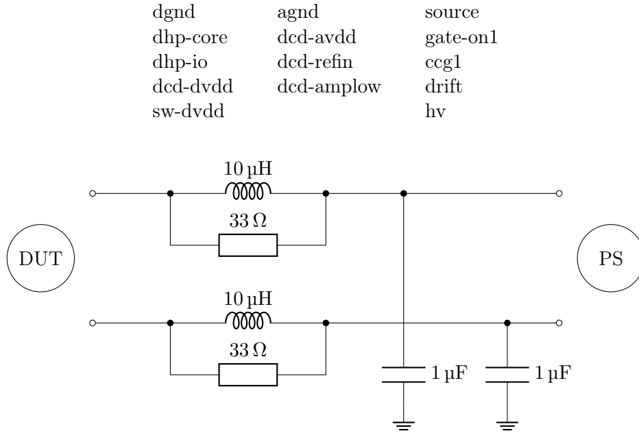
Figure 6.7.: Schematic sketch of the Coupling Decoupling Network (CDN). Two exemplary lines are drawn as an illustration. All of the 14 connected lines were handled in the same way.
