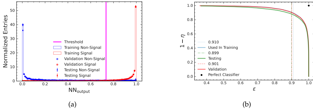
FIGURE F.4: Classifying model for the channel B^+ \rightarrow K^{*+}(\rightarrow K_S^0 \pi^+) ee . Both plots contain the three datasets that are used during training, validation and testing. In (a) the binary classifying output of the model and in (b) the ROC is shown. In (b) the vertical lines indicate the relative efficiency of the network which produces the closest point in the ROC curve to the perfect classifier at (1,1). The position of these lines, which also represents the relative efficiency of the classifier, is stated in the legend.
