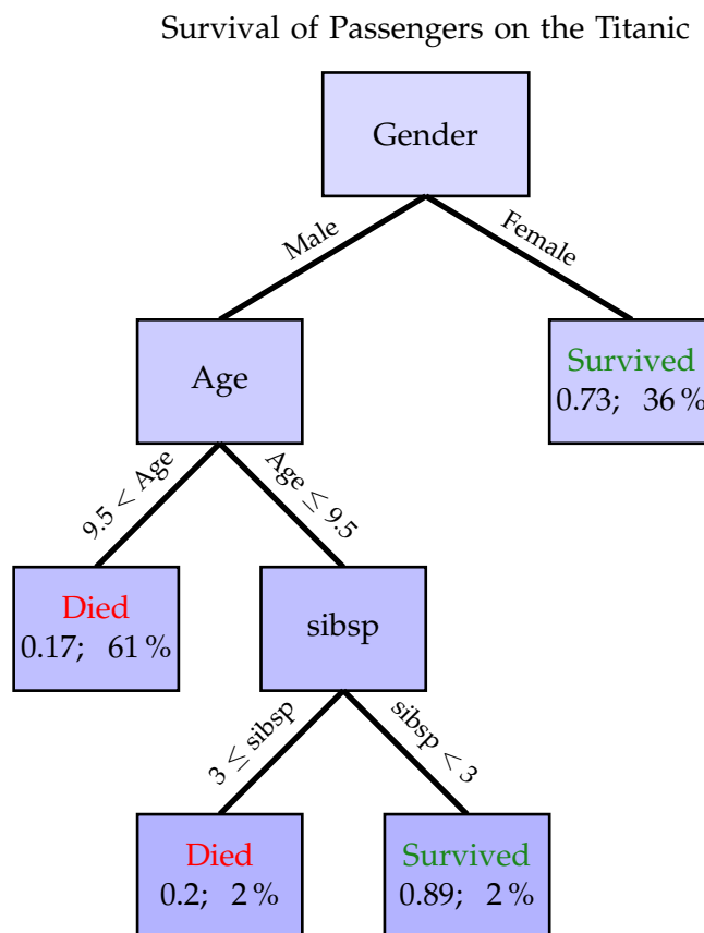
FIGURE 5.12: Example for a structure of a decision tree with a tree depth of three. The probability to survive the Titanic accident will be determined based on the features gender, age and how many siblings and spouses (sibsp) are on board. The numbers in each box (leaf) show the probability of survival (left number) and the percentage of the total data sample (right number). For example, 36% of all people on board were female and each of them had a 73% chance of survival according to the decision tree [84]. If the probability of survival is higher than 50 % the leaf is labeled Survived , otherwise Died .
