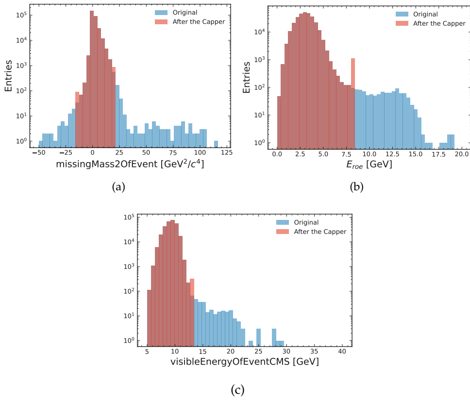
FIGURE E.1: The result of using the capper on the features missing-Mass2OfEvent (a), energy of the rest of event (b) and visibleEnergy-OfEventCMS (c). The few outliers are moved closer to the rest of the values.
