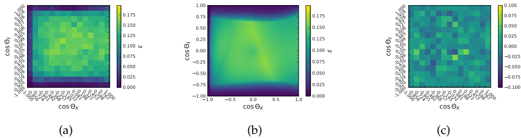
FIGURE G.40: (a) Input efficiencies for the acceptance model training. Resulting acceptance correction model for the decay B^+ \rightarrow K^{*+}(\rightarrow K_S^0 \pi^+) ee in the q_1^2 region. In (b) the resulting model function is shown. In (c) the difference between the predicted and true efficiency is shown.
