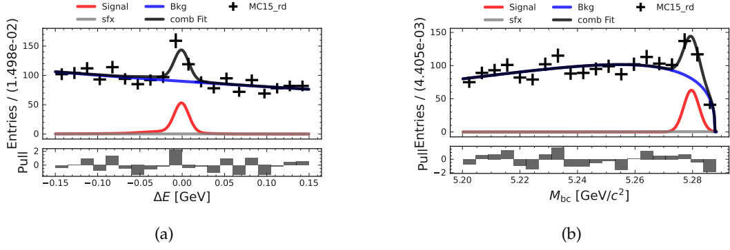
FIGURE I.15: M_{bc} and \Delta E fits in the q_1^2 -region for the B^0 \rightarrow K^{*0}(\rightarrow K^+\pi^-)\ell\ell channel with the MC15_rd dataset.
