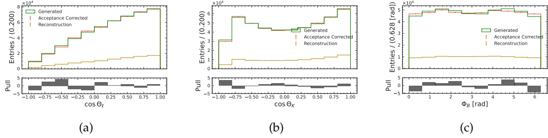
FIGURE G.53: Decay angle acceptance correction for \cos \theta_\ell (a), \cos \theta_K (b) and \Phi_B (c) for the B^0 \rightarrow K^{*0}(\rightarrow K^+\pi^-)ee channel in the q_3^2 -region. Green shows the distribution on generator level. The reconstructed candidates are shown in dark orange. They are corrected with the acceptance correction and the result is shown in red.
