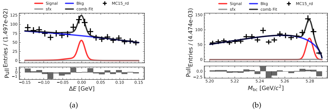
FIGURE I.16: M_{bc} and \Delta E fits in the q_2^2 -region for the B^0 \rightarrow K^{*0}(\rightarrow K^+\pi^-)\ell\ell channel with the MC15_rd dataset.
