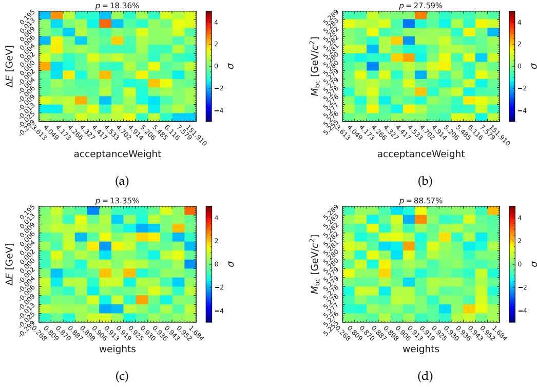
FIGURE H.16: Correlations between the \Delta E/M_{bc} and acceptance and PID weights in the B^0 \rightarrow K^{*0}(\rightarrow K^+ \pi^-) \mu \mu for signal events.
