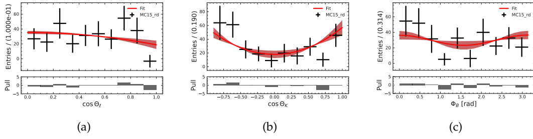
FIGURE I.39: Angular fit projections for the B^0 \rightarrow K^{*0}(\rightarrow K^+\pi^-)\ell\ell channel in the q_3^2 -region with the MC15_rd dataset.
