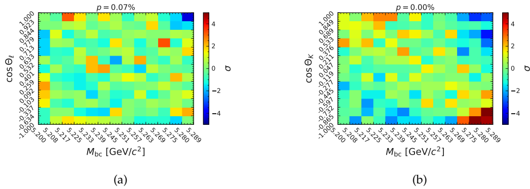
FIGURE 7.18: Correlation between M_{bc} and \cos\theta_\ell and \cos\theta_K in the B^+ \rightarrow K^{*+}(\rightarrow K^+\pi^0)ee channel for background events. A rather strong correlation can be observed between M_{bc} and \cos\theta_\ell . Due to this correlation, this channel can no longer be analyzed with the sWeights method.
