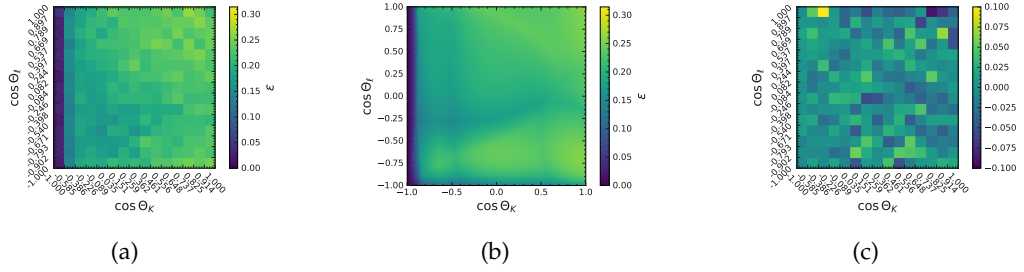
FIGURE G.30: (a) Input efficiencies for the acceptance model training. Resulting acceptance correction model for the decay B^0 \rightarrow K^{*0}(\rightarrow K^+ \pi^-)ee in the q_3^2 region. In (b) the resulting model function is shown. In (c) the difference between the predicted and true efficiency is shown.
