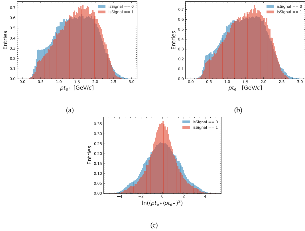
FIGURE E.3: Transverse momenta of the leptons are shown in (a) and (b). Ratio of the transverse momenta of both reconstructed leptons is shown in (c).
