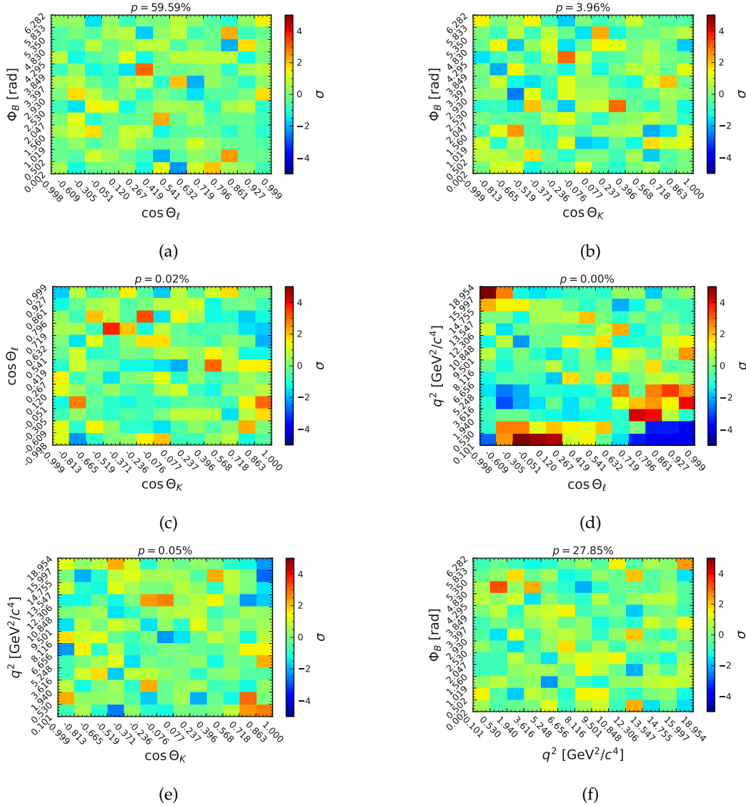
FIGURE 7.12: Correlations between four decay variables for the B^0 \rightarrow K^{*0}(\rightarrow K^+\pi^-)ee . There is a correlation between \cos \theta_\ell and q^2 . However, this correlation is expected since both of these variables depend on both leptons in the decay.
