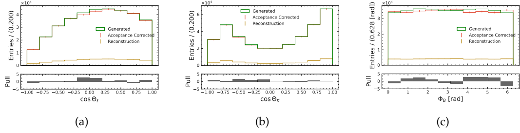
FIGURE G.64: Decay angle acceptance correction for \cos \theta_\ell (a), \cos \theta_K (b) and \Phi_B (c) for the B^+ \rightarrow K^{*+}(\rightarrow K_S^0 \pi^+) ee channel in the q_2^2 -region. Green shows the distribution on generator level. The reconstructed candidates are shown in dark orange. They are corrected with the acceptance correction and the result is shown in red.
