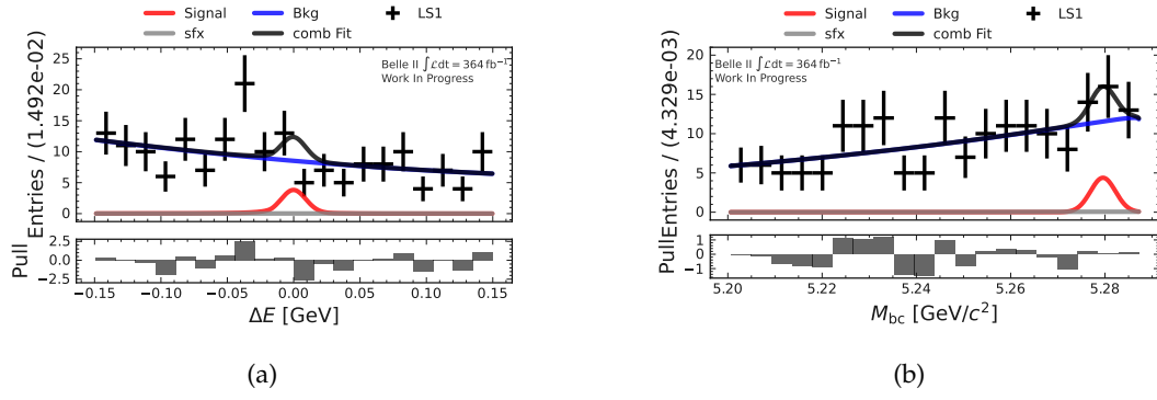
FIGURE I.51: M_{bc} and \Delta E fits in the q_3^2 -region for the B^0 \rightarrow K^{*0}(\rightarrow K^+\pi^-)\mu\mu channel with the LS1 dataset.
