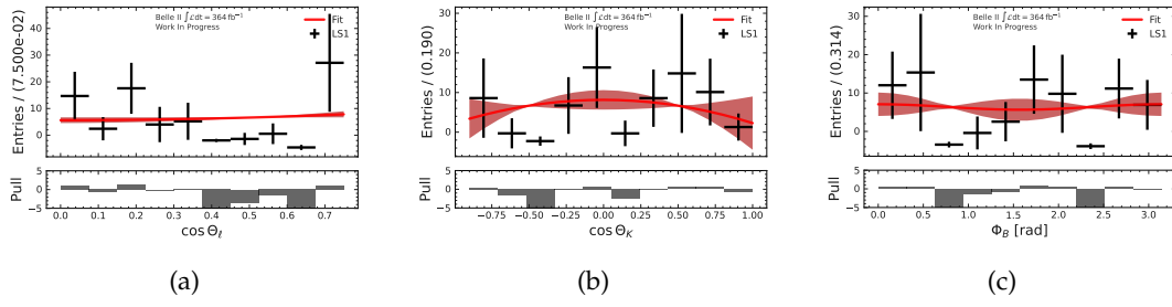
FIGURE I.65: Angular fit projections for the B^0 \rightarrow K^{*0}(\rightarrow K^+\pi^-)\ell\ell channel in the q_1^2 -region with the LS1 dataset.
