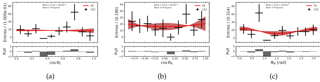
FIGURE I.66: Angular fit projections for the B^0 \rightarrow K^{*0}(\rightarrow K^+\pi^-)\ell\ell channel in the q_2^2 -region with the LS1 dataset.
