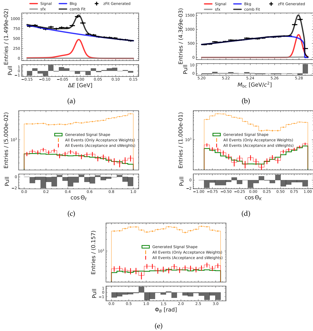
FIGURE 9.1: Showing the effect of the sWeights using toy MC. (a) and (b) show the discriminating variables, (c), (d) and (e) the target variables. The generated signal events are shown in green, the dataset containing signal and non-signal events in dark orange (only acceptance weights are applied) and red (acceptance and sWeights are applied). The amount of events corresponds to an integrated luminosity of \int \mathcal{L} dt = 50 \text{ ab}^{-1} .
