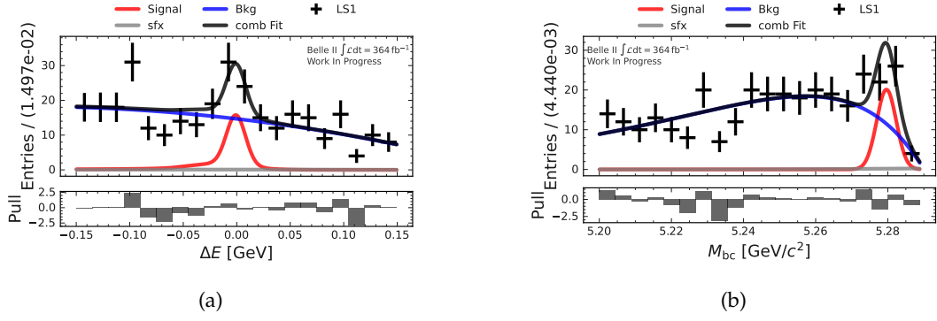
FIGURE I.54: M_{bc} and \Delta E fits in the q_2^2 -region for the B^0 \rightarrow K^{*0}(\rightarrow K^+\pi^-)\ell\ell channel with the LS1 dataset.
