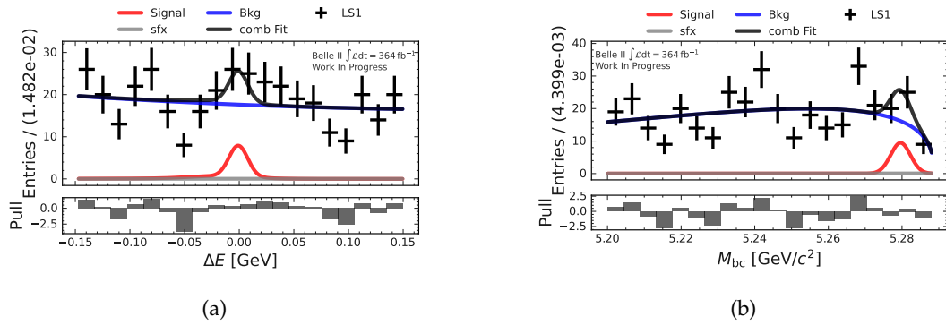
FIGURE I.53: M_{bc} and \Delta E fits in the q_1^2 -region for the B^0 \rightarrow K^{*0}(\rightarrow K^+\pi^-)\ell\ell channel with the LS1 dataset.
