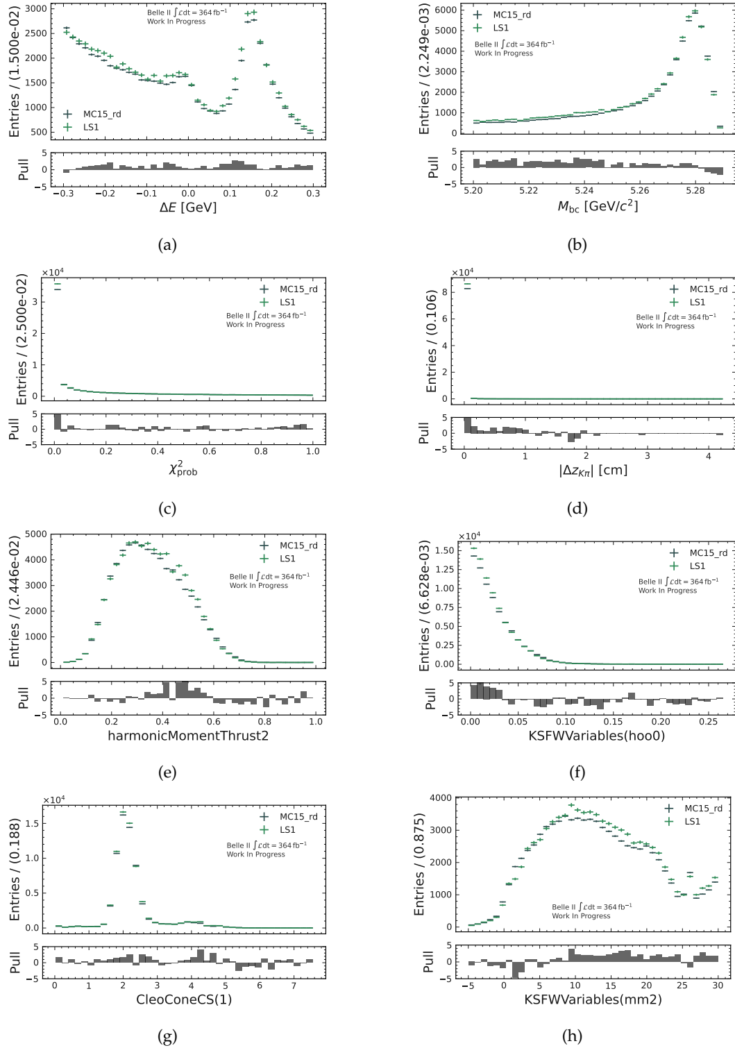
FIGURE D.6: Comparison between LS1 data and MC15_rd for the decay channel B^+ \rightarrow K^{*+}(\rightarrow K^+ \pi^0) ee . (a) and (b) show the discriminating variables \Delta E and M_{bc} , respectively. (c) - (h) show the comparison for the six most important features for classification of this decay channel.
