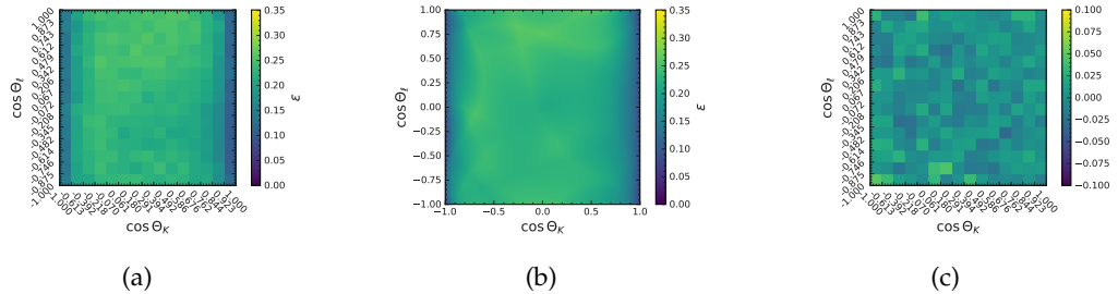
FIGURE G.37: (a) Input efficiencies for the acceptance model training. Resulting acceptance correction model for the decay B^0 \rightarrow K^{*0}(\rightarrow K^+\pi^-)\mu\mu in the q_4^2 region. In (b) the resulting model function is shown. In (c) the difference between the predicted and true efficiency is shown.
