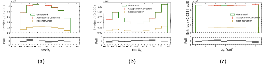
FIGURE G.52: Decay angle acceptance correction for \cos \theta_\ell (a), \cos \theta_K (b) and \Phi_B (c) for the B^0 \rightarrow K^{*0}(\rightarrow K^+\pi^-)ee channel in the q_1^2 -region. Green shows the distribution on generator level. The reconstructed candidates are shown in dark orange. They are corrected with the acceptance correction and the result is shown in red.
