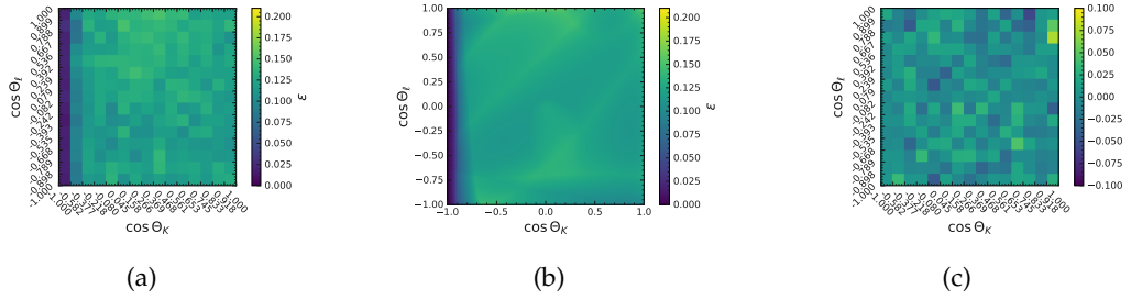
FIGURE G.48: (a) Input efficiencies for the acceptance model training. Resulting acceptance correction model for the decay B^+ \rightarrow K^{*+}(\rightarrow K_S^0 \pi^+) \mu \mu in the q_3^2 region. In (b) the resulting model function is shown. In (c) the difference between the predicted and true efficiency is shown.
