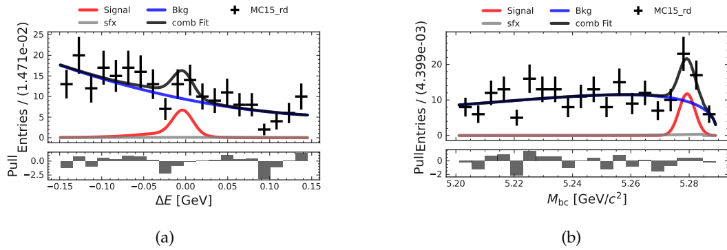
FIGURE I.8: M_{bc} and \Delta E fits in the q_2^2 -region for the B^+ \rightarrow K^{*+}(\rightarrow K_S^0 \pi^+) ee channel with the MC15_rd dataset.
