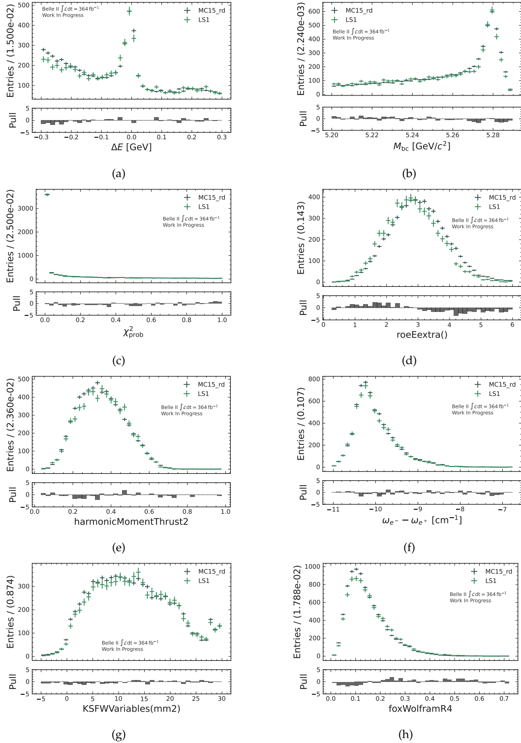
FIGURE D.4: Comparison between LS1 data and MC15_rd for the decay channel B^+ \rightarrow K^{*+}(\rightarrow K_S^0 \pi^+) ee . (a) and (b) show the discriminating variables \Delta E and M_{bc} , respectively. (c) - (h) show the comparison for the six most important features for classification of this decay channel.
