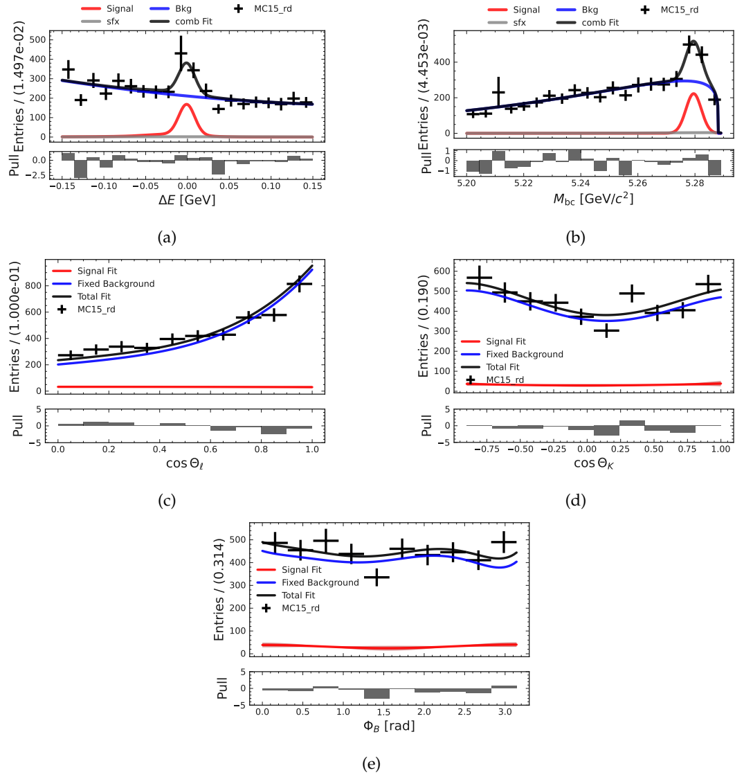
FIGURE J.13: Figures related to the fit study with fixed background shapes and no sWeights for the B^0 \rightarrow K^{*0}(\rightarrow K^+\pi^-)\ell\ell in the q_3^2 -region.
