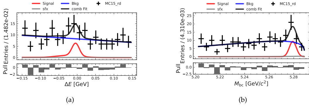
FIGURE I.7: M_{bc} and \Delta E fits in the q_1^2 -region for the B^+ \rightarrow K^{*+}(\rightarrow K_S^0 \pi^+) ee channel with the MC15_rd dataset.
