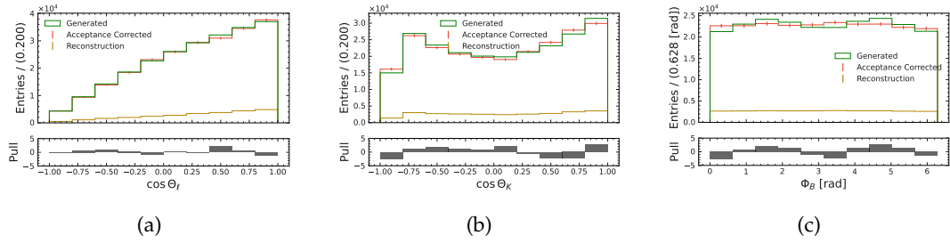
FIGURE G.65: Decay angle acceptance correction for \cos \theta_\ell (a), \cos \theta_K (b) and \Phi_B (c) for the B^+ \rightarrow K^{*+}(\rightarrow K_S^0 \pi^+) ee channel in the q_3^2 -region. Green shows the distribution on generator level. The reconstructed candidates are shown in dark orange. They are corrected with the acceptance correction and the result is shown in red.
