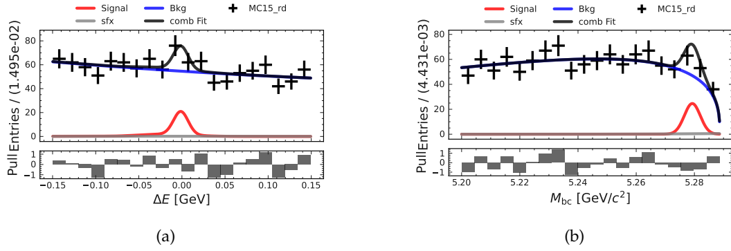
FIGURE I.19: M_{bc} and \Delta E fits in the q_1^2 -region for the B^+ \rightarrow K^{*+}(\rightarrow K_S^0 \pi^+) \ell \ell channel with the MC15_rd dataset.
