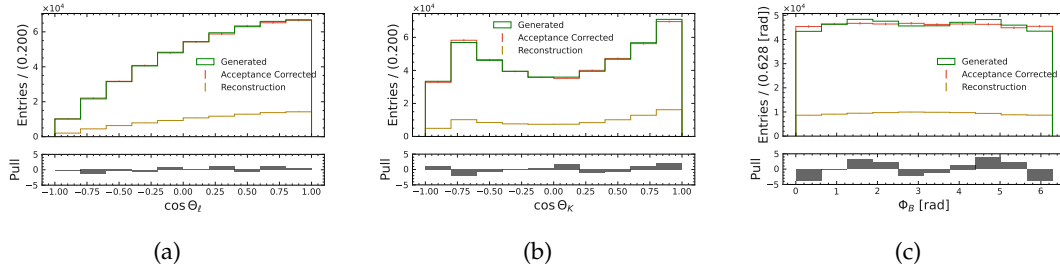
FIGURE G.55: Decay angle acceptance correction for \cos \theta_\ell (a), \cos \theta_K (b) and \phi_B (c) for the B^0 \rightarrow K^{*0}(\rightarrow K^+\pi^-)ee channel in the q_{l/\psi}^2 -region. Green shows the distribution on generator level. The reconstructed candidates are shown in dark orange. They are corrected with the acceptance correction and the result is shown in red.
