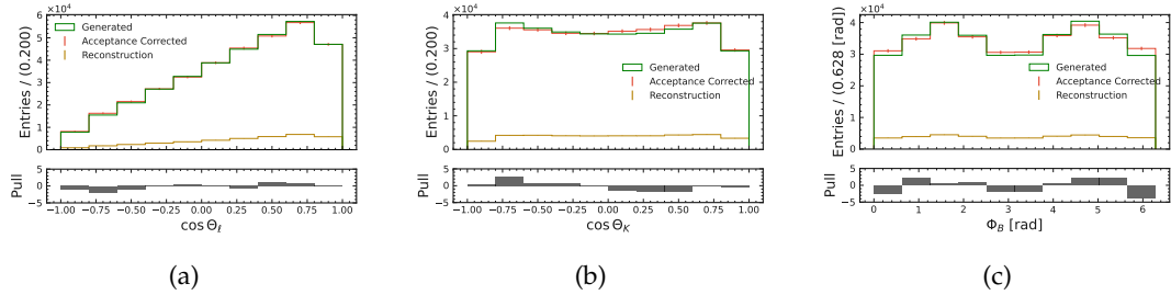
FIGURE G.66: Decay angle acceptance correction for \cos \theta_\ell (a), \cos \theta_K (b) and \Phi_B (c) for the B^+ \rightarrow K^{*+}(\rightarrow K_S^0 \pi^+) ee channel in the q_4^2 -region. Green shows the distribution on generator level. The reconstructed candidates are shown in dark orange. They are corrected with the acceptance correction and the result is shown in red.
