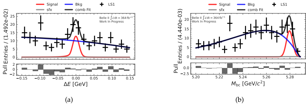
FIGURE I.50: M_{bc} and \Delta E fits in the q_2^2 -region for the B^0 \rightarrow K^{*0}(\rightarrow K^+ \pi^-) \mu\mu channel with the LS1 dataset.
