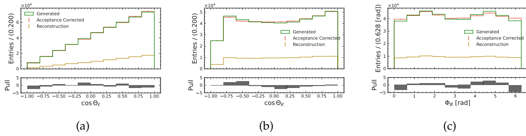
FIGURE G.62: Decay angle acceptance correction for \cos \theta_\ell (a), \cos \theta_K (b) and \phi_B (c) for the B^0 \rightarrow K^{*0}(\rightarrow K^+\pi^-)\mu\mu channel in the q_{\psi(2S)}^2 -region. Green shows the distribution on generator level. The reconstructed candidates are shown in dark orange. They are corrected with the acceptance correction and the result is shown in red.
