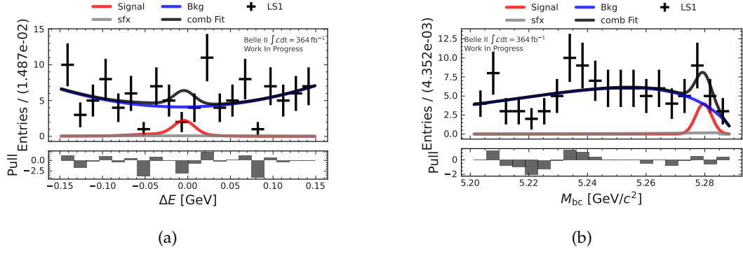
FIGURE I.48: M_{bc} and \Delta E fits in the q_4^2 -region for the B^0 \rightarrow K^{*0}(\rightarrow K^+ \pi^-) ee channel with the LS1 dataset.
