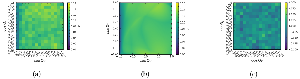
FIGURE G.49: (a) Input efficiencies for the acceptance model training. Resulting acceptance correction model for the decay B^+ \rightarrow K^{*+}(\rightarrow K_S^0 \pi^+) \mu \mu in the q_4^2 region. In (b) the resulting model function is shown. In (c) the difference between the predicted and true efficiency is shown.
