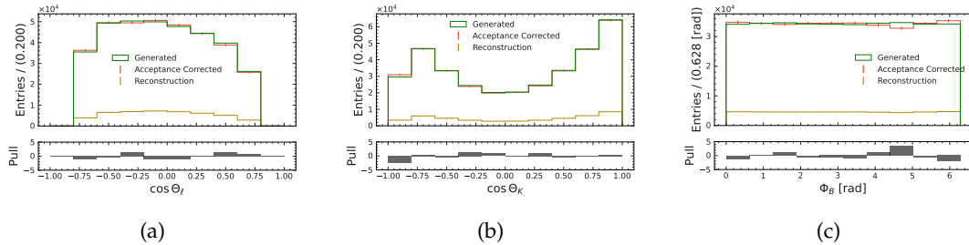
FIGURE G.63: Decay angle acceptance correction for \cos \theta_\ell (a), \cos \theta_K (b) and \phi_B (c) for the B^+ \rightarrow K^{*+}(\rightarrow K_S^0\pi^+)ee channel in the q_1^2 -region. Green shows the distribution on generator level. The reconstructed candidates are shown in dark orange. They are corrected with the acceptance correction and the result is shown in red.
