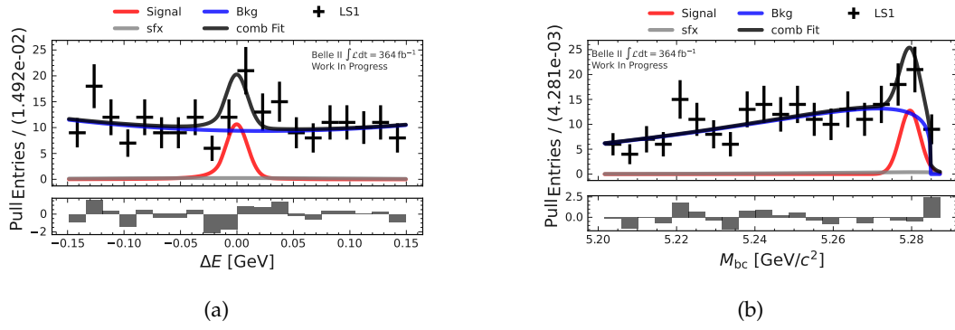
FIGURE I.52: M_{bc} and \Delta E fits in the q_4^2 -region for the B^0 \rightarrow K^{*0}(\rightarrow K^+\pi^-)\mu\mu channel with the LS1 dataset.
