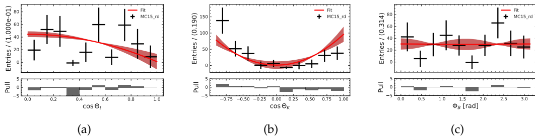
FIGURE I.42: Angular fit projections for the B^+ \rightarrow K^{*+}(\rightarrow K_S^0\pi^+)\ell\ell channel in the q_2^2 -region with the MC15_rd dataset.
