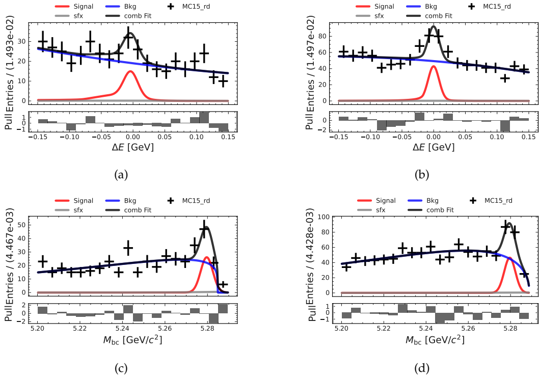
FIGURE 8.3: M_{bc} and \Delta E fits in the q_2^2 -region for the B^0 \rightarrow K^{*0}(\rightarrow K^+\pi^-)\ell\ell channel with the MC15_rd dataset. The fits for \ell = e ( \ell = \mu ) are shown on the left (right).
