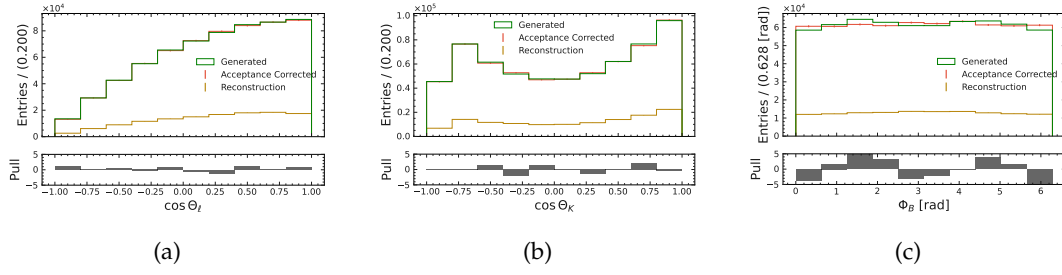
FIGURE G.61: Decay angle acceptance correction for \cos \theta_\ell (a), \cos \theta_K (b) and \phi_B (c) for the B^0 \rightarrow K^{*0}(\rightarrow K^+\pi^-)\mu\mu channel in the q_{l/\psi}^2 -region. Green shows the distribution on generator level. The reconstructed candidates are shown in dark orange. They are corrected with the acceptance correction and the result is shown in red.
