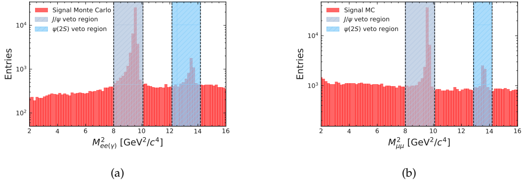
FIGURE 7.6: Depiction of the veto regions for the J/\psi and \psi(2S) in (a) for \ell\ell \triangleq ee and (b) for \ell\ell \triangleq \mu\mu . The \psi(2S) veto region is larger for the electrons due to their poorer energy resolution in the detector caused by bremsstrahlung photons.
