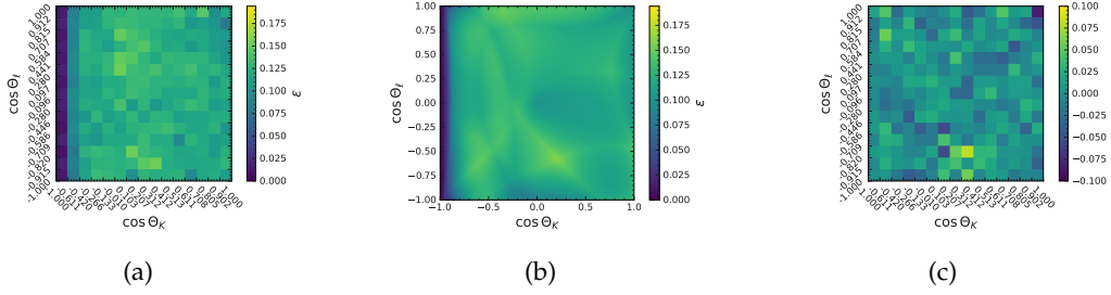
FIGURE G.50: (a) Input efficiencies for the acceptance model training. Resulting acceptance correction model for the decay B^+ \rightarrow K^{*+}(\rightarrow K_S^0 \pi^+) \mu \mu in the q_{J/\psi}^2 region. In (b) the resulting model function is shown. In (c) the difference between the predicted and true efficiency is shown.
