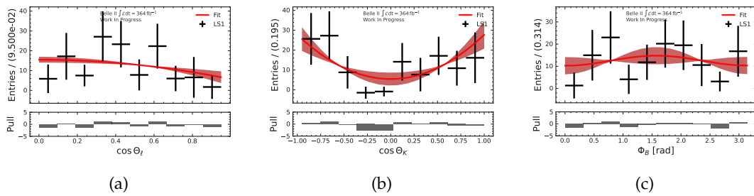
FIGURE I.68: Angular fit projections for the B^0 \rightarrow K^{*0}(\rightarrow K^+\pi^-)\ell\ell channel in the q_4^2 -region with the LS1 dataset.
