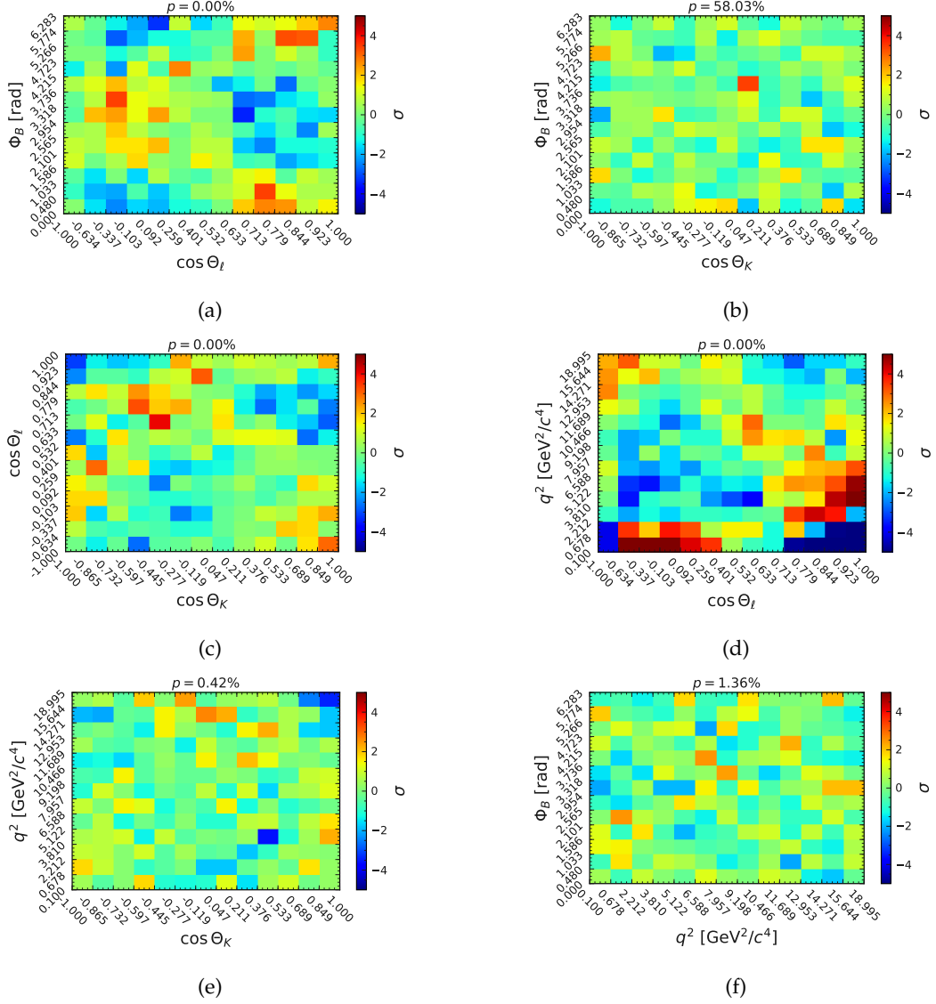
FIGURE G.4: Correlations Between the Four Decay Variables for the B^+ \rightarrow K^{*+}(\rightarrow K^+ \pi^0) e e . There is a correlation between \cos \Theta_\ell and q^2 . However, this correlation is expected since both of these variables depend on both leptons in the decay.
