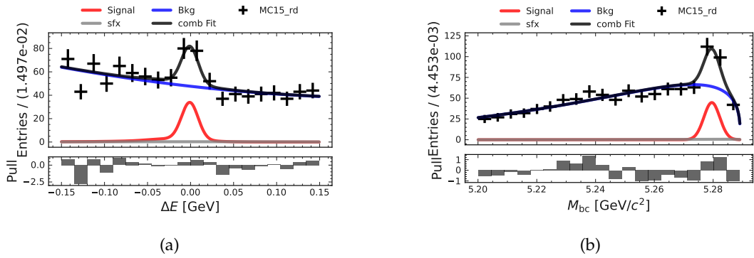
FIGURE I.17: M_{bc} and \Delta E fits in the q_3^2 -region for the B^0 \rightarrow K^{*0}(\rightarrow K^+\pi^-)\ell\ell channel with the MC15_rd dataset.
