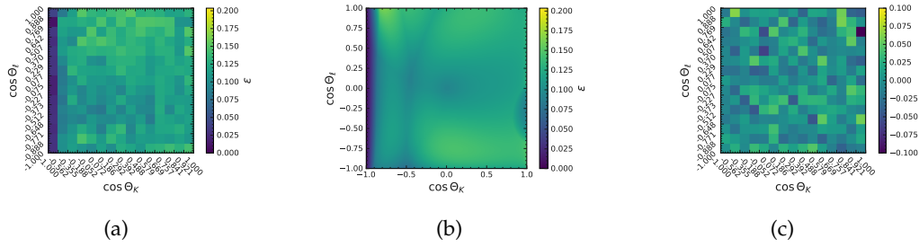
FIGURE G.45: (a) Input efficiencies for the acceptance model training. Resulting acceptance correction model for the decay B^+ \rightarrow K^{*+}(\rightarrow K_S^0 \pi^+) ee in the q_{\psi(2S)}^2 region. In (b) the resulting model function is shown. In (c) the difference between the predicted and true efficiency is shown.
