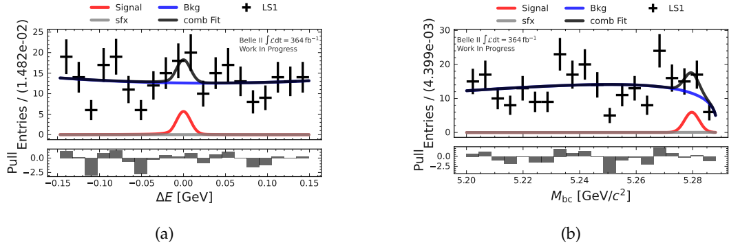
FIGURE I.49: M_{bc} and \Delta E fits in the q_1^2 -region for the B^0 \rightarrow K^{*0}(\rightarrow K^+ \pi^-) \mu\mu channel with the LS1 dataset.
