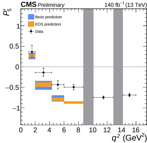
FIGURE 2.10: Most recent measurements of the P'_5 variable done by CMS [23]. This plot also shows the flavio [27] and EOS [28] SM prediction.
