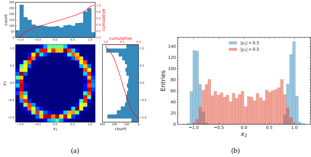
FIGURE 4.3: Distributions of correlations between two observables. (a) The linear correlation has been calculated to be r \approx 0.0 indicating that there is no correlation. However, a cut on y_2 results in a different distribution in x_2 . This can be seen in (b). Both variables are correlated.
