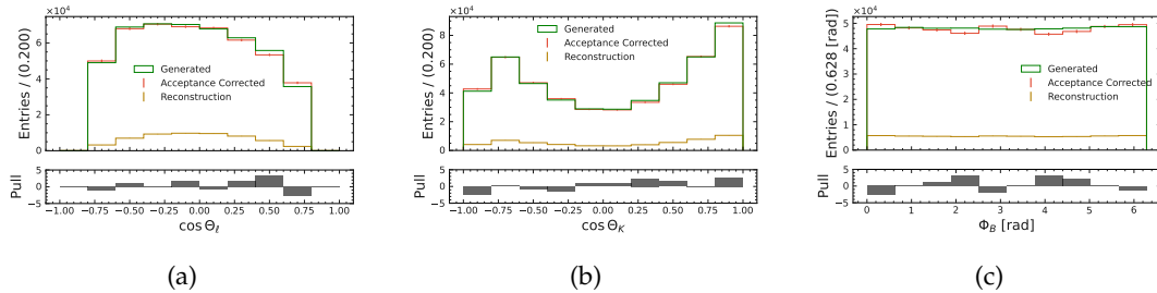
FIGURE G.69: Decay angle acceptance correction for \cos \theta_\ell (a), \cos \theta_K (b) and \phi_B (c) for the B^+ \rightarrow K^{*+}(\rightarrow K_S^0 \pi^+) \mu\mu channel in the q_1^2 -region. Green shows the distribution on generator level. The reconstructed candidates are shown in dark orange. They are corrected with the acceptance correction and the result is shown in red.
