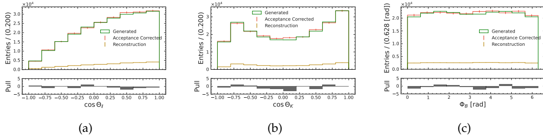
FIGURE G.67: Decay angle acceptance correction for \cos \theta_\ell (a), \cos \theta_K (b) and \phi_B (c) for the B^+ \rightarrow K^{*+}(\rightarrow K_S^0 \pi^+) ee channel in the q_{l/\psi}^2 -region. Green shows the distribution on generator level. The reconstructed candidates are shown in dark orange. They are corrected with the acceptance correction and the result is shown in red.
