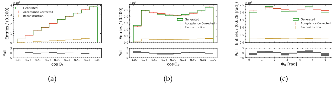
FIGURE G.68: Decay angle acceptance correction for \cos \theta_\ell (a), \cos \theta_K (b) and \phi_B (c) for the B^+ \rightarrow K^{*+}(\rightarrow K_S^0 \pi^+) ee channel in the q_{\psi(2S)}^2 -region. Green shows the distribution on generator level. The reconstructed candidates are shown in dark orange. They are corrected with the acceptance correction and the result is shown in red.
