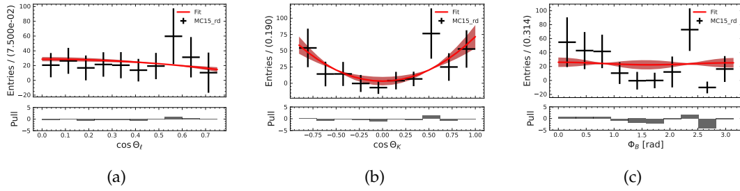
FIGURE I.41: Angular fit projections for the B^+ \rightarrow K^{*+}(\rightarrow K_S^0\pi^+)\ell\ell channel in the q_1^2 -region with the MC15_rd dataset.
