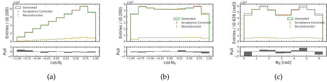
FIGURE G.72: Decay angle acceptance correction for \cos \theta_\ell (a), \cos \theta_K (b) and \phi_B (c) for the B^+ \rightarrow K^{*+}(\rightarrow K_S^0 \pi^+) \mu \mu channel in the q_4^2 -region. Green shows the distribution on generator level. The reconstructed candidates are shown in dark orange. They are corrected with the acceptance correction and the result is shown in red.
