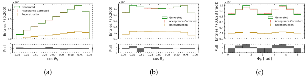
FIGURE G.60: Decay angle acceptance correction for \cos \theta_\ell (a), \cos \theta_K (b) and \Phi_B (c) for the B^0 \rightarrow K^{*0}(\rightarrow K^+ \pi^-) \mu \mu channel in the q_4^2 -region. Green shows the distribution on generator level. The reconstructed candidates are shown in dark orange. They are corrected with the acceptance correction and the result is shown in red.
