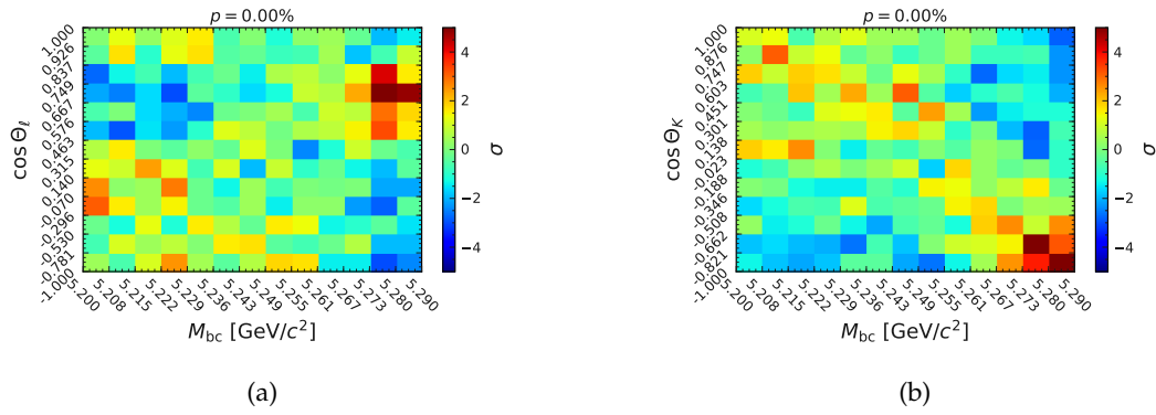
FIGURE 7.19: Correlation between M_{bc} and \cos \theta_\ell and \cos \theta_K in the B^+ \rightarrow K^{*+}(\rightarrow K^+ \pi^0) \mu \mu channel for background events. A rather strong correlation can be observed between M_{bc} and \cos \theta_\ell . In the case of this \mu -channels, there also appears to be a correlation between M_{bc} and \cos \theta_\ell . Due to these correlations, this channel can no longer be analyzed with the sWeights method.
