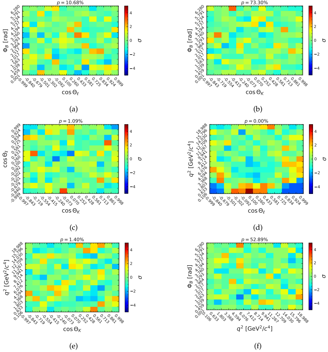
FIGURE G.2: Correlations Between the Four Decay Variables for the B^+ \rightarrow K^{*+}(\rightarrow K_S^0 \pi^+) ee . There is a correlation between \cos \theta_\ell and q^2 . However, this correlation is expected since both of these variables depend on both leptons in the decay.
