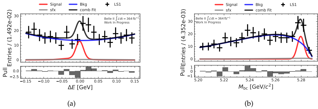
FIGURE I.56: M_{bc} and \Delta E fits in the q_4^2 -region for the B^0 \rightarrow K^{*0}(\rightarrow K^+\pi^-)\ell\ell channel with the LS1 dataset.
