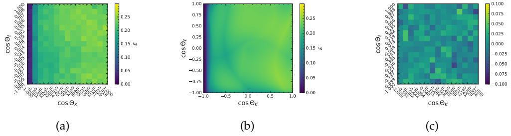
FIGURE G.36: (a) Input efficiencies for the acceptance model training. Resulting acceptance correction model for the decay B^0 \rightarrow K^{*0}(\rightarrow K^+\pi^-)\mu\mu in the q_3^2 region. In (b) the resulting model function is shown. In (c) the difference between the predicted and true efficiency is shown.
