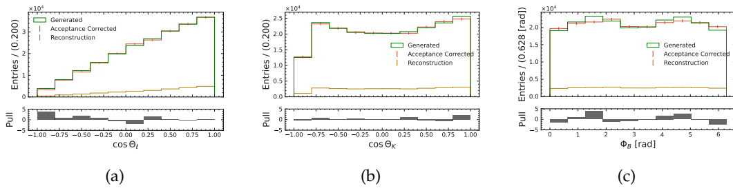
FIGURE G.74: Decay angle acceptance correction for \cos \theta_\ell (a), \cos \theta_K (b) and \phi_B (c) for the B^+ \rightarrow K^{*+}(\rightarrow K_S^0 \pi^+) \mu \mu channel in the q_J^2/\psi(2S)^- region. Green shows the distribution on generator level. The reconstructed candidates are shown in dark orange. They are corrected with the acceptance correction and the result is shown in red.
