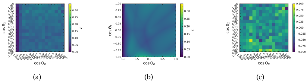
FIGURE G.51: (a) Input efficiencies for the acceptance model training. Resulting acceptance correction model for the decay B^+ \rightarrow K^{*+}(\rightarrow K_S^0 \pi^+) \mu \mu in the q_{\psi(2S)}^2 region. In (b) the resulting model function is shown. In (c) the difference between the predicted and true efficiency is shown.
