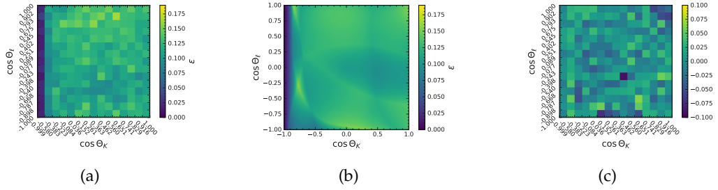
FIGURE G.42: (a) Input efficiencies for the acceptance model training. Resulting acceptance correction model for the decay B^+ \rightarrow K^{*+}(\rightarrow K_S^0 \pi^+) ee in the q_3^2 region. In (b) the resulting model function is shown. In (c) the difference between the predicted and true efficiency is shown.
