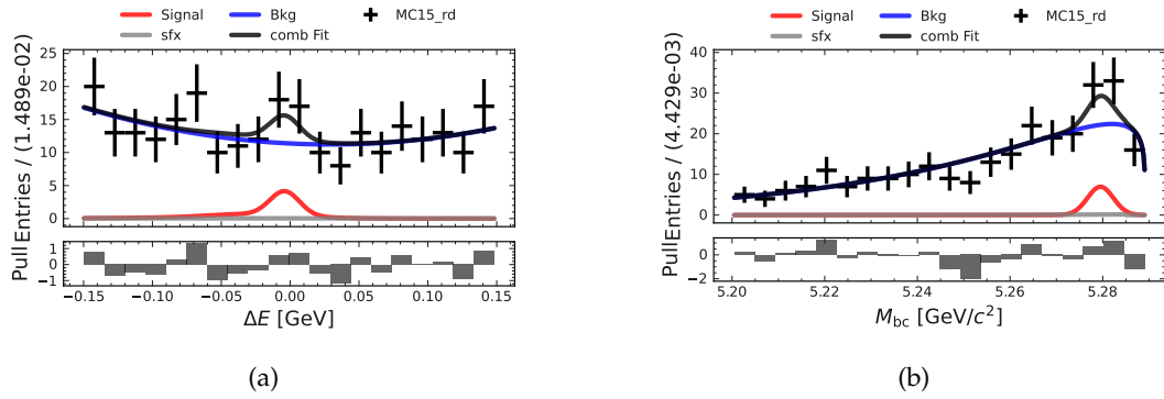
FIGURE I.2: M_{bc} and \Delta E fits in the q_3^2 -region for the B^0 \rightarrow K^{*0}(\rightarrow K^+\pi^-)ee channel with the MC15_rd dataset.
