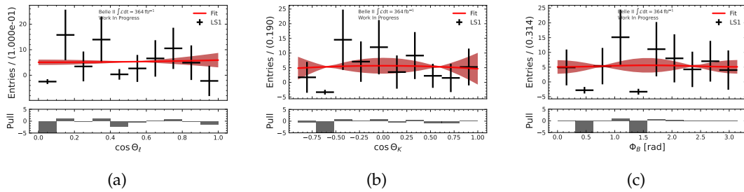
FIGURE I.67: Angular fit projections for the B^0 \rightarrow K^{*0}(\rightarrow K^+\pi^-)\ell\ell channel in the q_3^2 -region with the LS1 dataset.
