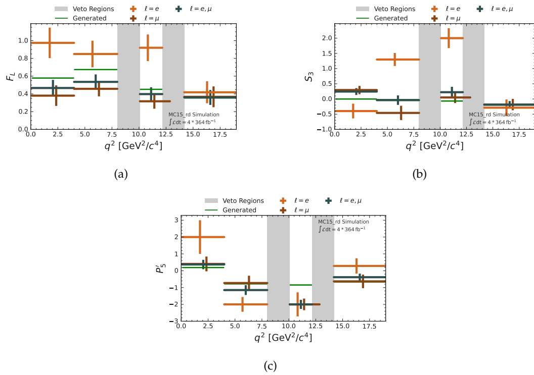
FIGURE 9.5: Angular parameters obtained by the three dimensional fit as a function of q^2 for the B^0 \rightarrow K^{*0}(\rightarrow K^+ \pi^-) \ell \ell channels in the MC15_rd dataset without the s Weights method. Instead the background shape is fixed. (a) shows F_L , (b) S_3 and (c) P'_5 .
