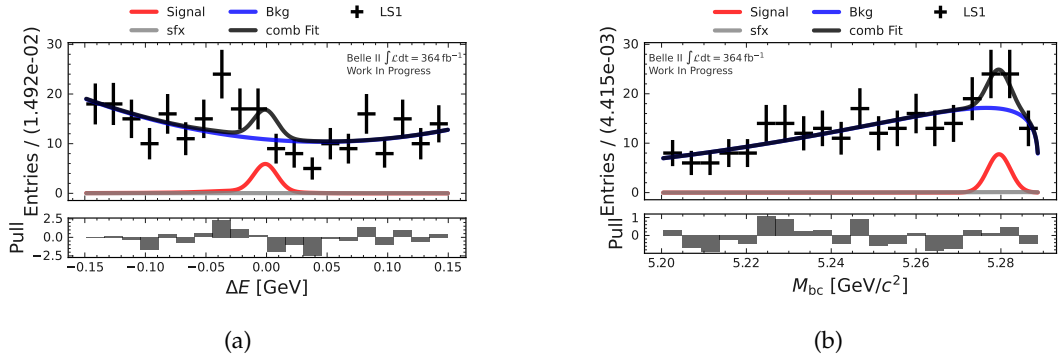
FIGURE I.55: M_{bc} and \Delta E fits in the q_3^2 -region for the B^0 \rightarrow K^{*0}(\rightarrow K^+\pi^-)\ell\ell channel with the LS1 dataset.
