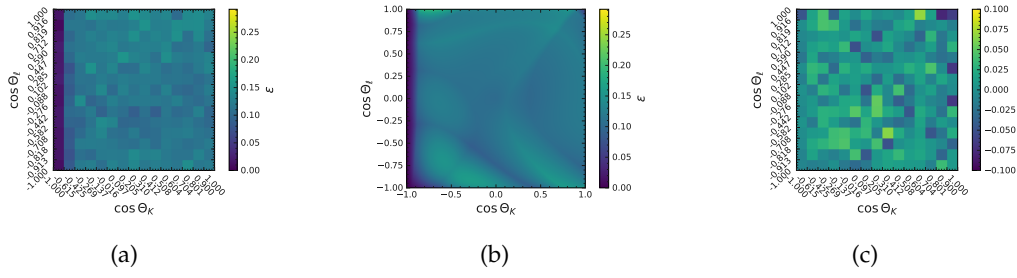
FIGURE G.44: (a) Input efficiencies for the acceptance model training. Resulting acceptance correction model for the decay B^+ \rightarrow K^{*+}(\rightarrow K_S^0 \pi^+) ee in the q_{l/\psi}^2 region. In (b) the resulting model function is shown. In (c) the difference between the predicted and true efficiency is shown.
