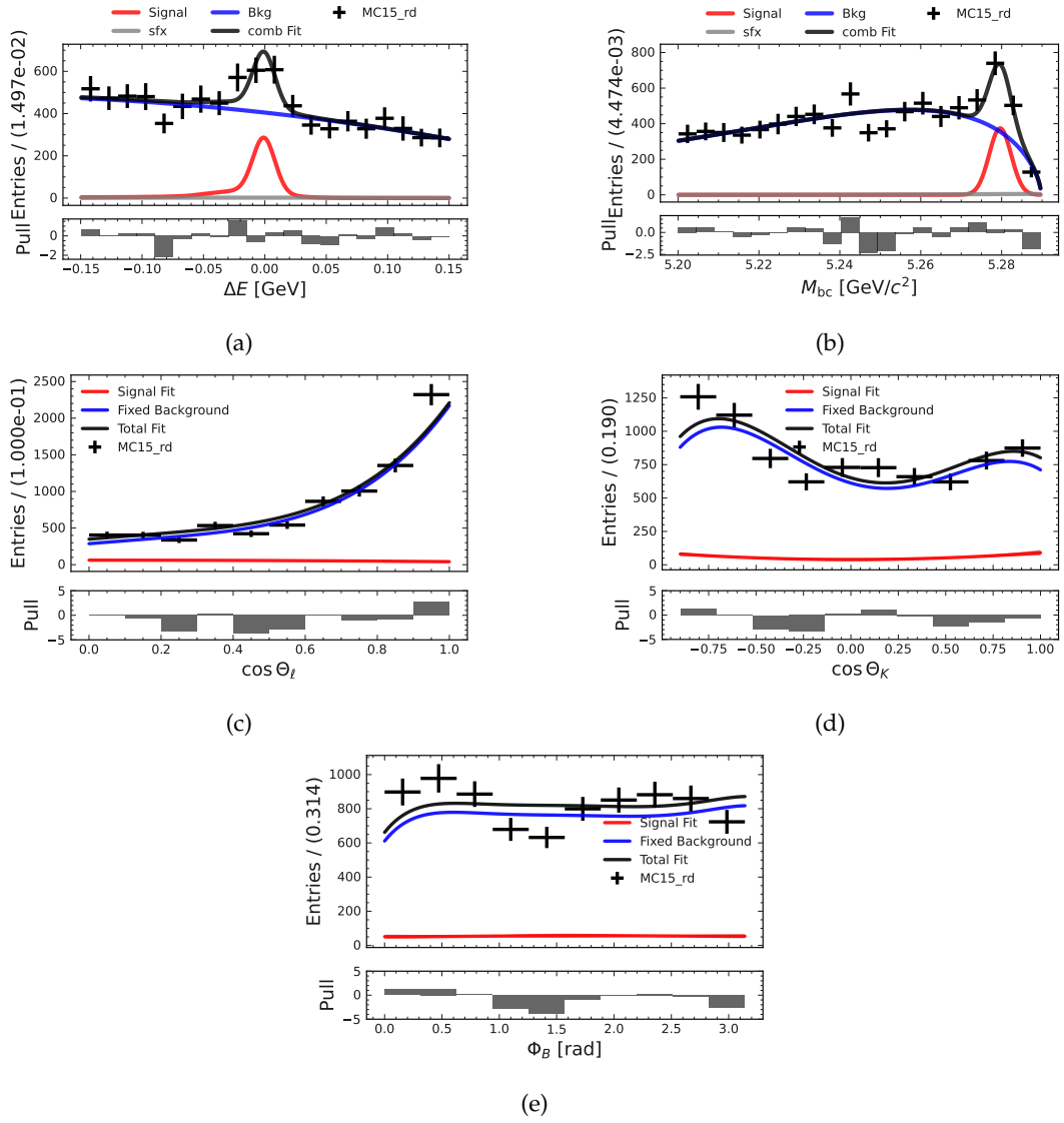
FIGURE J.12: Figures related to the fit study with fixed background shapes and no sWeights for the B^0 \rightarrow K^{*0}(\rightarrow K^+\pi^-)\ell\ell in the q_2^2 -region.
