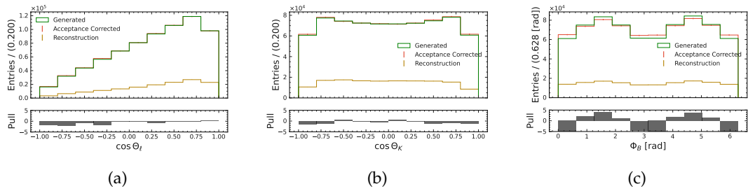
FIGURE G.54: Decay angle acceptance correction for \cos \theta_\ell (a), \cos \theta_K (b) and \Phi_B (c) for the B^0 \rightarrow K^{*0}(\rightarrow K^+\pi^-)ee channel in the q_4^2 -region. Green shows the distribution on generator level. The reconstructed candidates are shown in dark orange. They are corrected with the acceptance correction and the result is shown in red.
