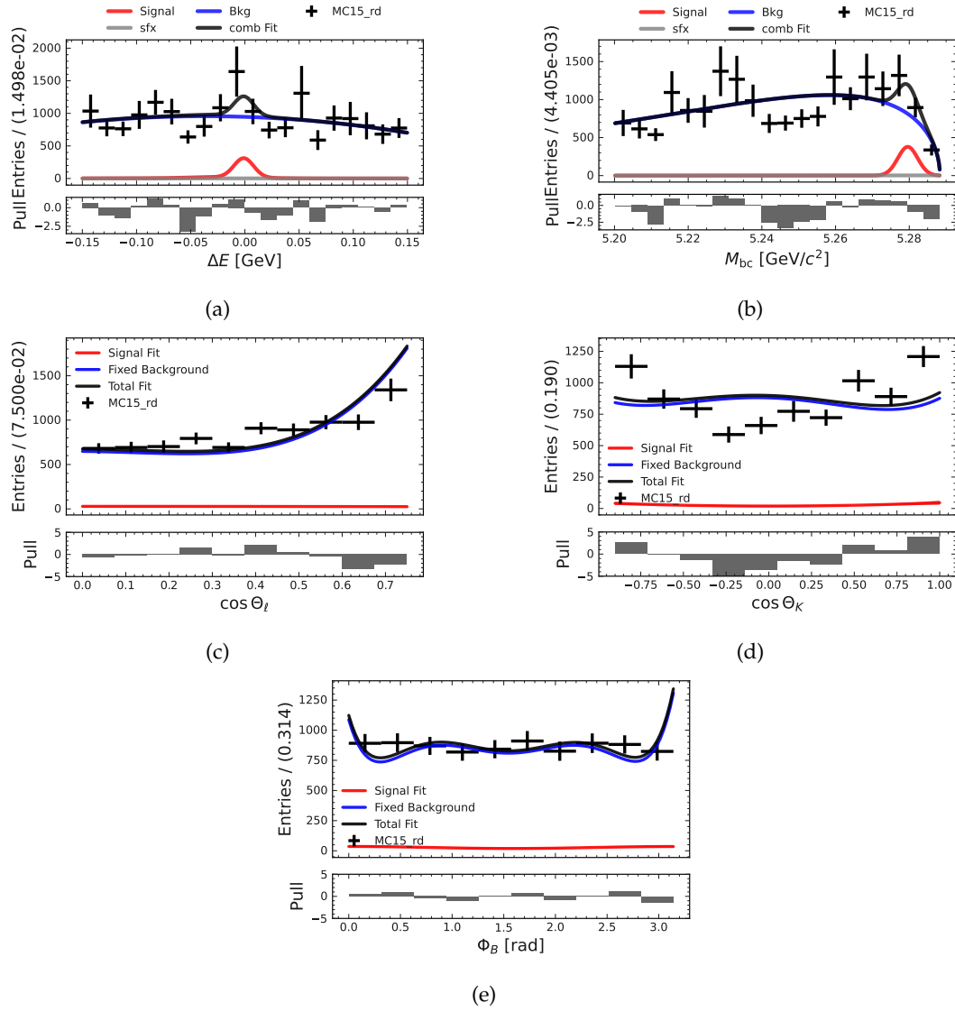
FIGURE J.11: Figures related to the fit study with fixed background shapes and no sWeights for the B^0 \rightarrow K^{*0}(\rightarrow K^+\pi^-)\ell\ell in the q_1^2 -region.
