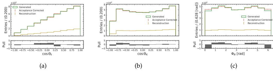
FIGURE G.56: Decay angle acceptance correction for \cos \theta_\ell (a), \cos \theta_K (b) and \phi_B (c) for the B^0 \rightarrow K^{*0}(\rightarrow K^+\pi^-)ee channel in the q_{\psi(2S)}^2 -region. Green shows the distribution on generator level. The reconstructed candidates are shown in dark orange. They are corrected with the acceptance correction and the result is shown in red.
