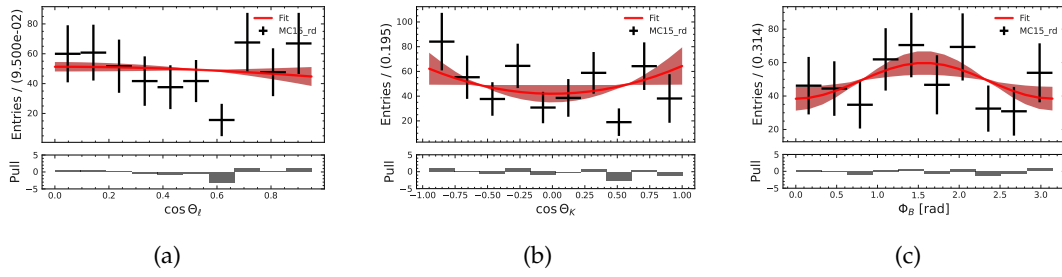
FIGURE I.40: Angular fit projections for the B^0 \rightarrow K^{*0}(\rightarrow K^+\pi^-)\ell\ell channel in the q_4^2 -region with the MC15_rd dataset.
