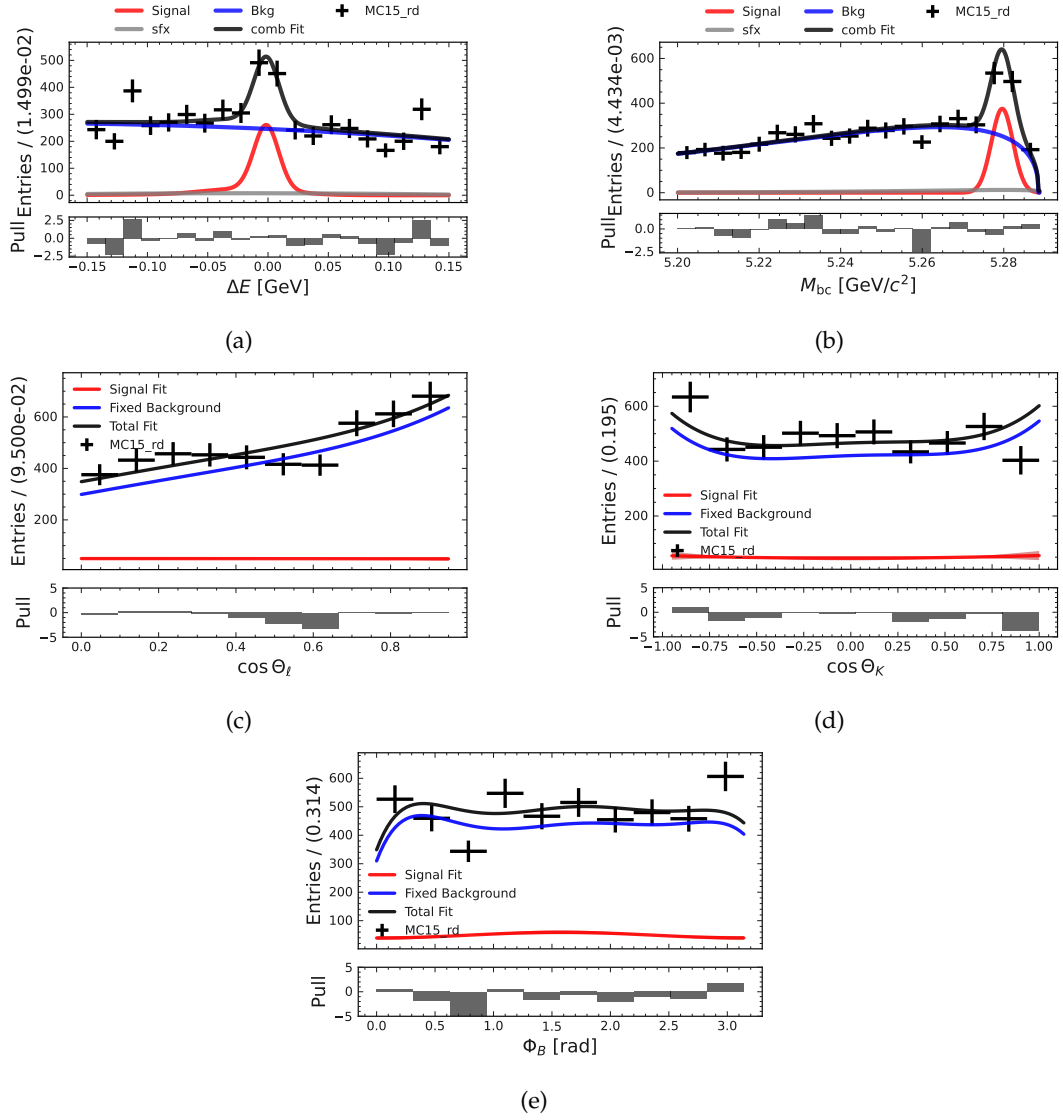
FIGURE J.14: Figures related to the fit study with fixed background shapes and no sWeights for the B^0 \rightarrow K^{*0}(\rightarrow K^+\pi^-)\ell\ell in the q_4^2 -region.
