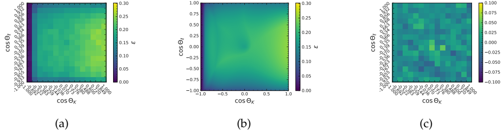
FIGURE G.35: (a) Input efficiencies for the acceptance model training. Resulting acceptance correction model for the decay B^0 \rightarrow K^{*0}(\rightarrow K^+\pi^-)\mu\mu in the q_2^2 region. In (b) the resulting model function is shown. In (c) the difference between the predicted and true efficiency is shown.
