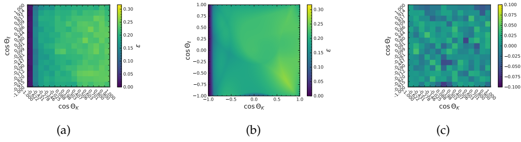
FIGURE G.38: (a) Input efficiencies for the acceptance model training. Resulting acceptance correction model for the decay B^0 \rightarrow K^{*0}(\rightarrow K^+ \pi^-) \mu \mu in the q_{l/\psi}^2 region. In (b) the resulting model function is shown. In (c) the difference between the predicted and true efficiency is shown.
