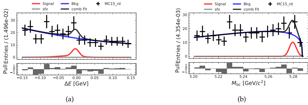
FIGURE I.1: M_{bc} and \Delta E fits in the q_1^2 -region for the B^0 \rightarrow K^{*0}(\rightarrow K^+\pi^-)ee channel with the MC15_rd dataset.
