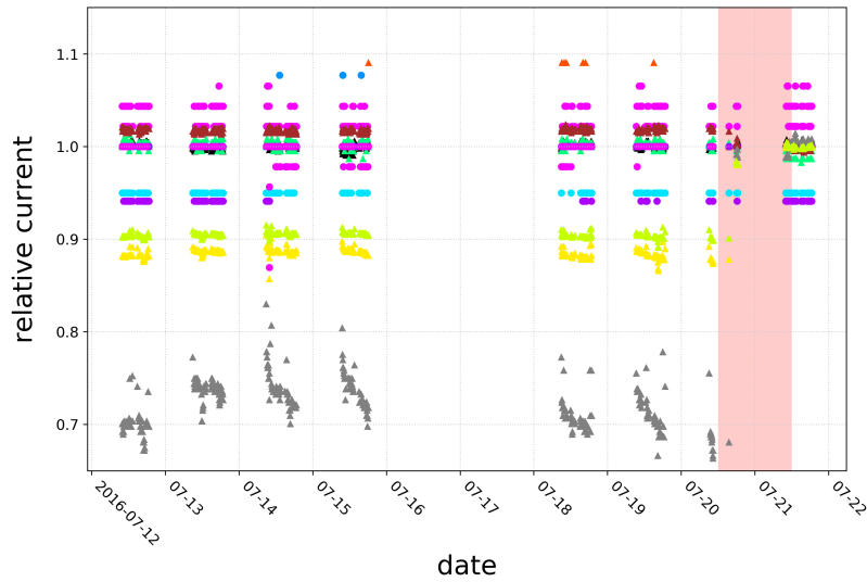
Figure A.8.: Development of relative currents during the EMC measurement campaign. For each power supply line the current is shown relative to the corresponding current in the last measurement. Lines with very small currents are not plotted as their value in the last measurement was either 0 mA or the low measurement accuracy would lead to delusive values for the plotted deviation.
