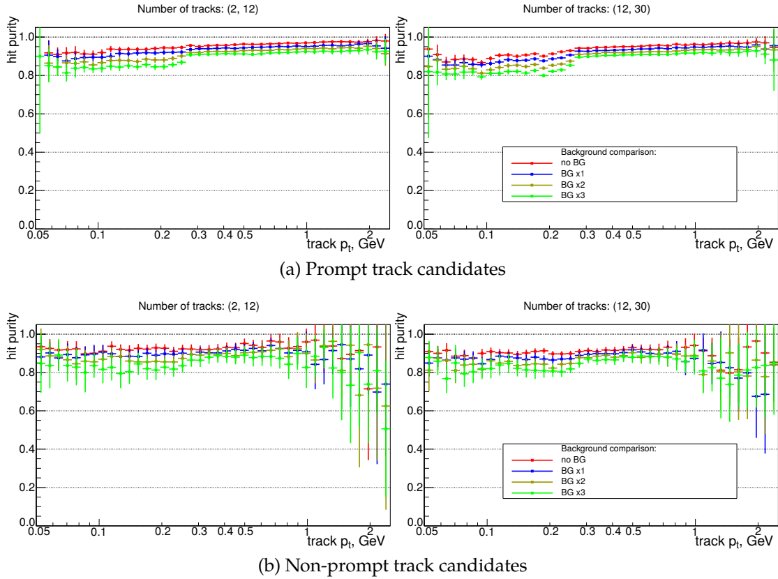
Figure 7.17.: Comparison of the track hit purities of the Belle II track finding chain with different beam background levels for prompt (a) and non-prompt (b) track candidates samples based on the number of generated tracks in event (event multiplicity) in bins of track's p_t
