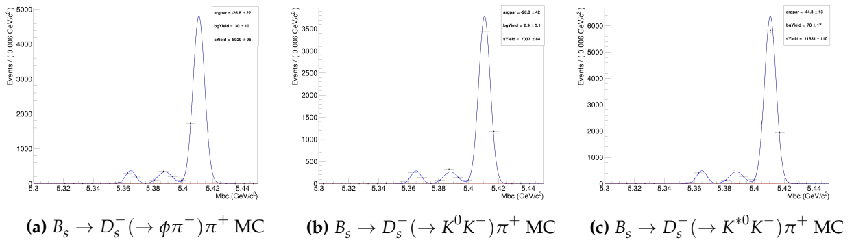
Figure 4.52.: M_{bc} fits with nn_{out} \geq 0.95
