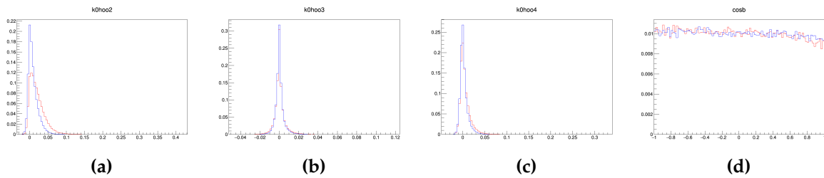
Figure 4.19.: Variables used for NeuroBayes training from MC. The red curve are background ( q\bar{q} continuum). The blue curve is signal MC.
