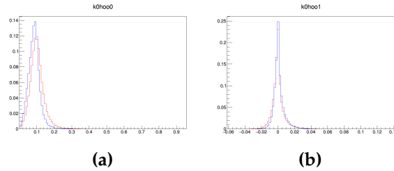
Figure 4.18.: Variables used for NeuroBayes training from MC. The red curve are background ( q\bar{q} continuum). The blue curve is signal MC.
