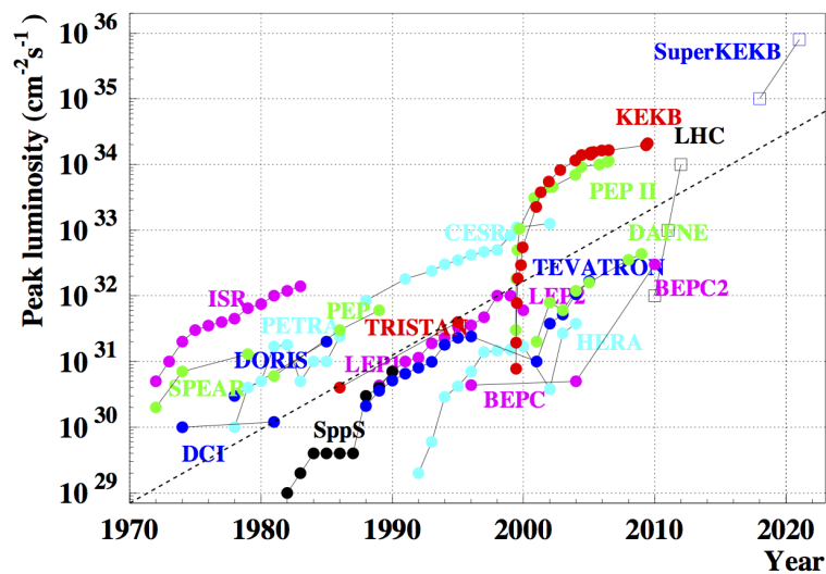
Figure 2.1.: Accelerator luminosities
