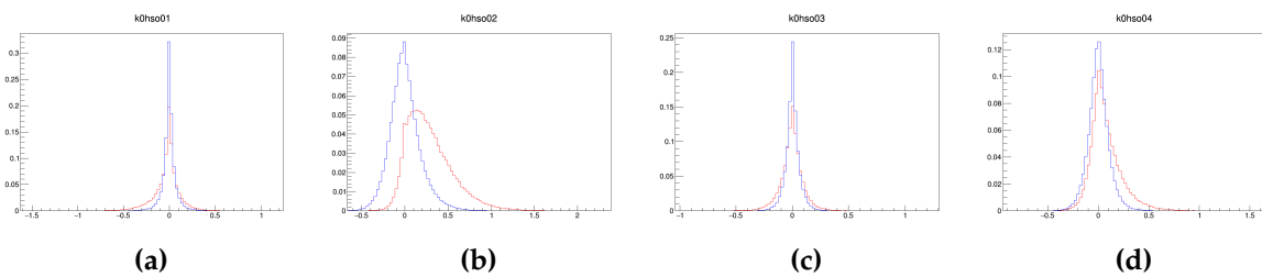
Figure 4.15.: Variables used for NeuroBayes training from MC. The red curve are background ( q\bar{q} continuum). The blue curve is signal MC.
