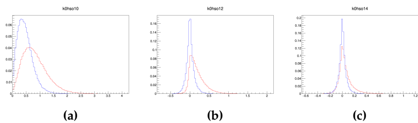
Figure 4.16.: Variables used for NeuroBayes training from MC. The red curve are background ( q\bar{q} continuum). The blue curve is signal MC.
