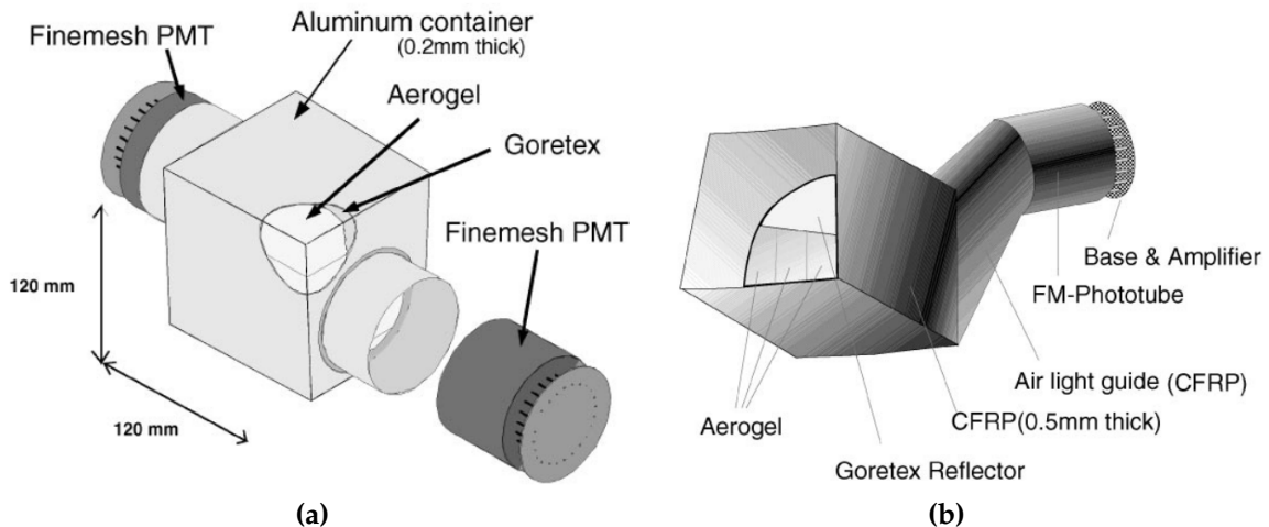
Figure 1.9.: PMTs for the ACC; Barrel ACC (left), Endcap ACC (right)
