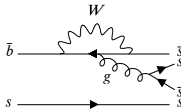
Figure 3.3.: Feynman diagram for a penguin process
