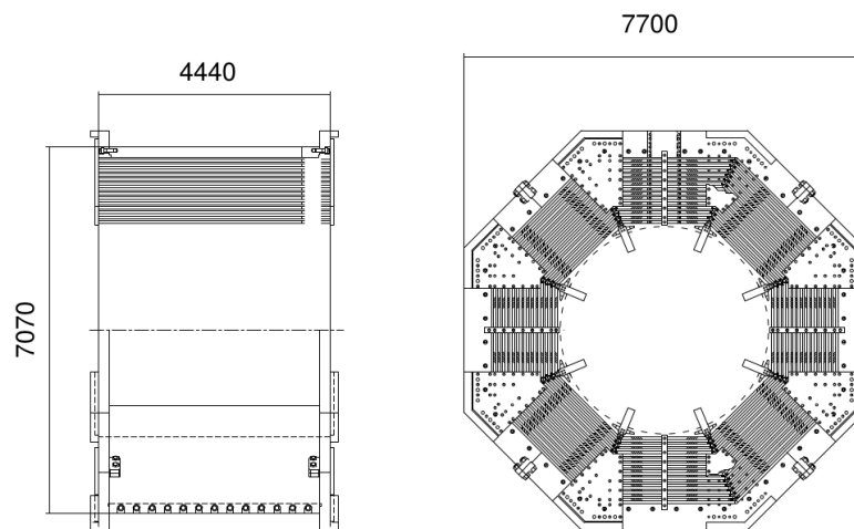
Figure 1.20.: View of the Belle barrel iron yoke structure
