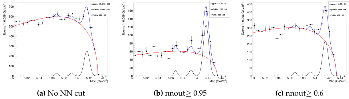
Figure 4.55.: B_s^0 \rightarrow D_s^- \rho^+ - Results from fitting to the full 121.4 \text{ fb}^{-1} integrated luminosity \Upsilon(5S) data sample
