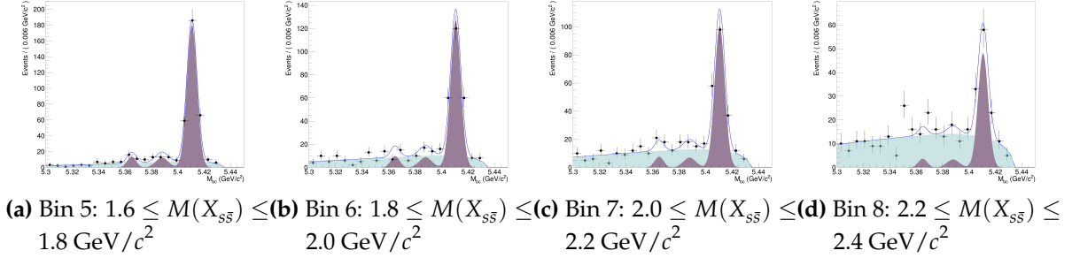
Figure 4.29.: M_{bc} distributions in individual X_{S\bar{S}} mass bins; B_s^0 \rightarrow K^\pm K_S^0 + n\pi modes. The dark shaded curve is the signal Gaussian portion of the fit, the light shaded curve is the ARGUS portion of the fit, and the blue curve is the sum of the two.
