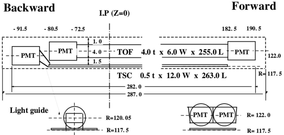
Figure 1.10.: Diagram of the TOF system
