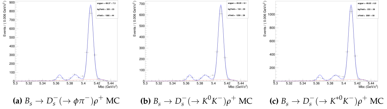
Figure 4.50.: M_{bc} fits with nn_{out} \geq 0.95
