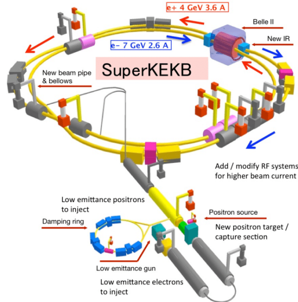
Figure 2.1: The SuperKEKB Collider [4]
