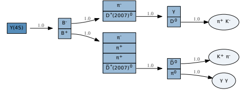
(f) Mode 5: B_{\text{sig}}: B^+, H_c: D^{*0}
