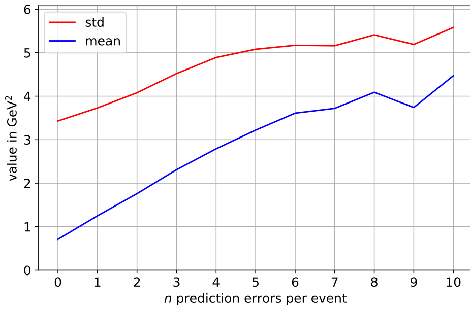
Figure 6.6: n -prediction errors dependance of std and mean in m_{\text{miss}}^2 distribution in figure 6.5 ( n \in \mathbb{N}, 0 \leq n \leq 10 ).
