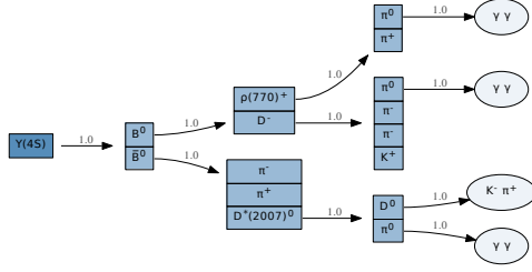
(a) Mode 0: B_{\text{sig}}: \bar{B}^0, H_c: D^-
