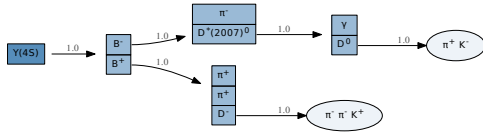
(c) Mode 2: B_{\text{sig}}: B^-, H_c: D^-
