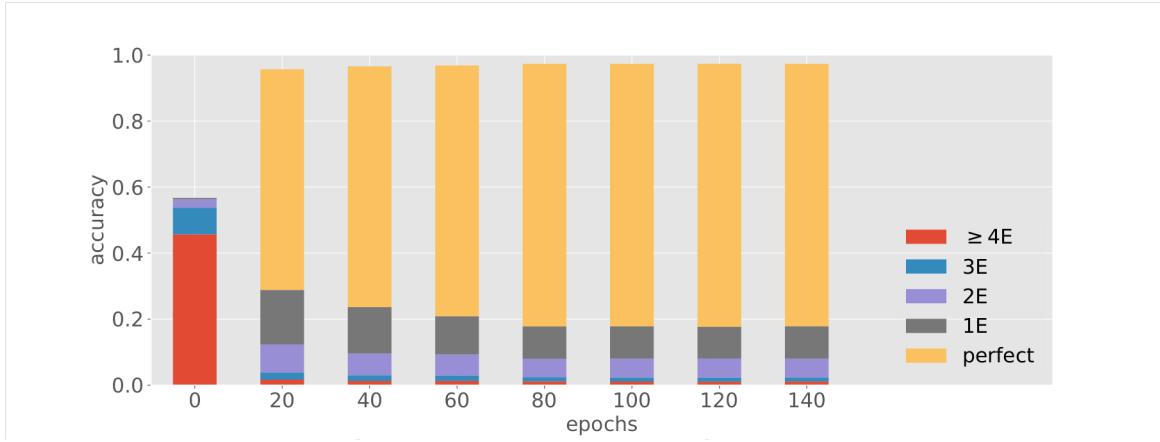
Figure 5.4: Fraction of number of prediction errors per event, normalized to the overall accuracy for X - H_c - B_{\text{sig}} - background training over training epochs on validation data set.
