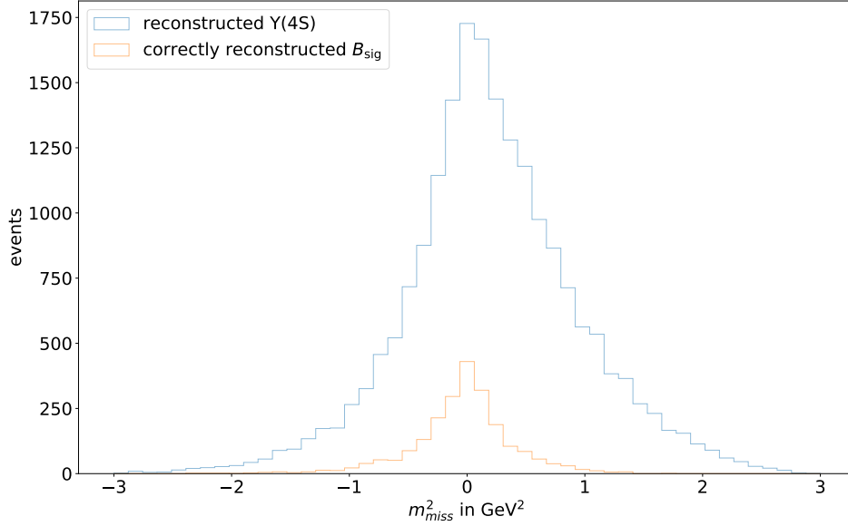
Figure 6.1: m_{\text{miss}}^2 , as defined in equation (2.2), distribution for the existing semi-inclusive tagging method. In blue all events which passed all the applied selections are shown and in orange all events which additionally have a correctly reconstructed B_{\text{sig}} .
