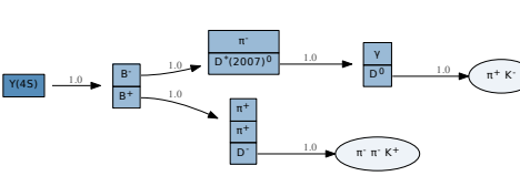
(f) Mode 5: B_{\text{sig}}: B^+, H_c: D^{*0}
