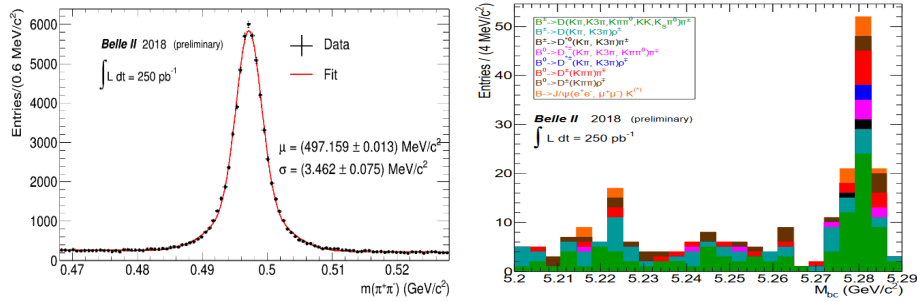
Fig. 3. Invariant mass of reconstructed $K_S^0 \to \pi^+\pi^-$ (left) and beam constrained mass $M_{bc}$ for reconstructed $B$ meson from different modes.
