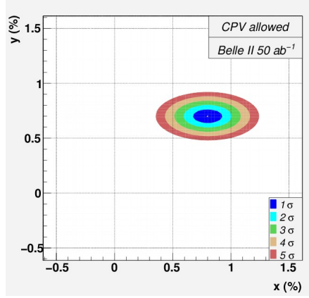
Fig. 2 Expected Belle II precision at 50 \text{ ab}^{-1} data.
