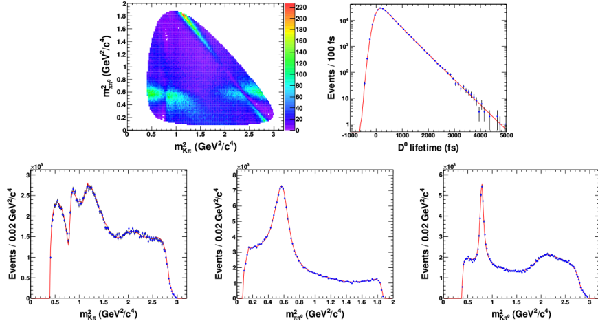
Fig. 1 The top row shows the time-dependent Dalitz plot fit and the decay time fit to the lifetime-smearred sample of wrong-sign D^0 \rightarrow K^-\pi^+\pi^0 decays. The bottom row shows projections of the fitted Dalitz variables.
