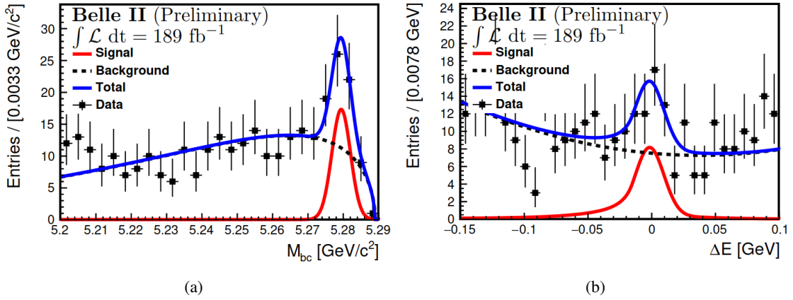
Figure 3: Fit to the (a) M_{bc} and (b) \Delta E distributions of B \rightarrow K^* l^+ l^- events.
